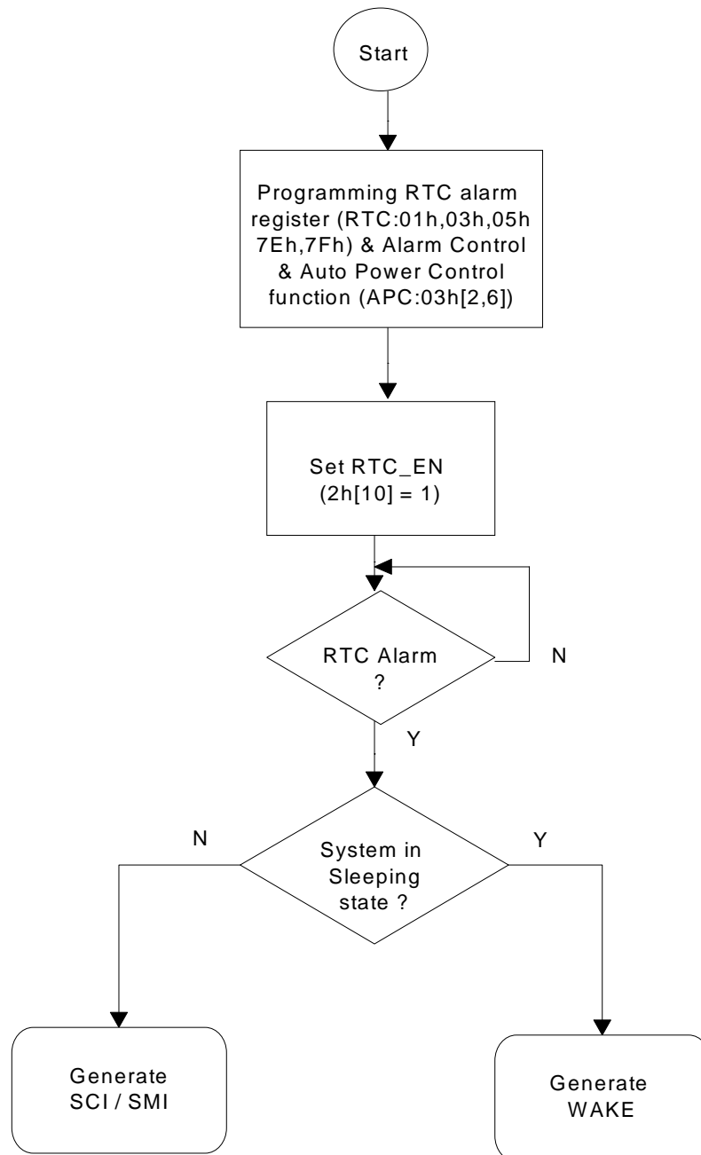
Figure 3-21 RTC Alarm Flow Chart
