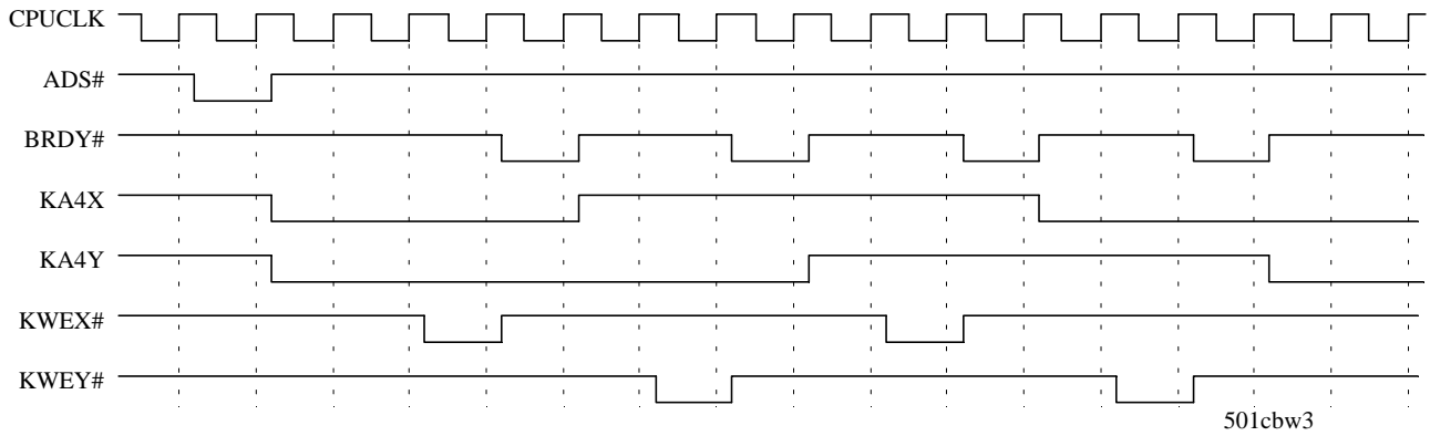
Cache Burst Write Hit Cycle 5-3-3-3
