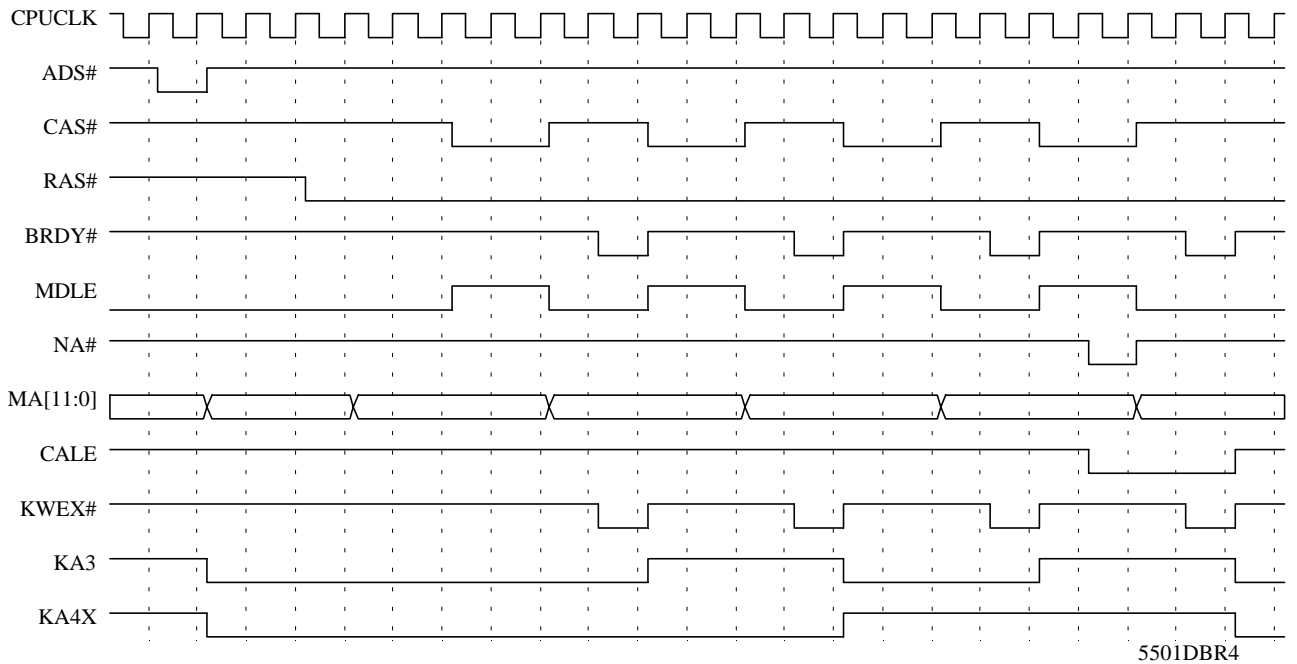
DRAM Burst Read - Row Miss 10-4-4-4 (Cache 3/4-x-x-x)
