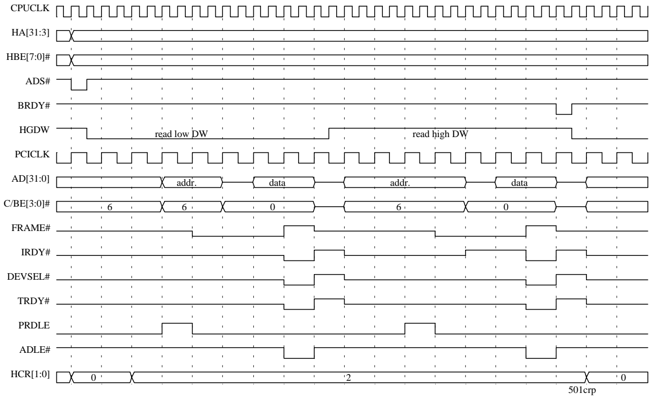
CPU Read PCI Slave
