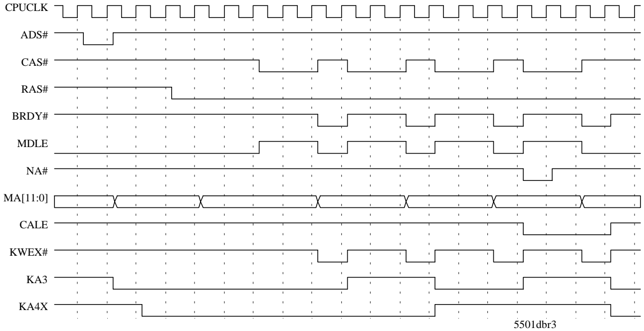
DRAM Burst Read - Row Miss 9-3-3-3 (Cache 3/4-x-x-x)
