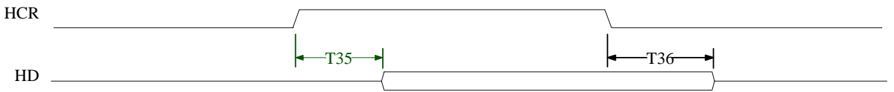
Figure 3.13 CPU Read DRAM or PCI Cycle
