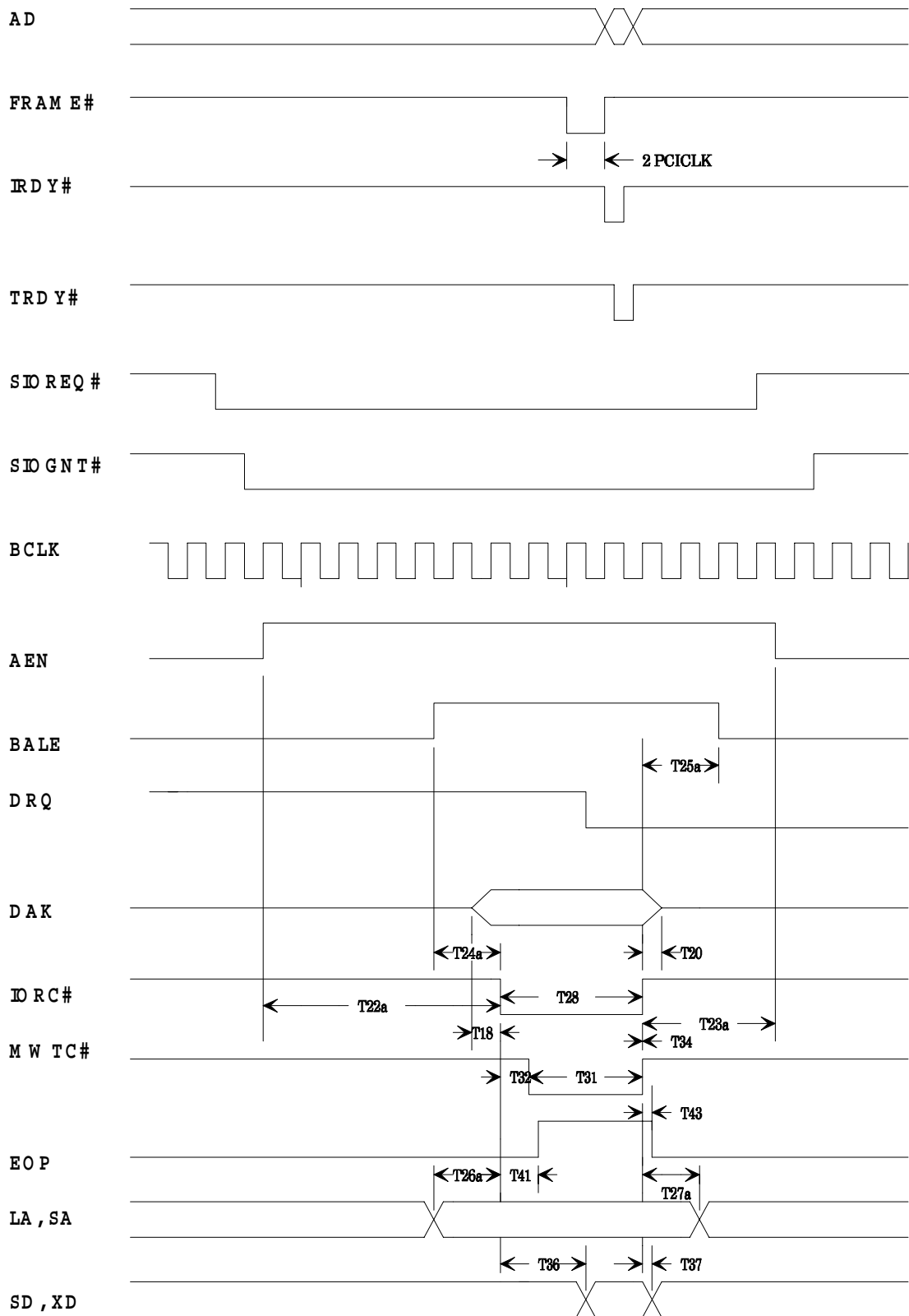
DMA cycle (IOWC#, MRDC#), DMACLK = BCLK
