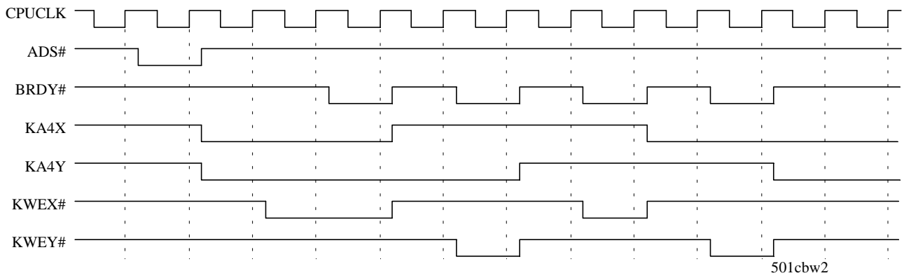
Cache Burst Write Hit Cycle 4-2-2-2
