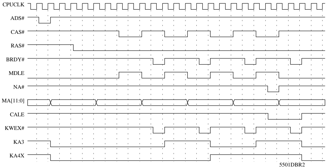
DRAM Burst Read - Row Miss 11-4-4-4 (Cache 3/4-x-x-x)
