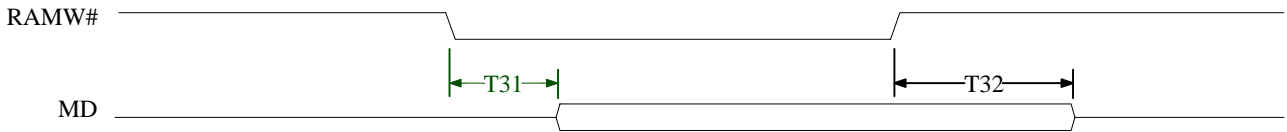
Figure 3.11 CPU Write DRAM Cycle
