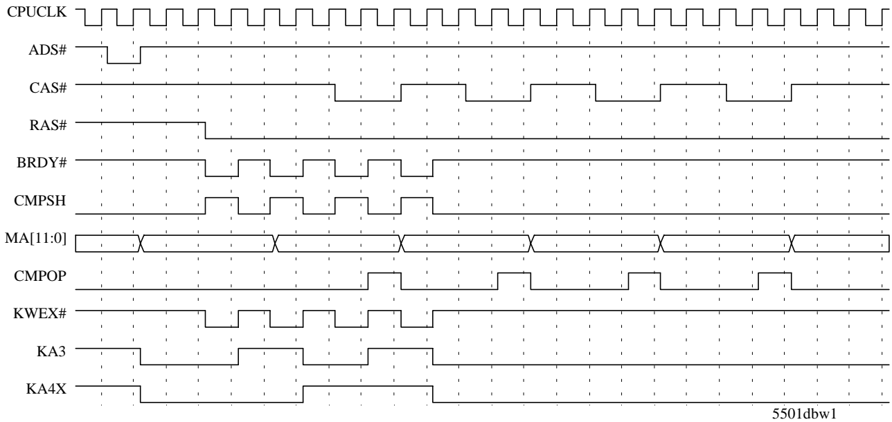
EDO Burst Read (7-2-2-2)
