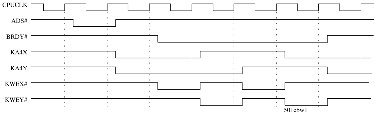
Cache Burst Write Hit Cycle 3-1-1-1
