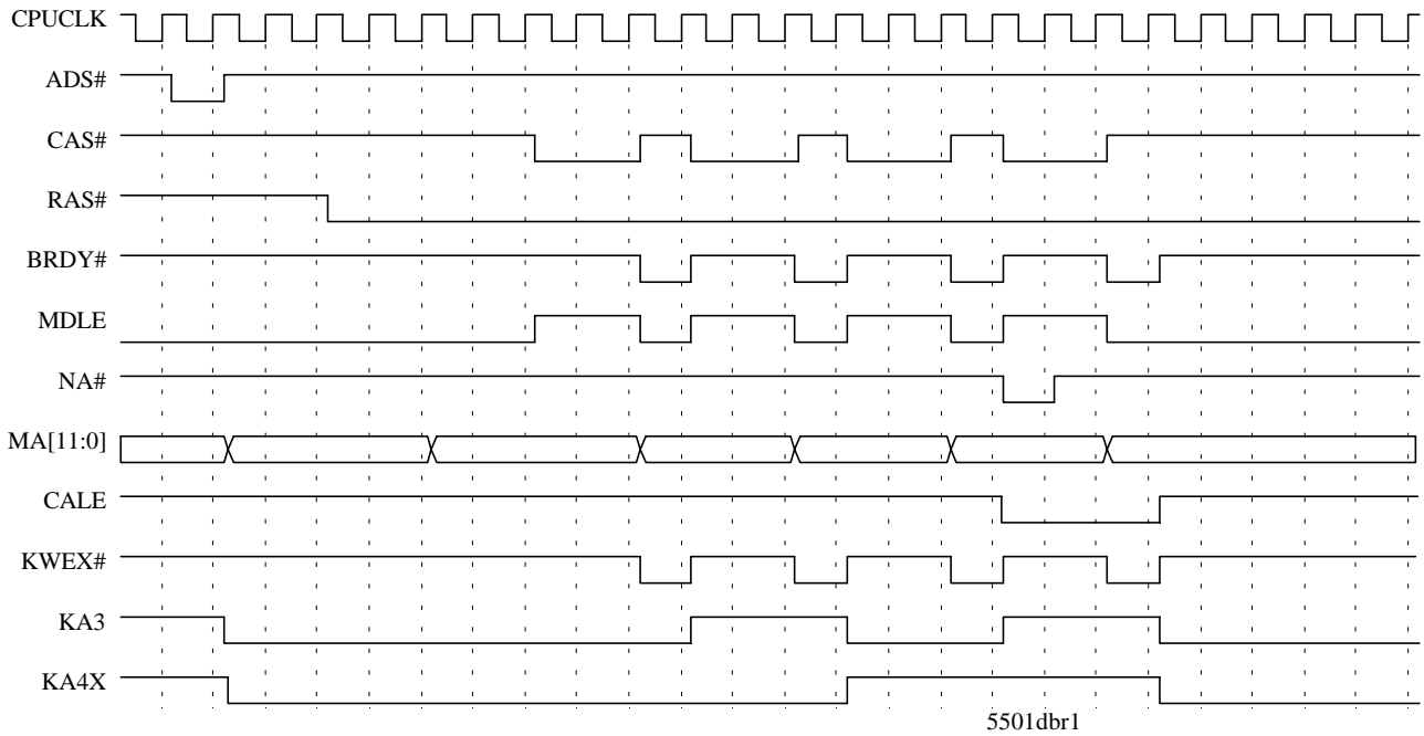
DRAM Burst Read - Row Miss 10-3-3-3 (Cache 3/4-x-x-x)
