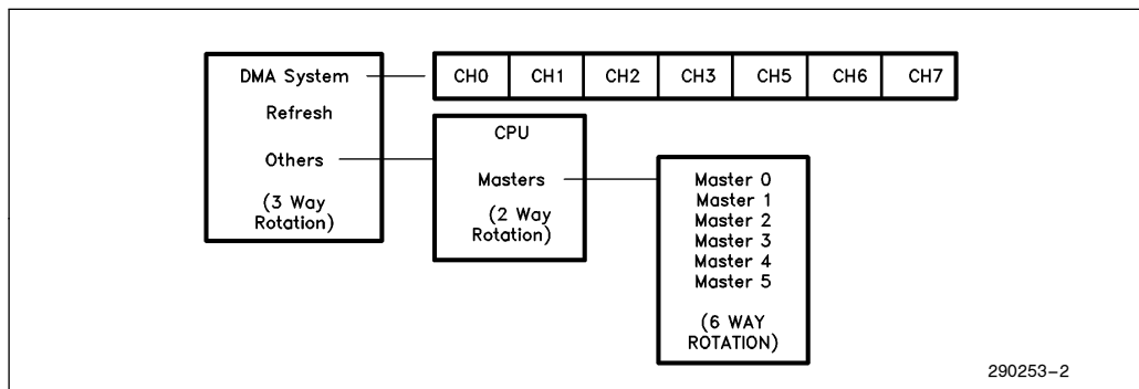
Figure 2-1. Arbitration Priority
