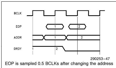
Figure 8-6. Burst Mode EOP Timing
