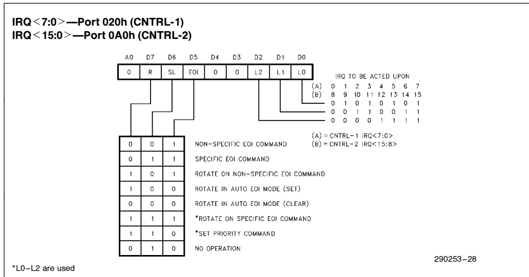
Figure 5-9. OCW2
