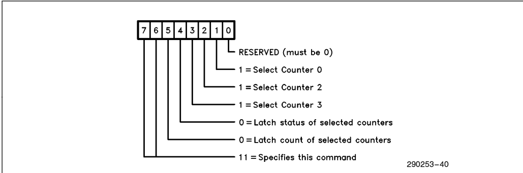
Figure 7-3. Current Read-Back Command Format
