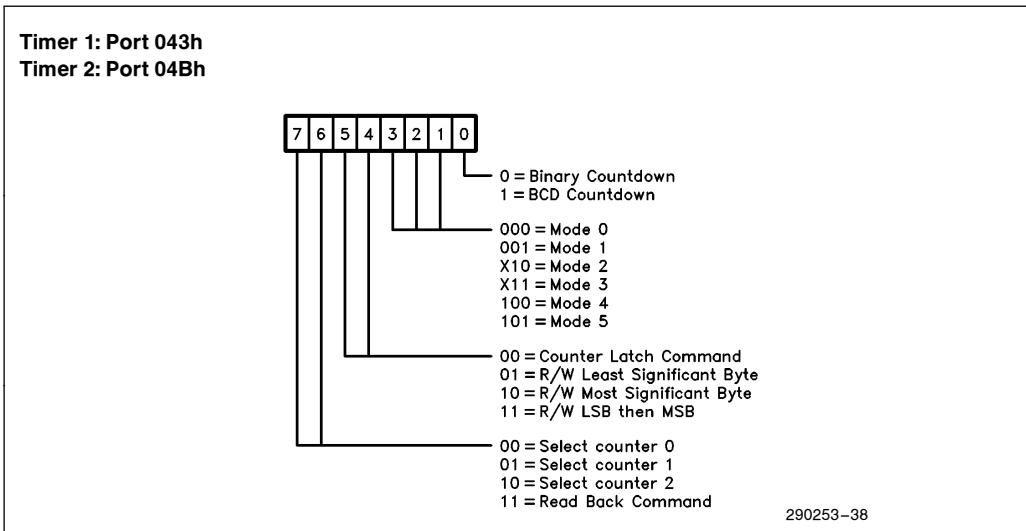
Figure 7-1. Control Word
