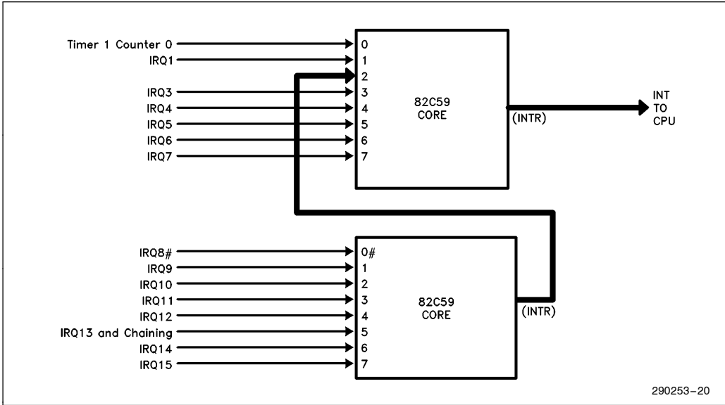
Figure 5-1. Interrupt Controller
