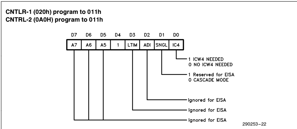
Figure 5-3. ICW1
