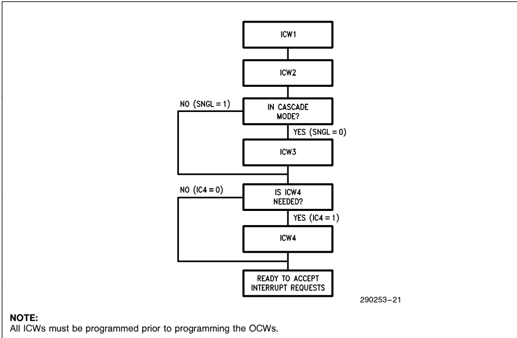
Figure 5-2. Initialization Sequence
