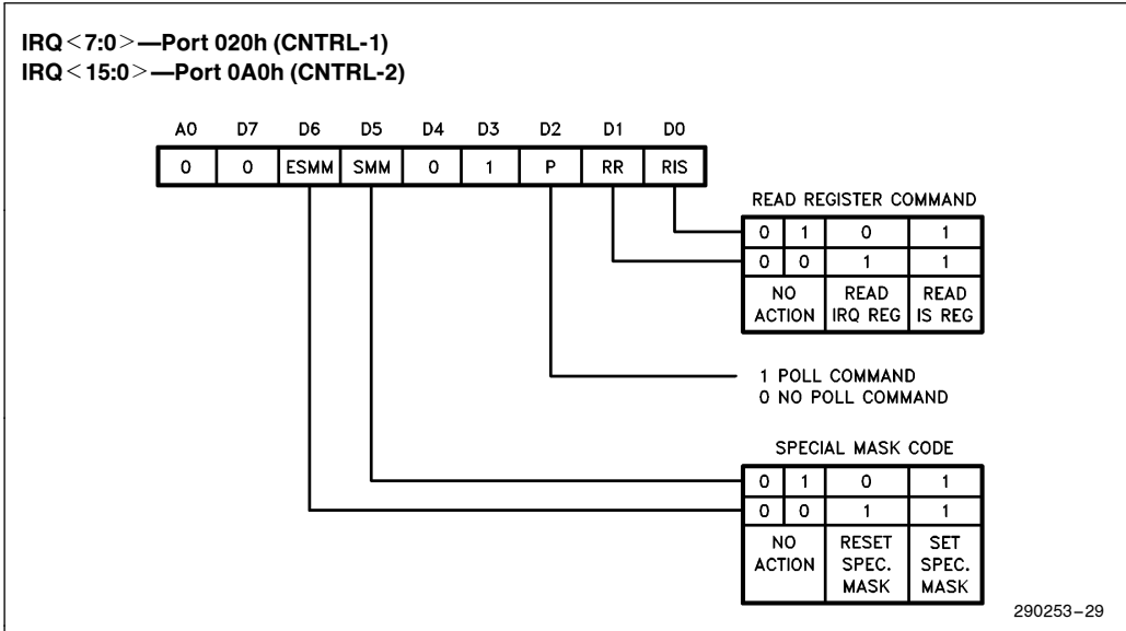
Figure 5-10. OCW3
