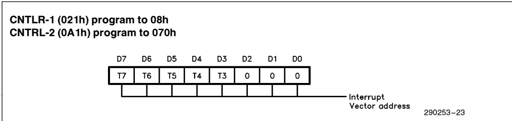
Figure 5-4. ICW2
