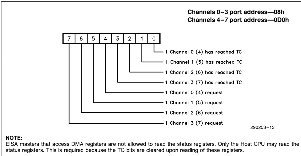
Figure 3-10. Status Register (Read Only)
