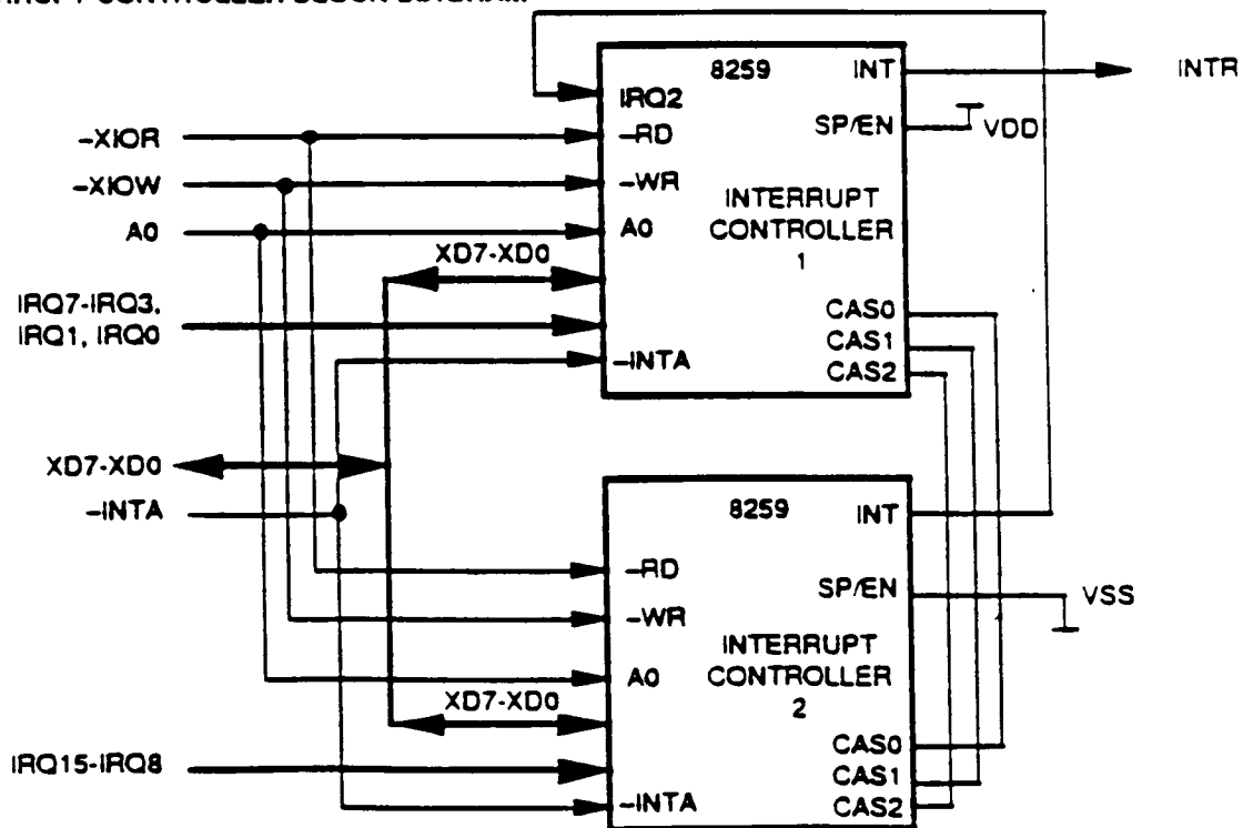
FIGURE 2. INTERRUPT CONTROLLER BLOCK DIAGRAM
