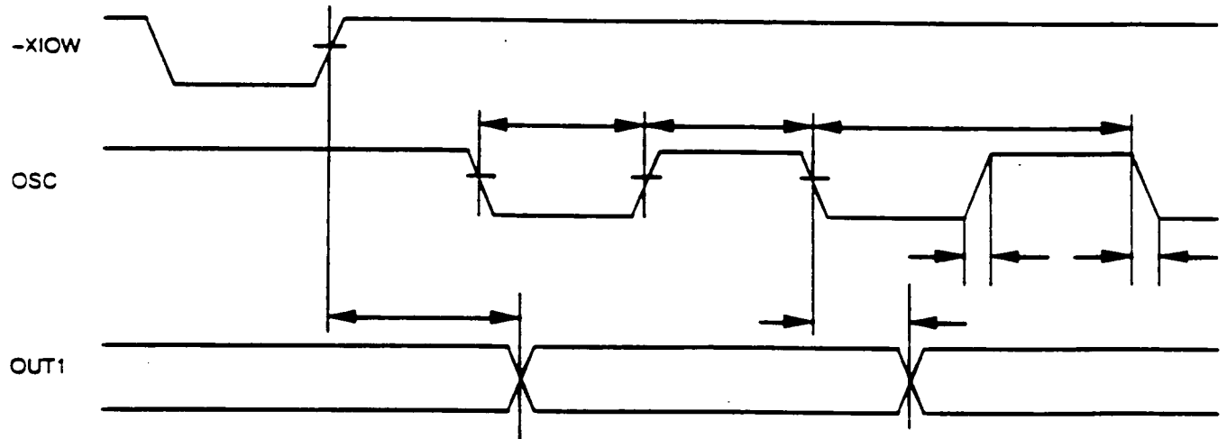
FIGURE 10. TIMER/COUNTER TIMING
