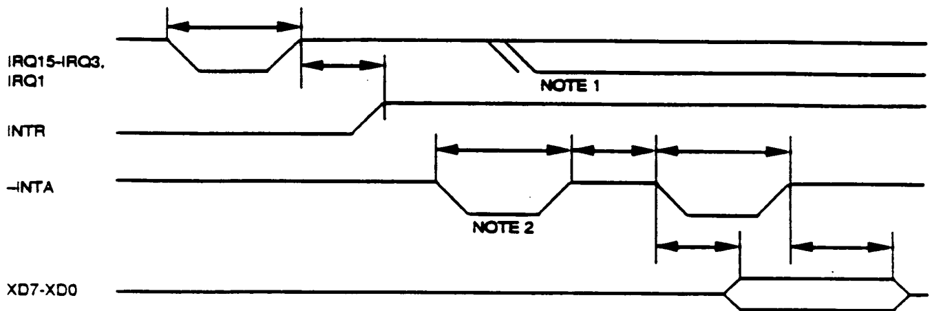
FIGURE 7. INTERRUPT TIMING
