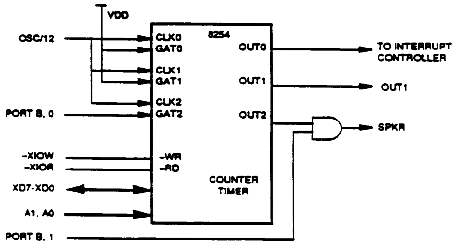
FIGURE 3. COUNTER/TIMER BLOCK DIAGRAM
