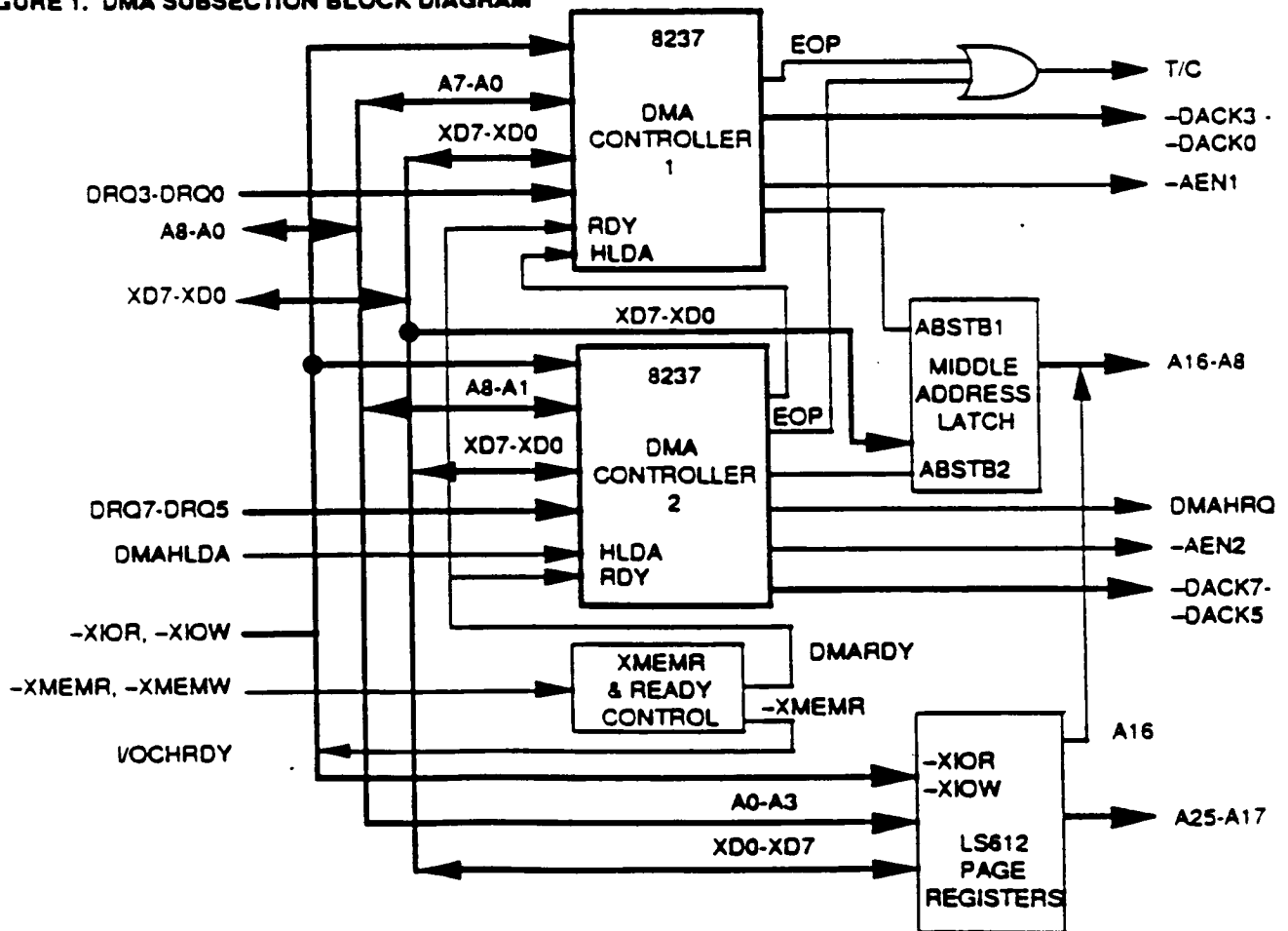
FIGURE 1. DMA SUBSECTION BLOCK DIAGRAM
