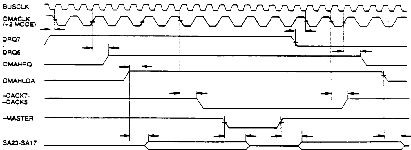
FIGURE 8. MASTER MODE TIMING
