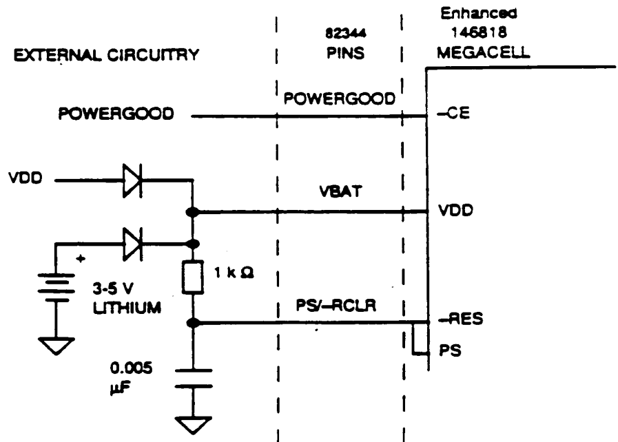
FIGURE 4. RTC LOW POWER OPERATION CIRCUIT
