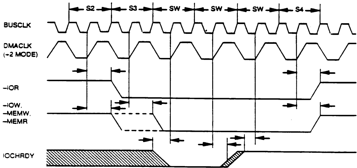
FIGURE 9. IOCHRDY TIMING
