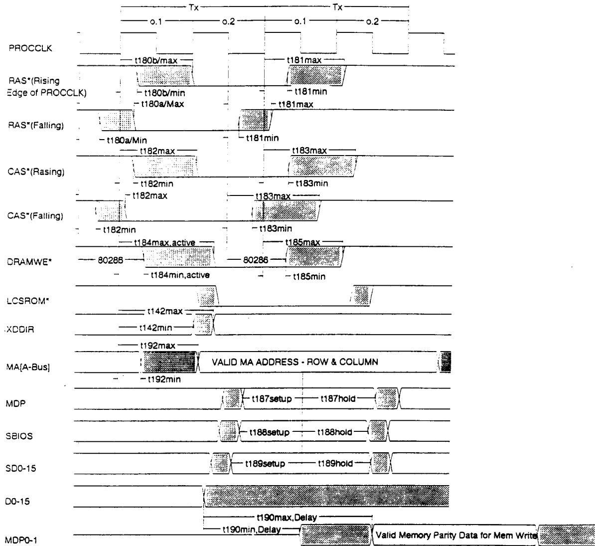
A.C. WAVEFORMS - MEMORY SPECIFICATION - Output Valid Delay for Memory Interface
