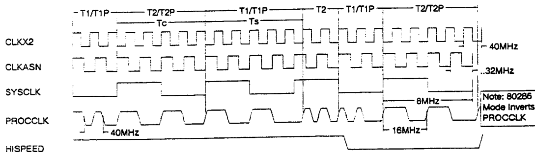
CLOCK SWITCHING DIAGRAM PROCessor Clock - High speed Clock X 2 switch to Low speed 1/2 ClocKASN Input - Low speed, 1/2 CLKASN to High speed, CLKX2 - HISPEED Switch High to Low
