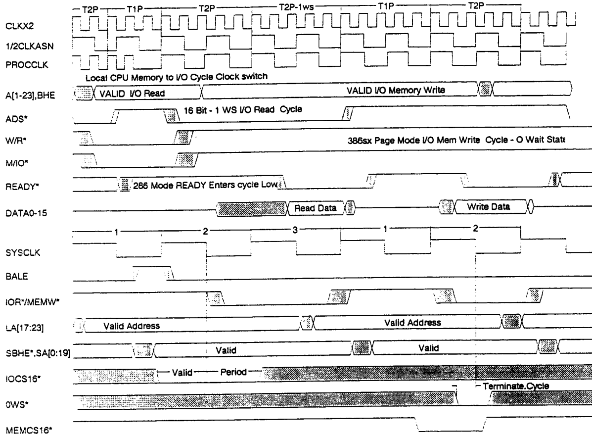
I/O BUS FUNCTIONAL TIMING - Standard Read Cycle and Ows I/O Memory Write Cycle
