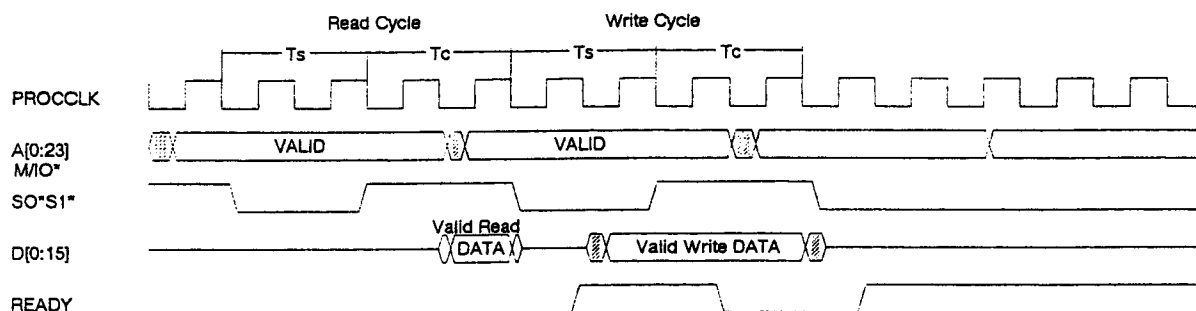
80286 CPU FUNCTIONAL TIMING - Read and Write Cycles
