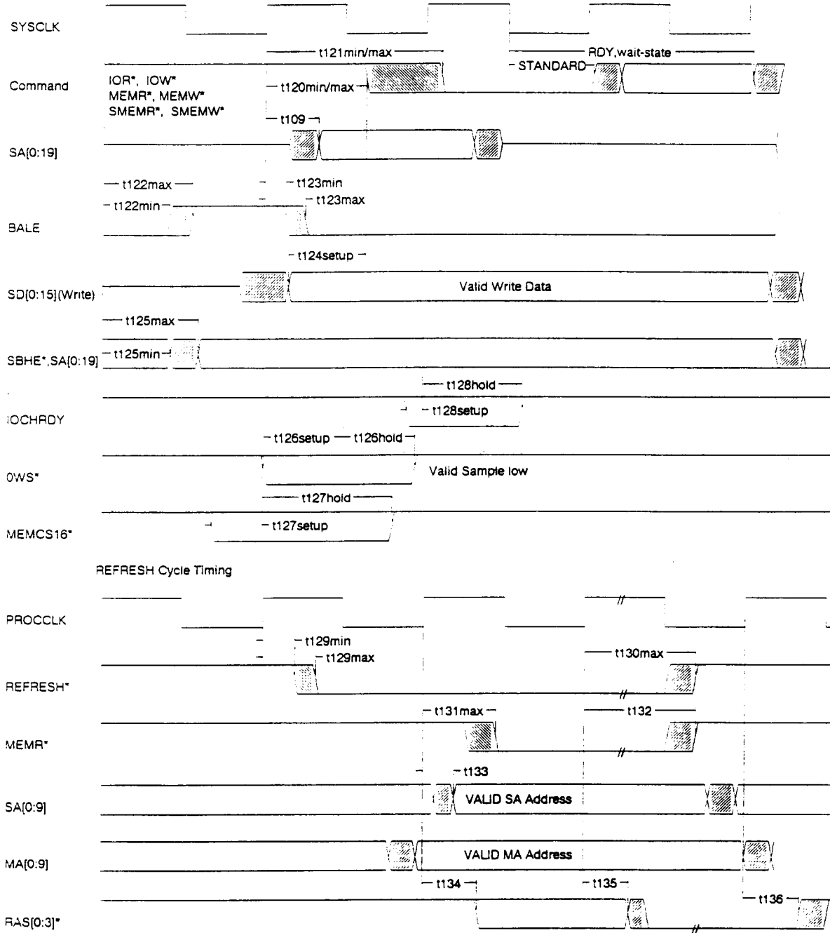
A.C. WAVEFORMS - IO INTERFACE Timing
