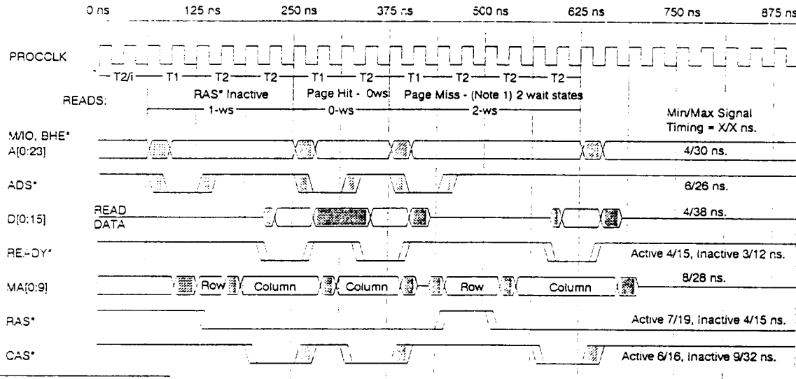
PAGE MODE FUNCTIONAL MEMORY TIMING - Read Cycles, 80386SX, Non-Pipelined Addressing
