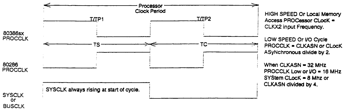
CPU PROCESSOR CLOCK RELATIONSHIPS
