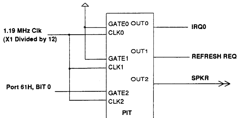
Programmable Interval Timer
