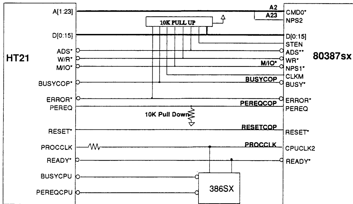
NPU Interface
