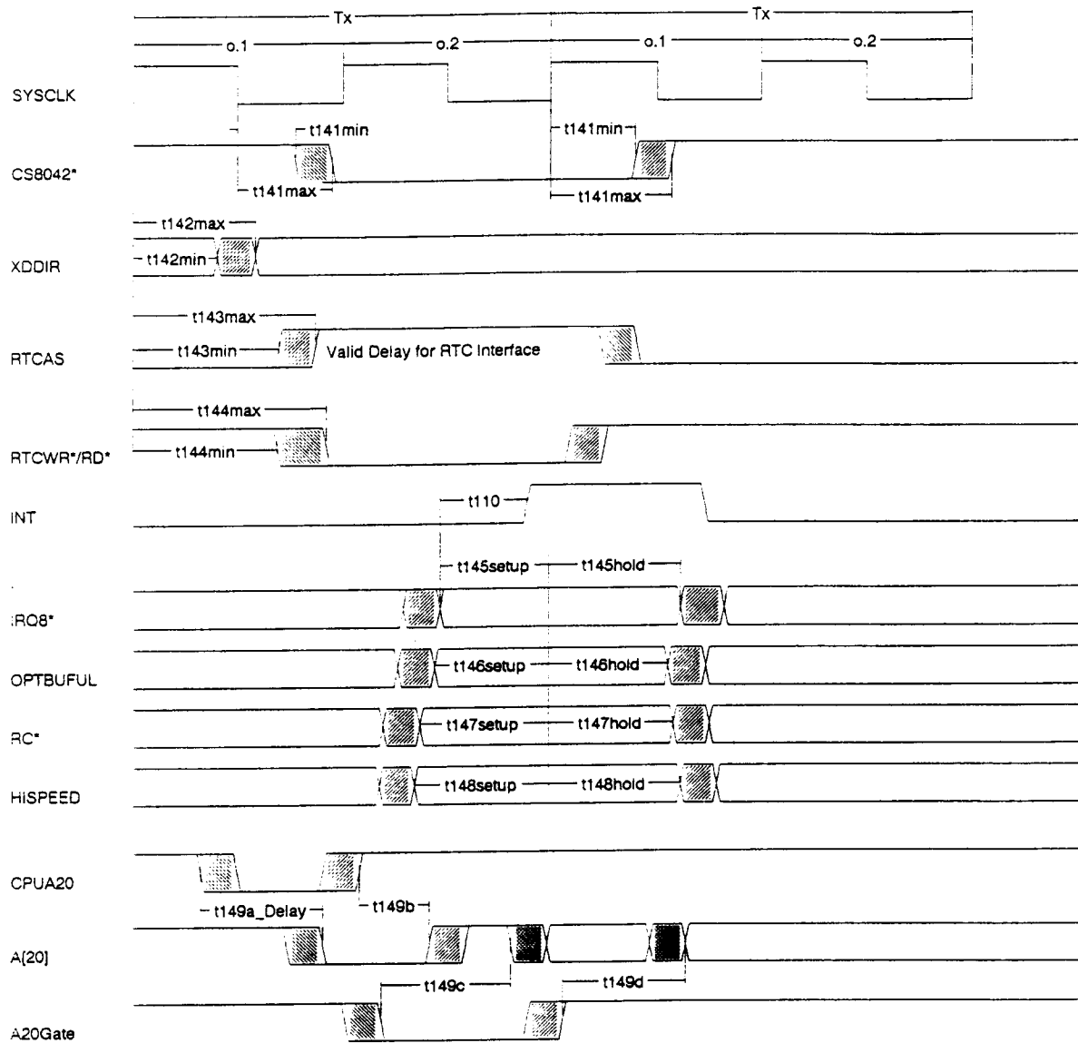
A.C. WAVEFORMS - Valid Delay, Setup and Hold timing for Keyboard and RTC Interface
