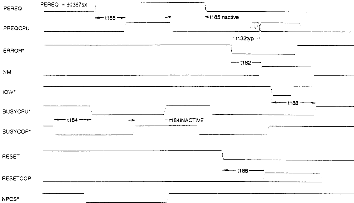
A.C. WAVEFORMS - NPU Interface - Signals shown for timing reference
