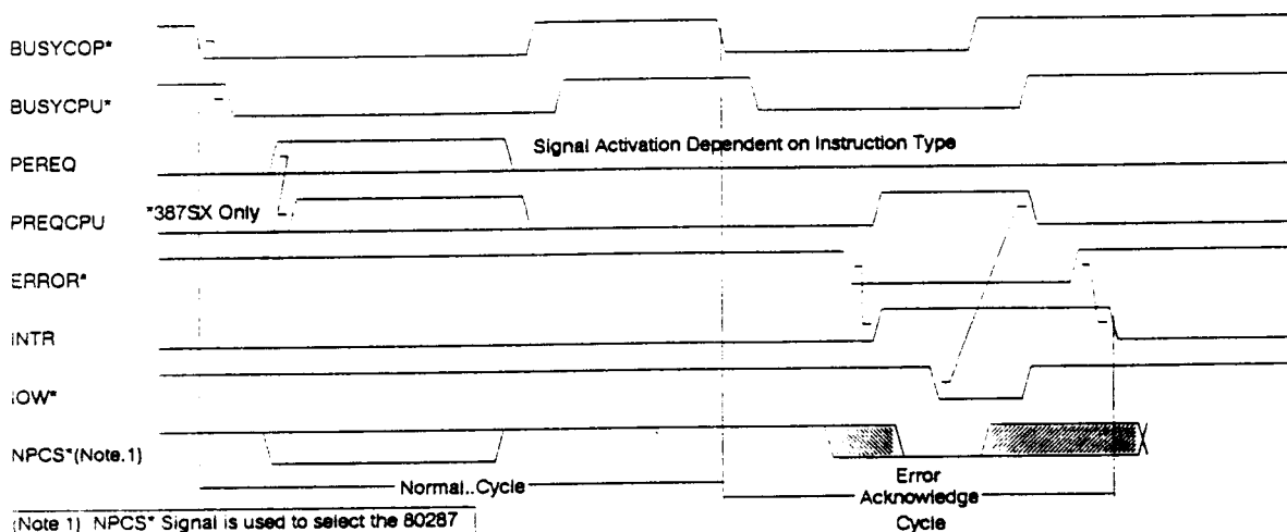
NPU FUNCTIONAL TIMING DIAGRAM - NPU Bus/CPU Interface Cycles
