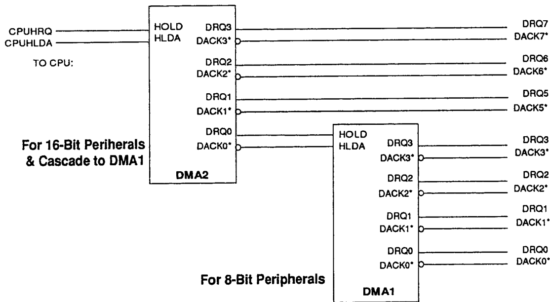
Cascaded DMA Controllers
