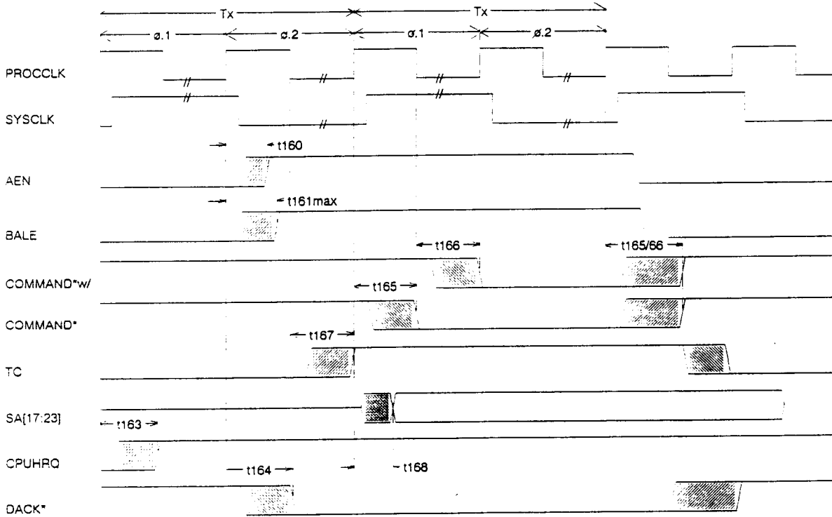
A.C. WAVEFORMS - Output Valid Delay, Setup and Hold timing for I/O Interface, DMA Signals
