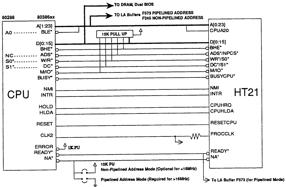
CPU Interface Diagram
