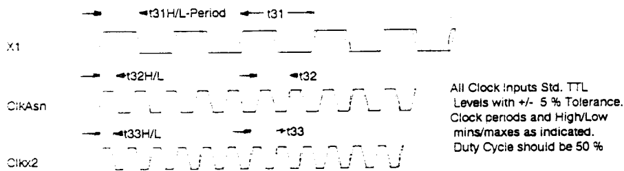
A.C. WAVEFORMS - INPUT CLOCK SPECIFICATIONS
