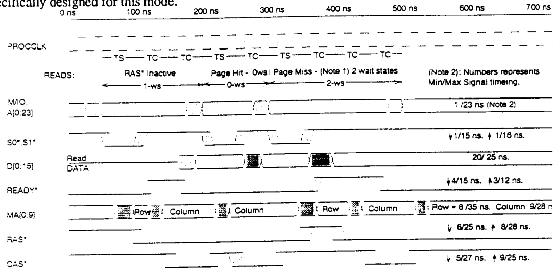
PAGE MODE FUNCTIONAL MEMORY TIMING - Read Cycles, 80286 Operation
