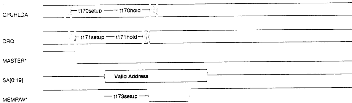
A.C. WAVEFORMS - Output Valid Delay, Setup and Hold timing for I/O Interface, DMA Signals
