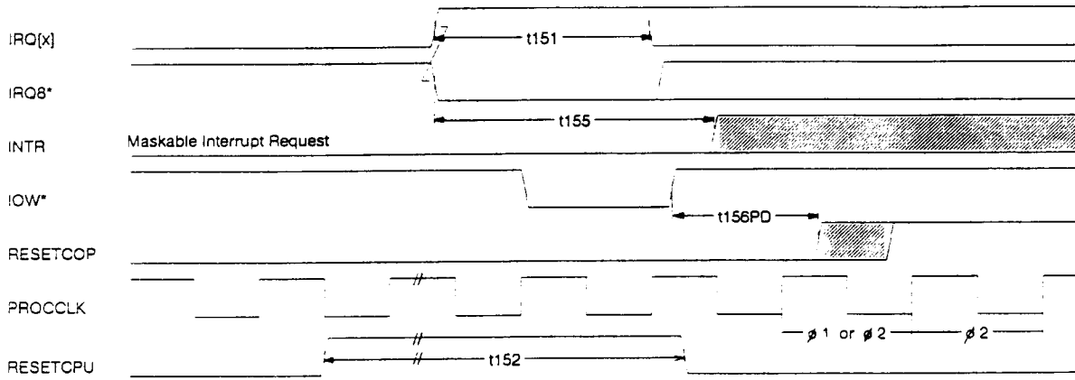
A.C. WAVEFORMS - INTERRUPT AND RESET SIGNAL SPECS - Interrupt Signals and Reset
