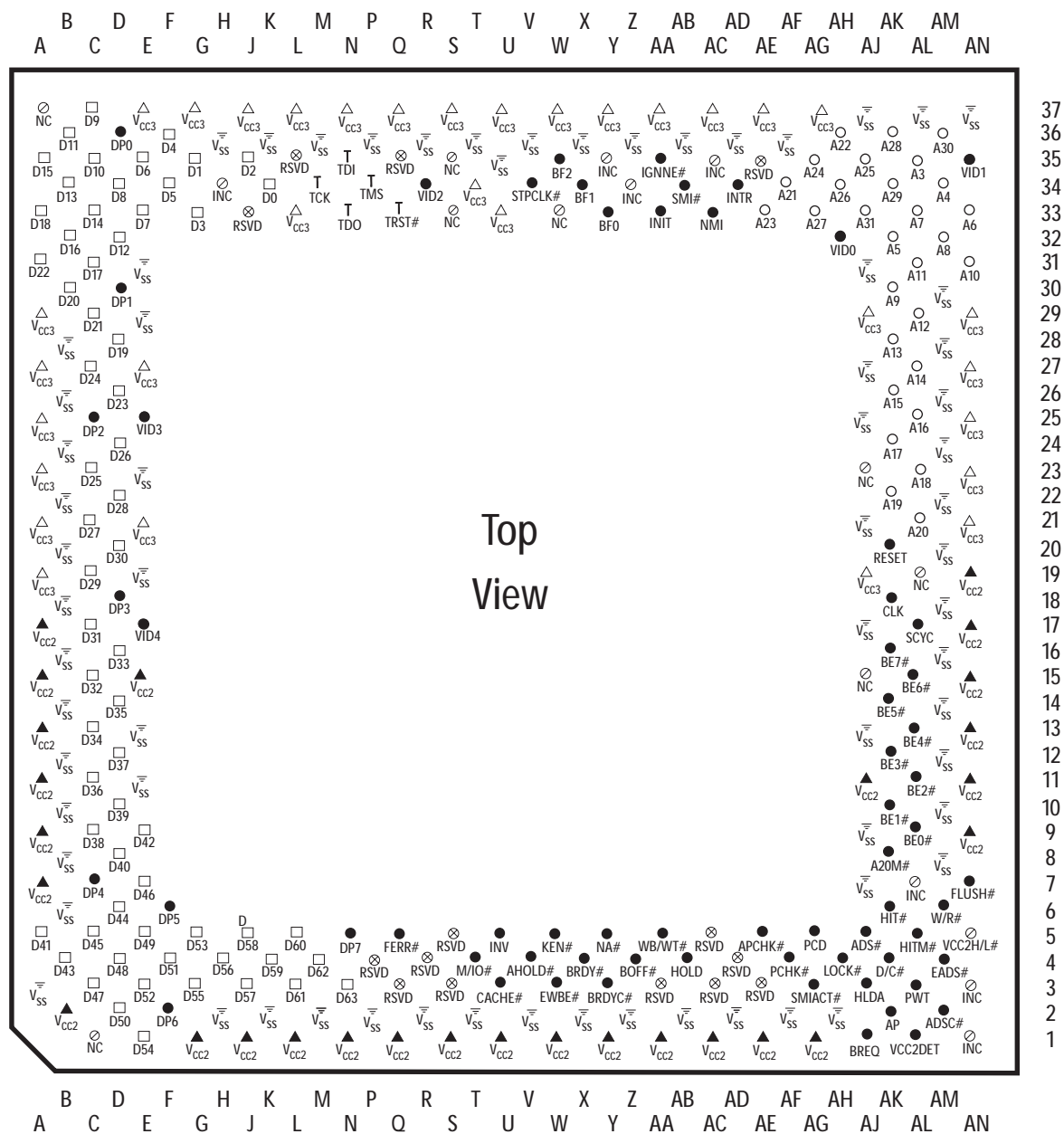
Figure 116. Mobile AMD-K6®-2+ Processor Top-Side View
