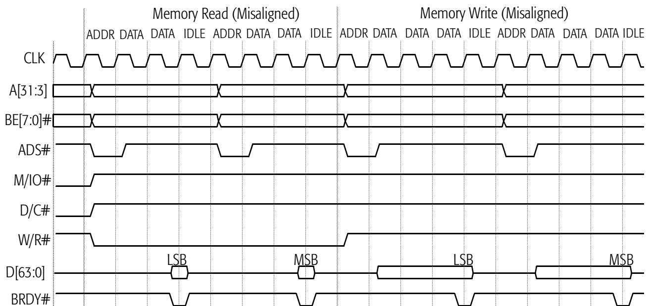
Figure 57. Misaligned Single-Transfer Memory Read and Write
