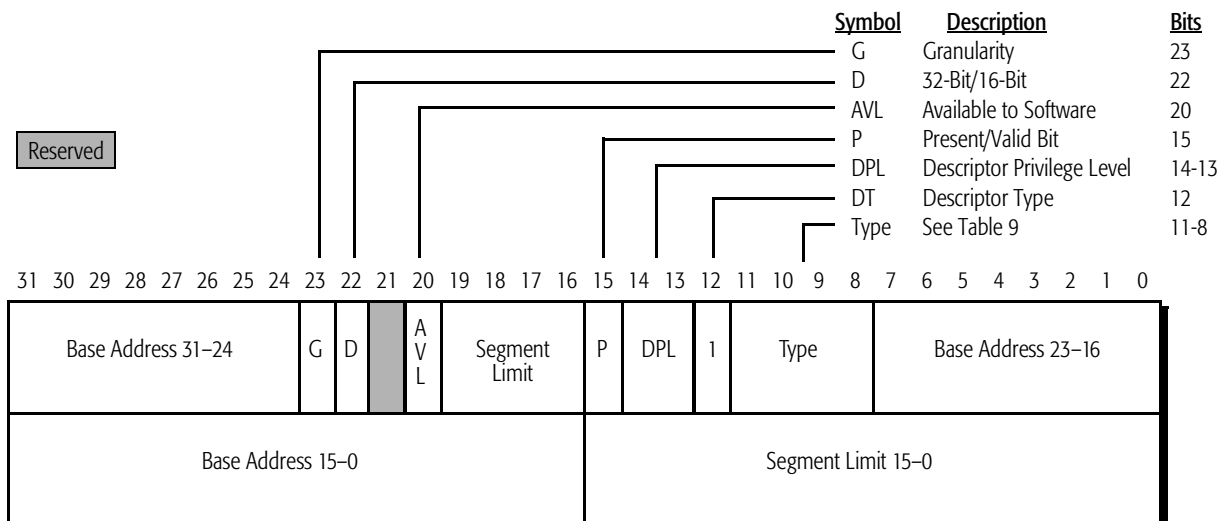
Figure 50. Application Segment Descriptor
