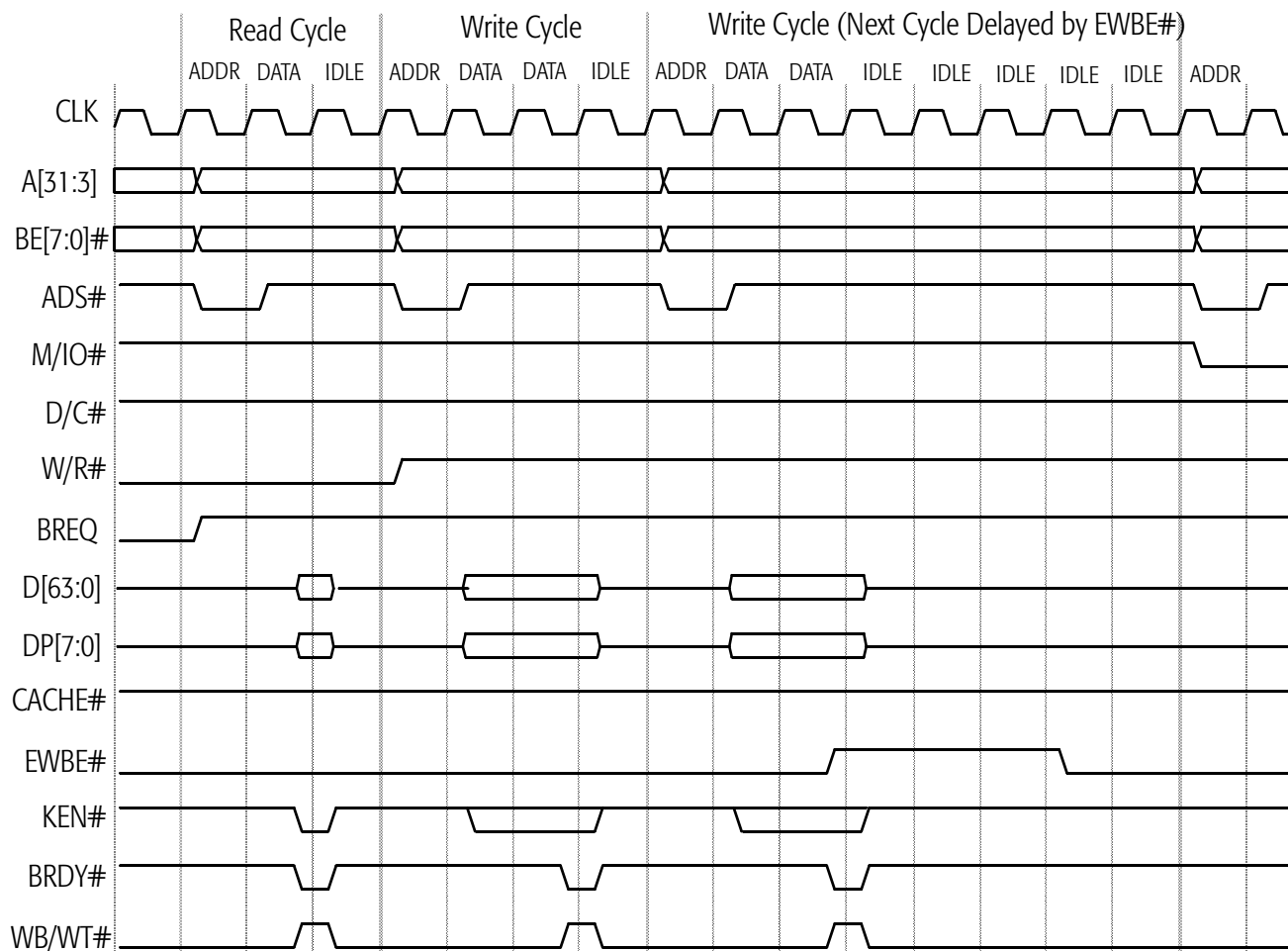
Figure 56. Non-Pipelined Single-Transfer Memory Read/Write and Write Delayed by EWBE#
