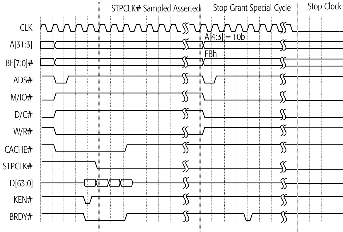
Figure 75. Stop Grant and Stop Clock Modes, Part 1
