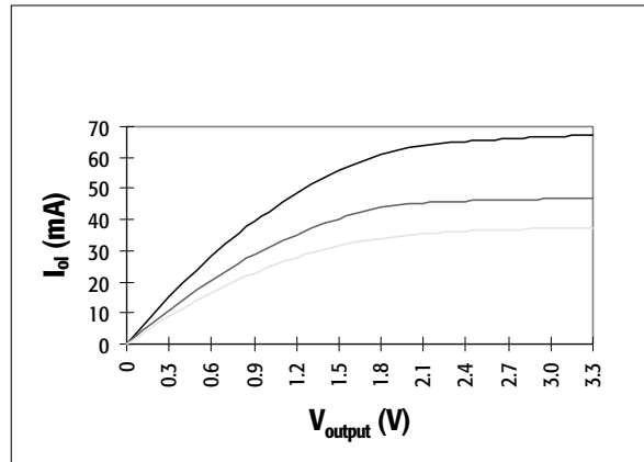
Figure 99. Pulldown V/I Curves
