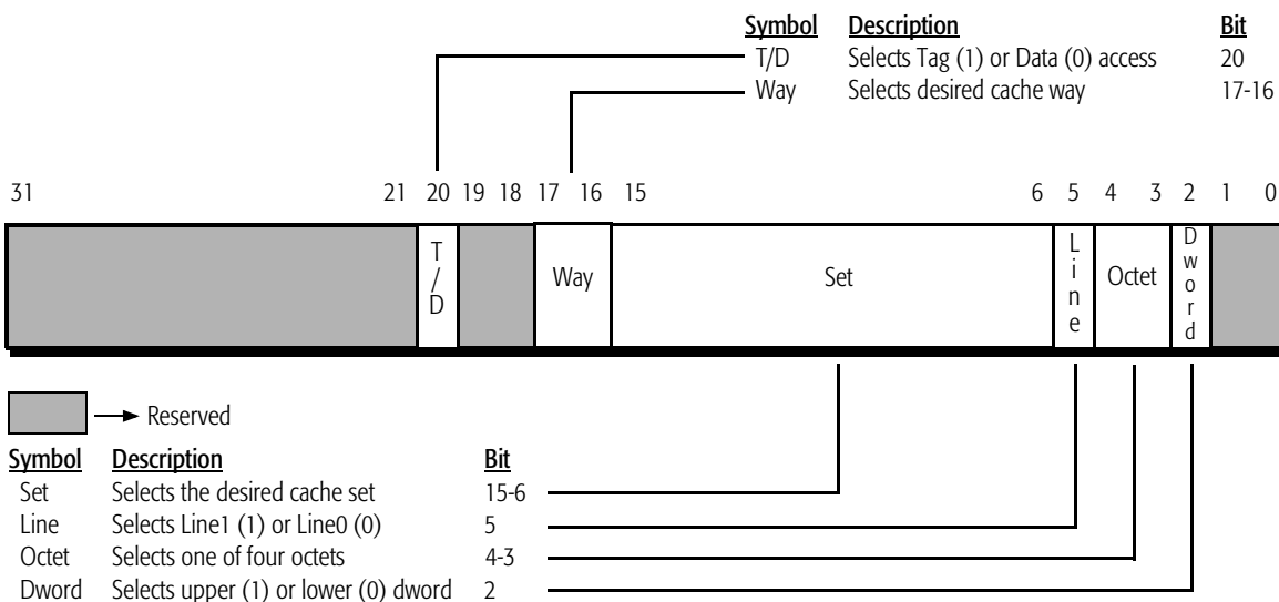
Figure 89. L2 Tag or Data Location - EDX
