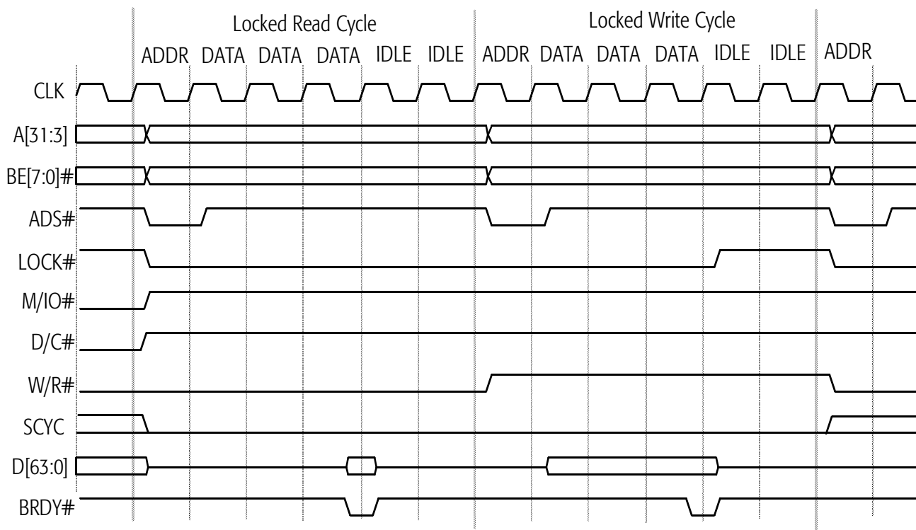
Figure 70. Basic Locked Operation
