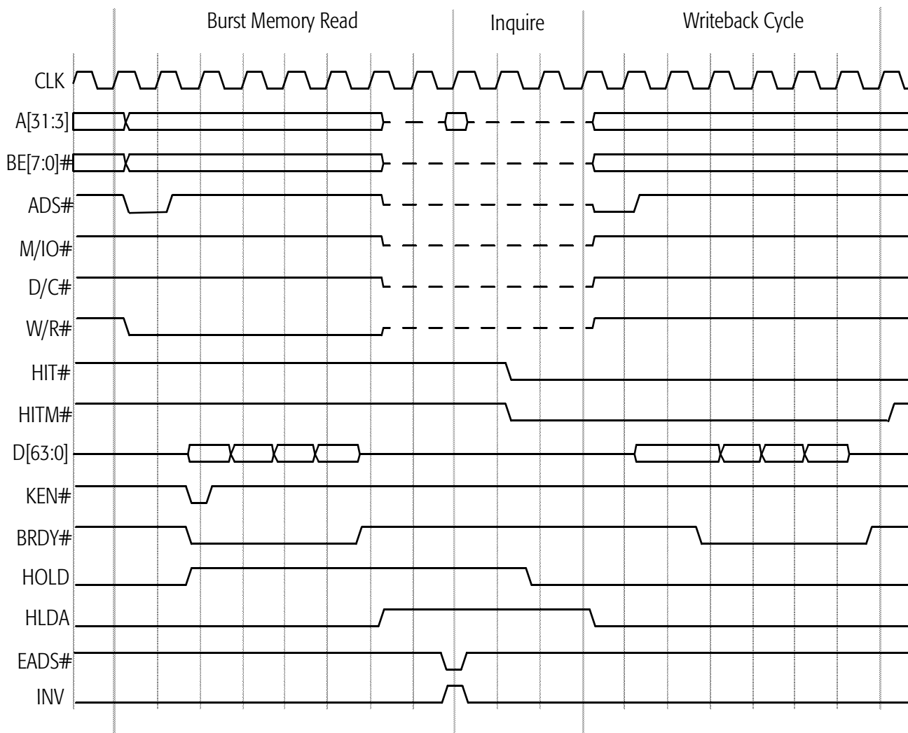
Figure 64. HOLD-Initiated Inquire Hit to Modified Line
