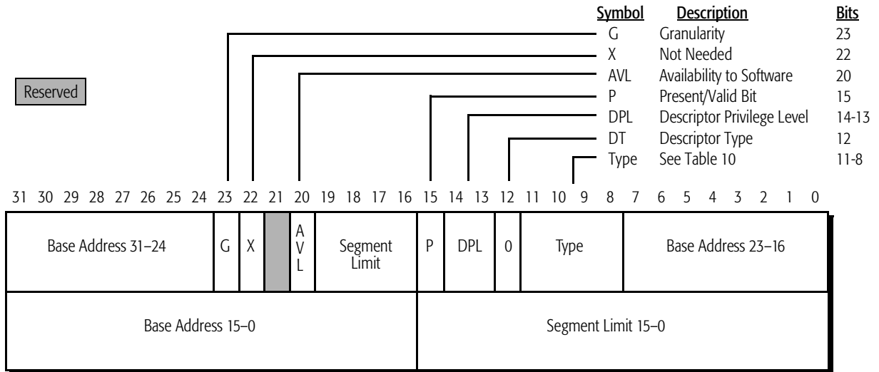
Figure 51. System Segment Descriptor
