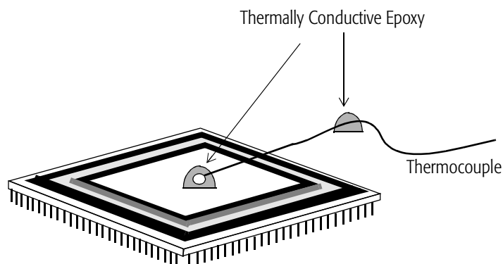
Figure 113. Measuring Case Temperature
