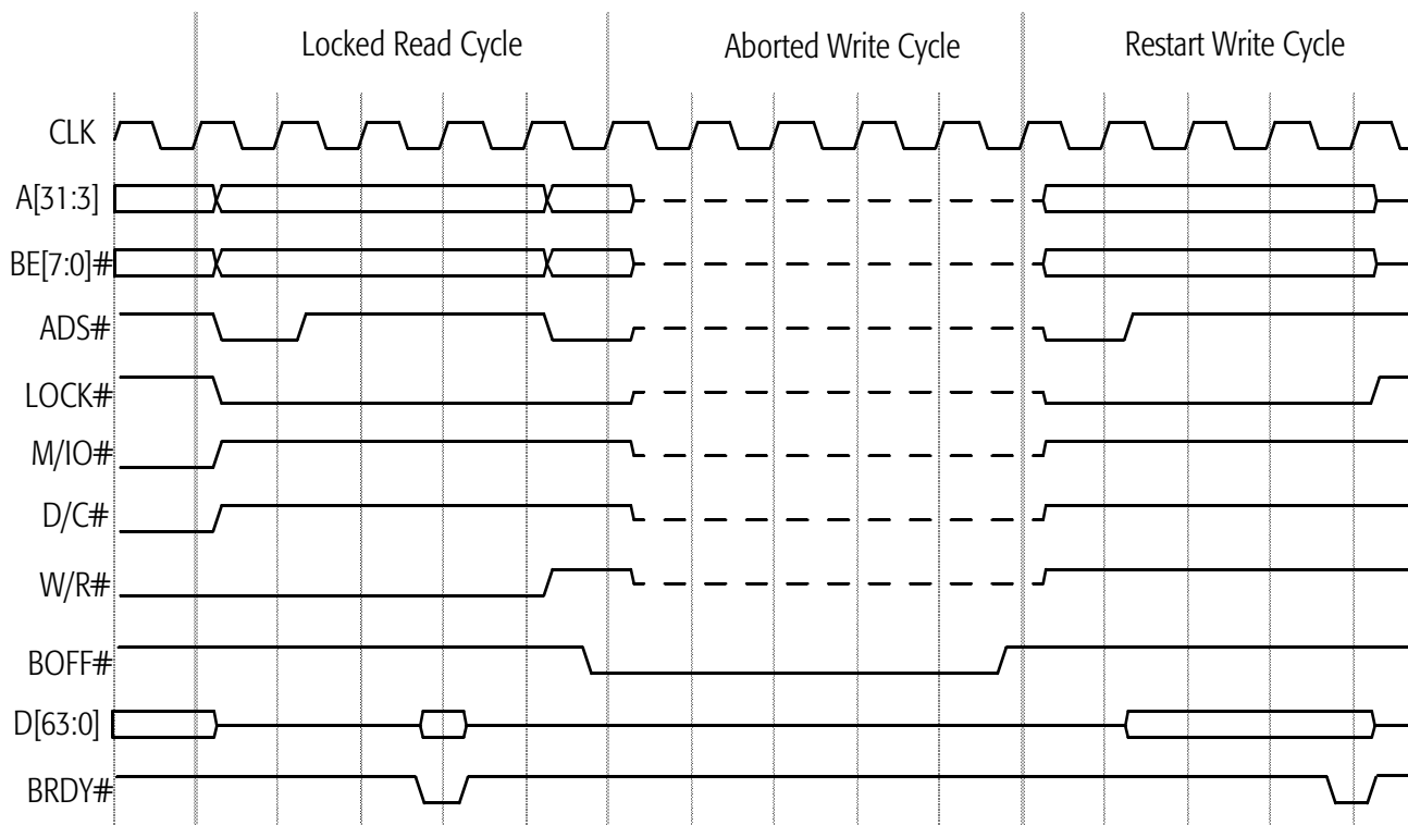
Figure 71. Locked Operation with BOFF# Intervention
