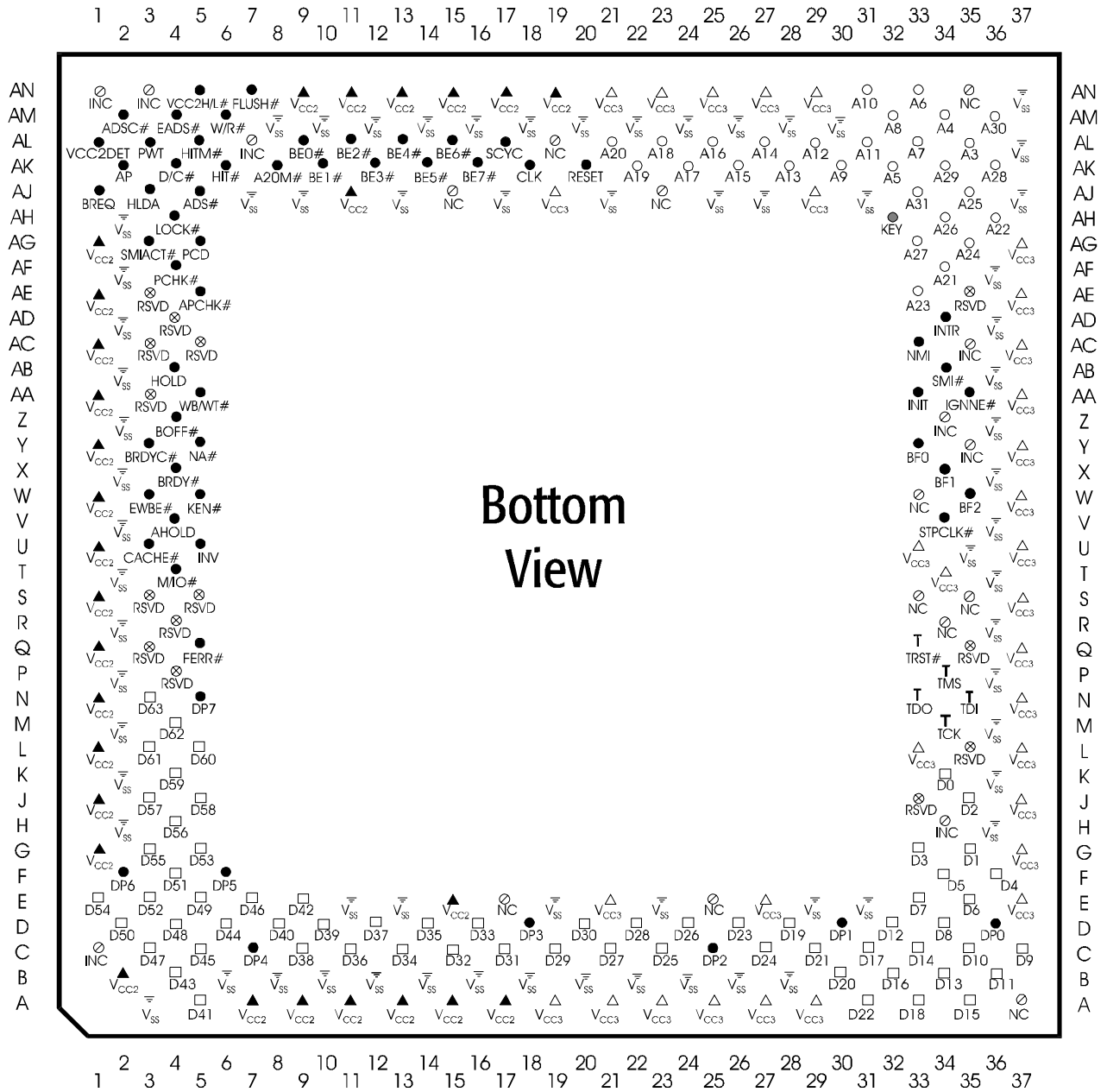
Figure 119. AMD-K6®-III Processor Pin-Side View
