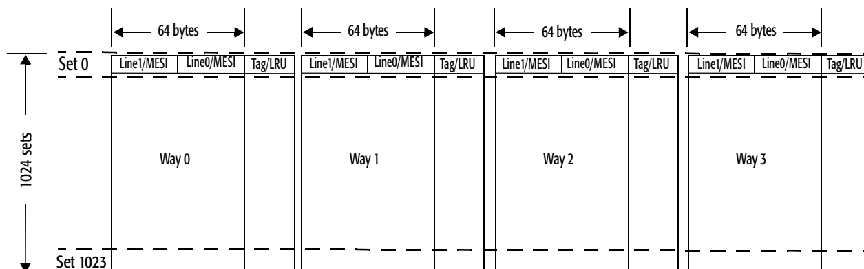
Figure 87. L2 Cache Organization
