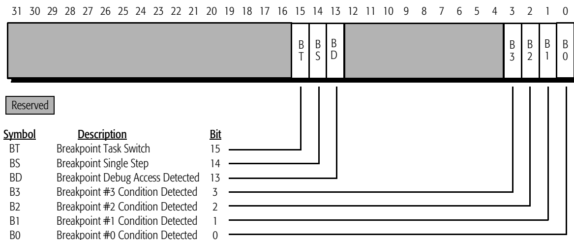
Figure 94. Debug Register DR6
