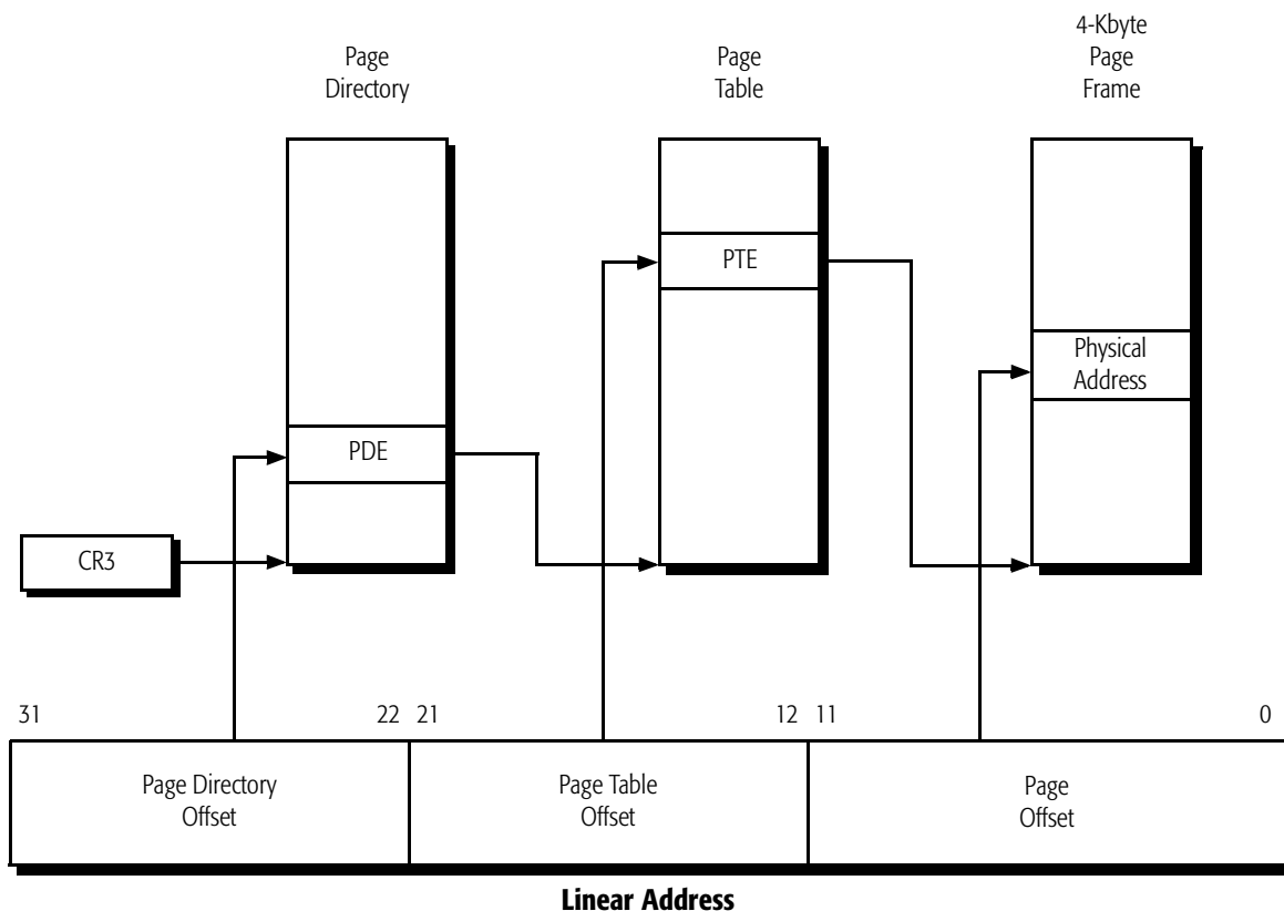
Figure 45. 4-Kbyte Paging Mechanism
