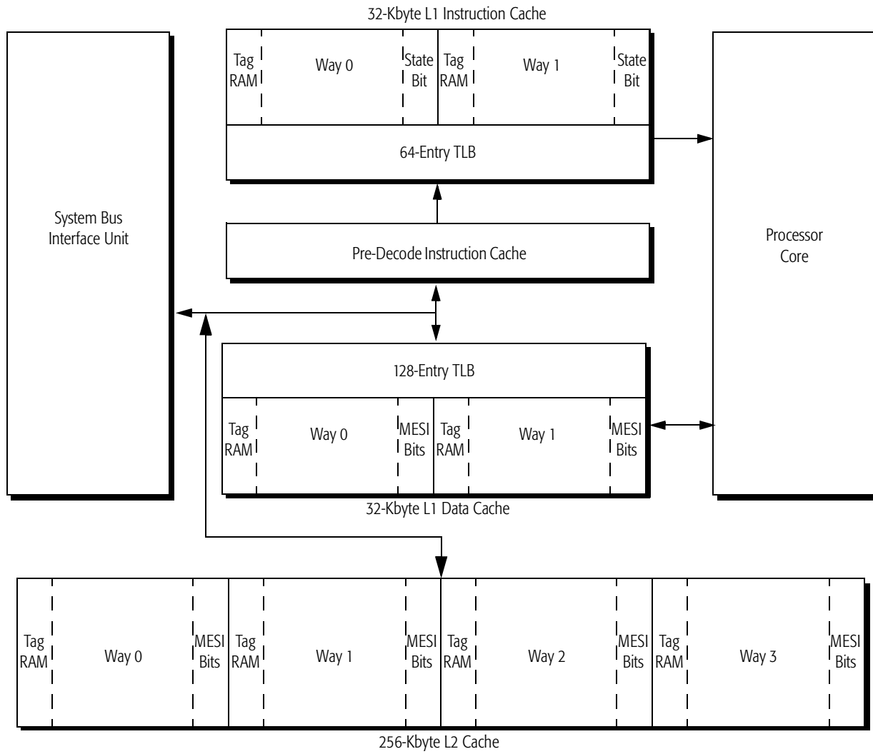
Figure 78. L1 and L2 Cache Organization
