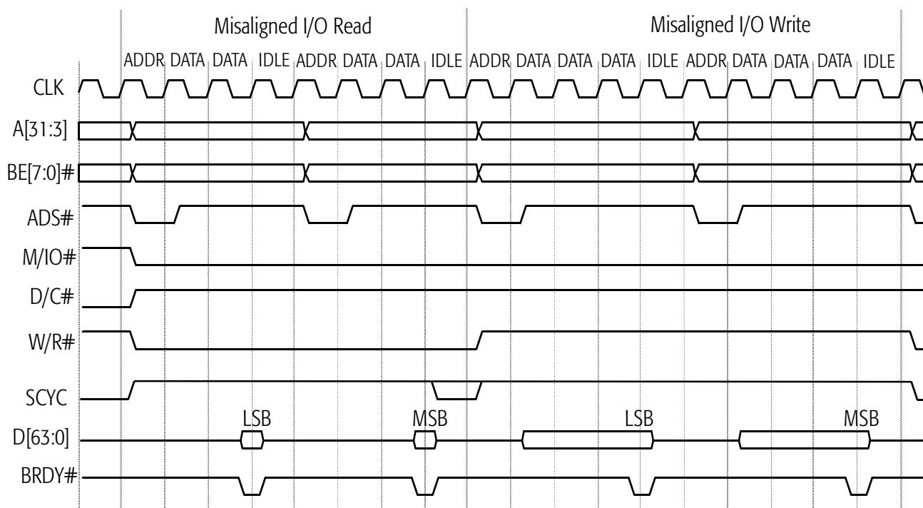
Figure 61. Misaligned I/O Transfer
