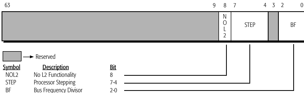
Figure 38. Processor State Observability Register (PSOR)—MSR C000_0087h
