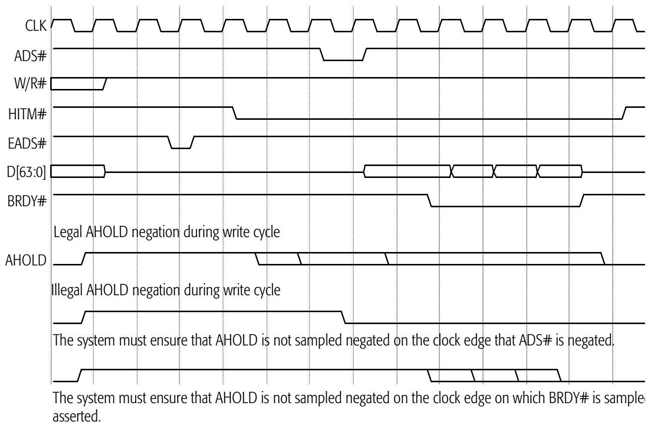
Figure 68. AHOLD Restriction
