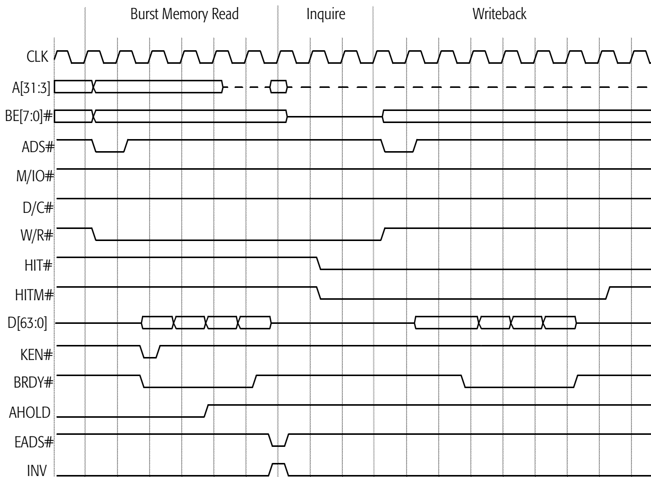
Figure 67. AHOLD-Initiated Inquire Hit to Modified Line
