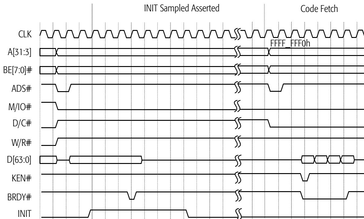
Figure 77. INIT-Initiated Transition from Protected Mode to Real Mode
