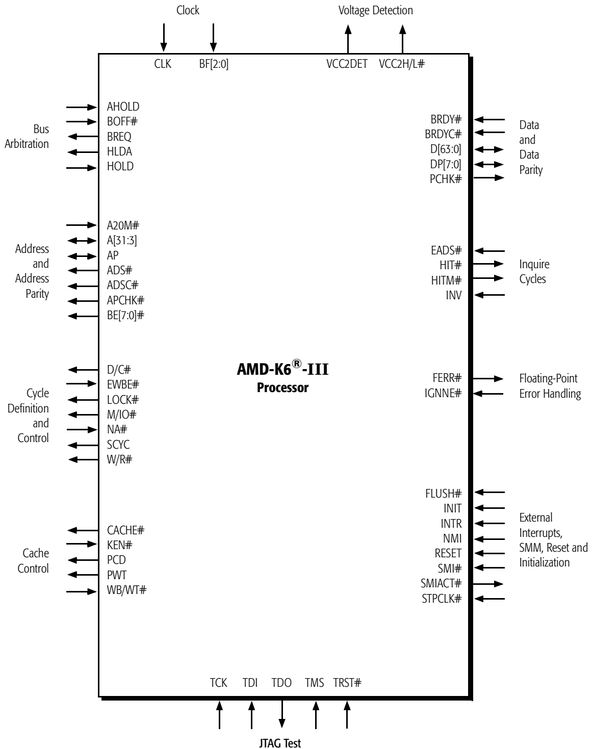
Figure 53. Logic Symbol Diagram
