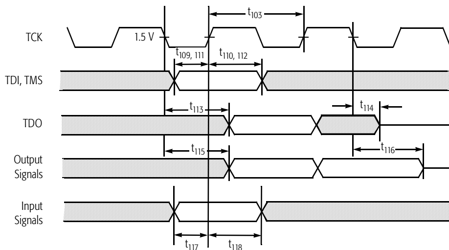
Figure 109. Test Signal Timing Diagram
