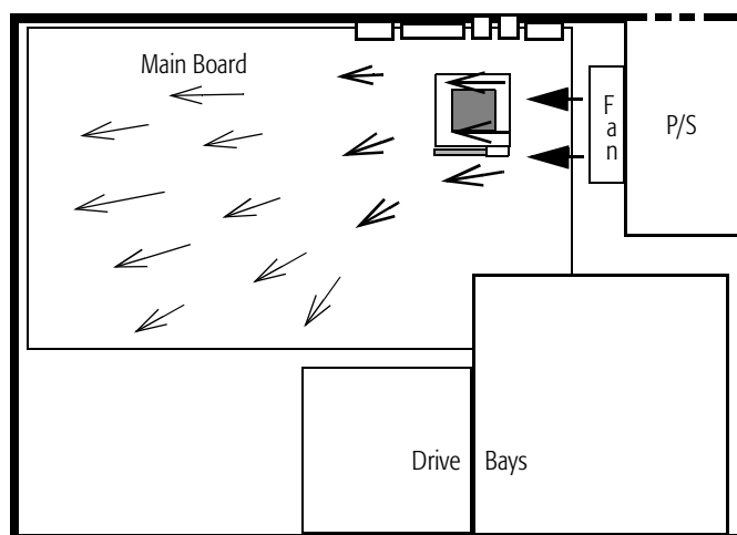
Figure 117. Airflow Path in an ATX Form-Factor System
