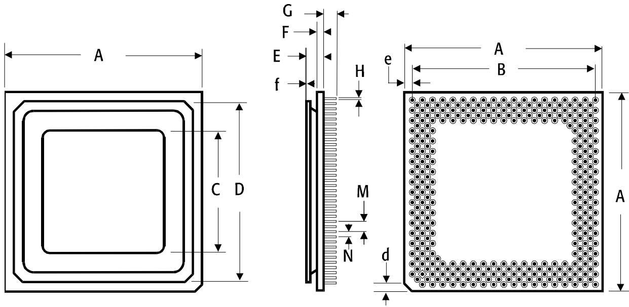
Figure 120. 321-Pin Staggered CPGA Package Specification
