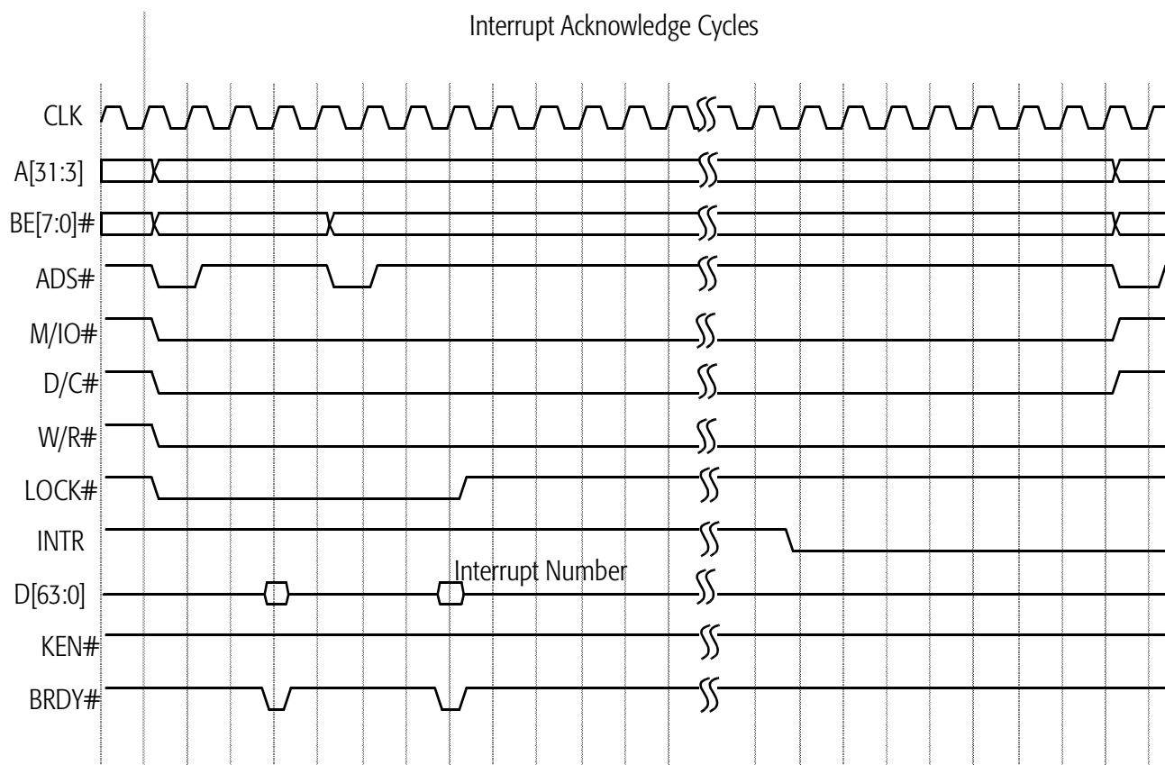
Figure 72. Interrupt Acknowledge Operation
