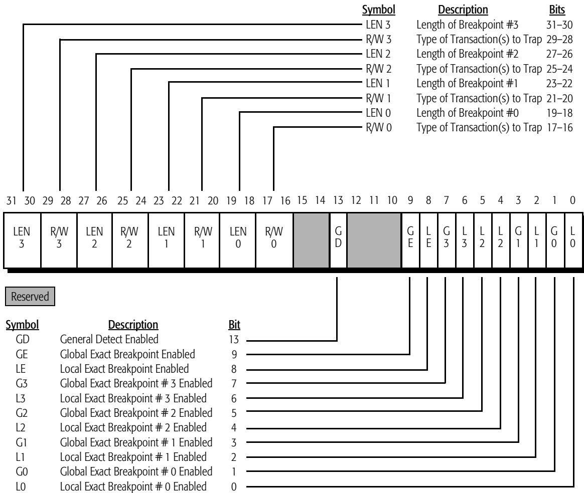
Figure 93. Debug Register DR7
