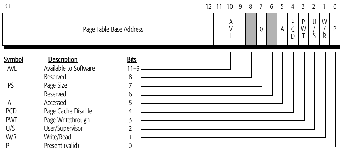
Figure 47. Page Directory Entry 4-Kbyte Page Table (PDE)
