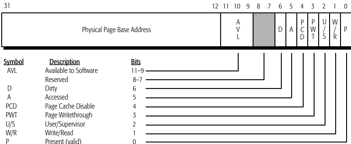
Figure 49. Page Table Entry (PTE)
