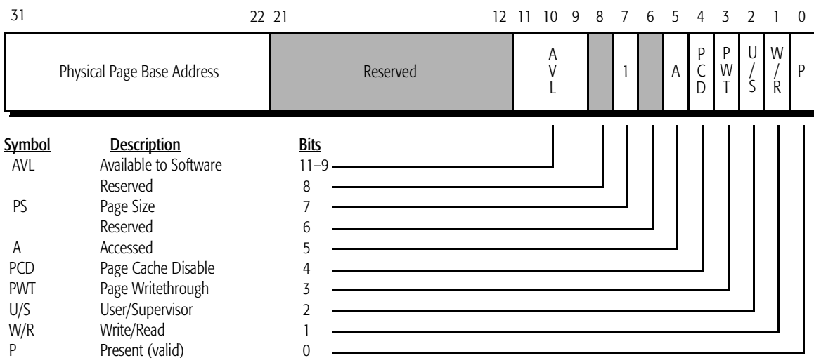
Figure 48. Page Directory Entry 4-Mbyte Page Table (PDE)
