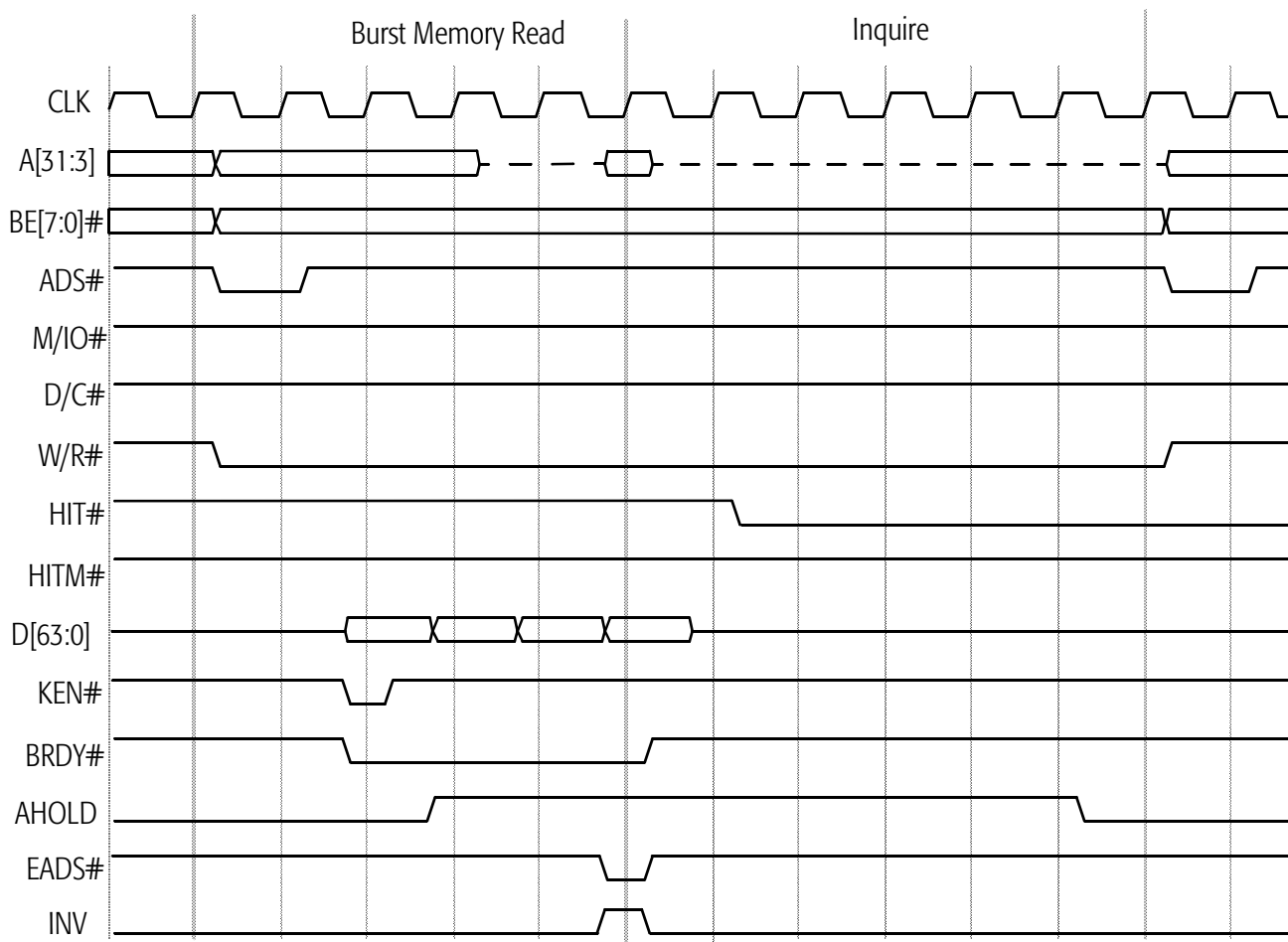
Figure 66. AHOLD-Initiated Inquire Hit to Shared or Exclusive Line
