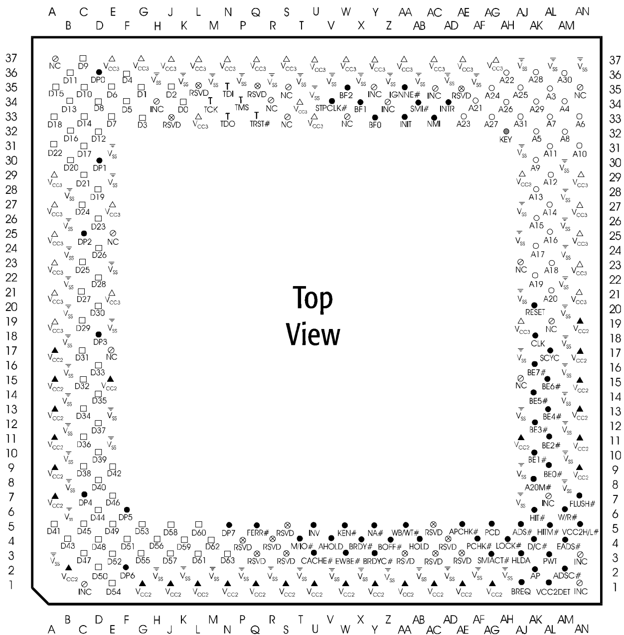
Figure 118. AMD-K6®-III Processor Top-Side View
