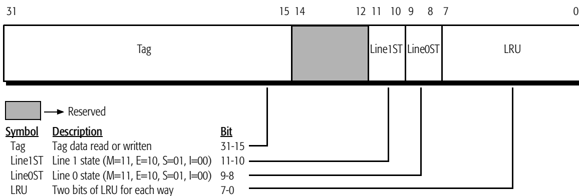
Figure 91. L2 Tag Information - EAX
