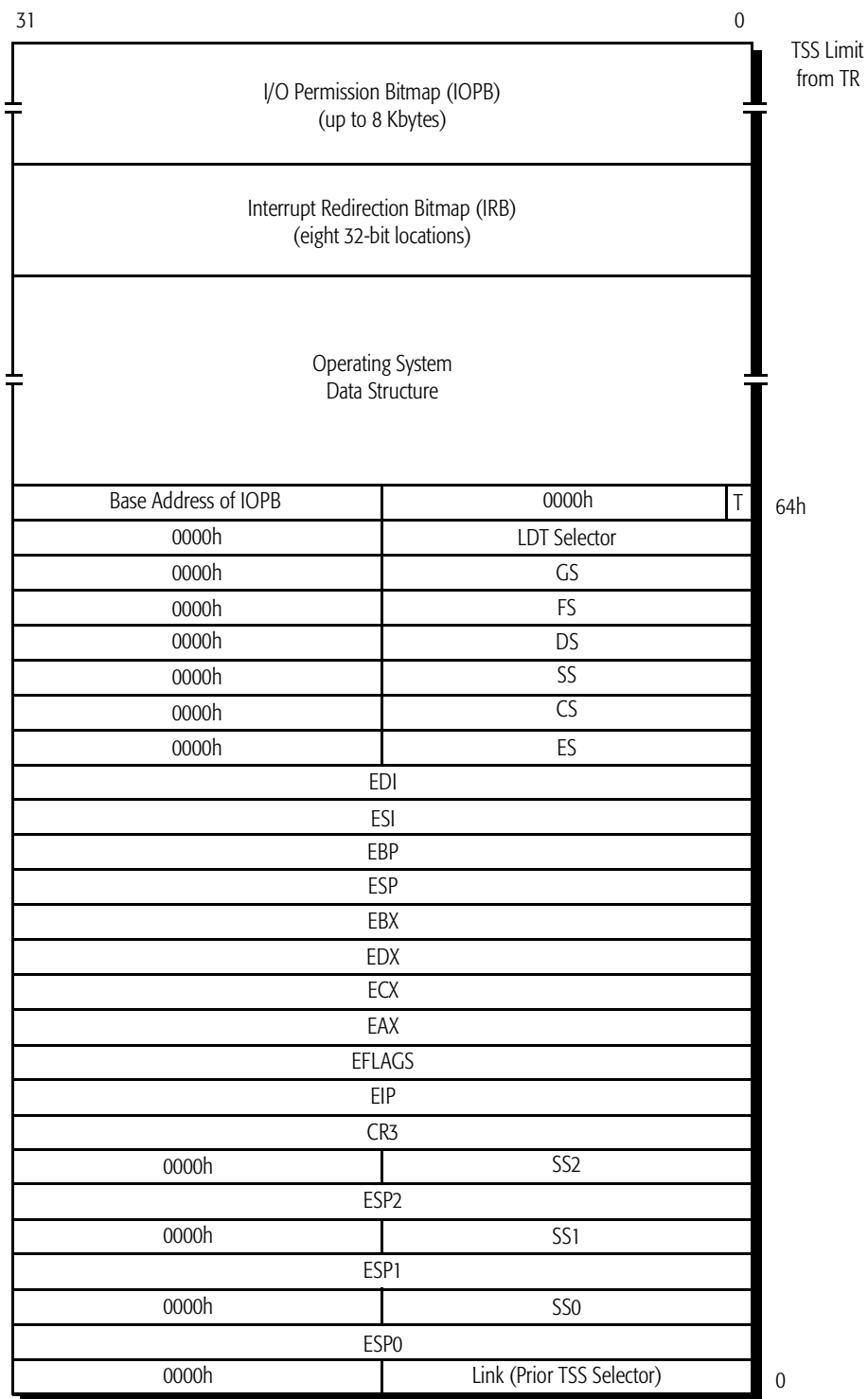
Figure 44. Task State Segment (TSS)
