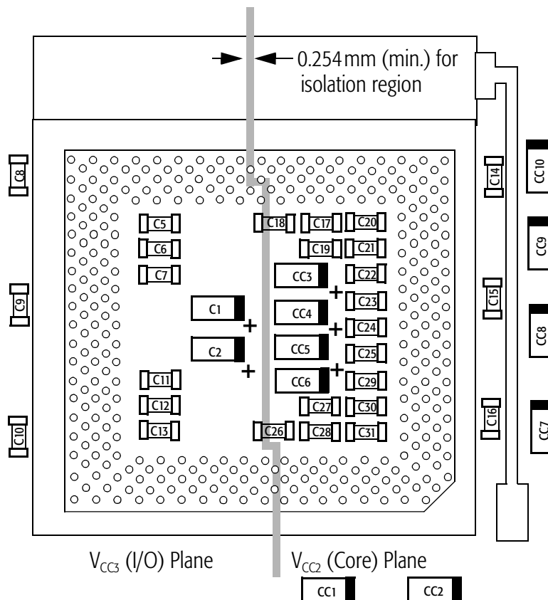
Figure 98. Suggested Component Placement
