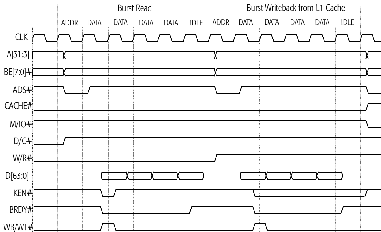
Figure 59. Burst Writeback due to Cache-Line Replacement
