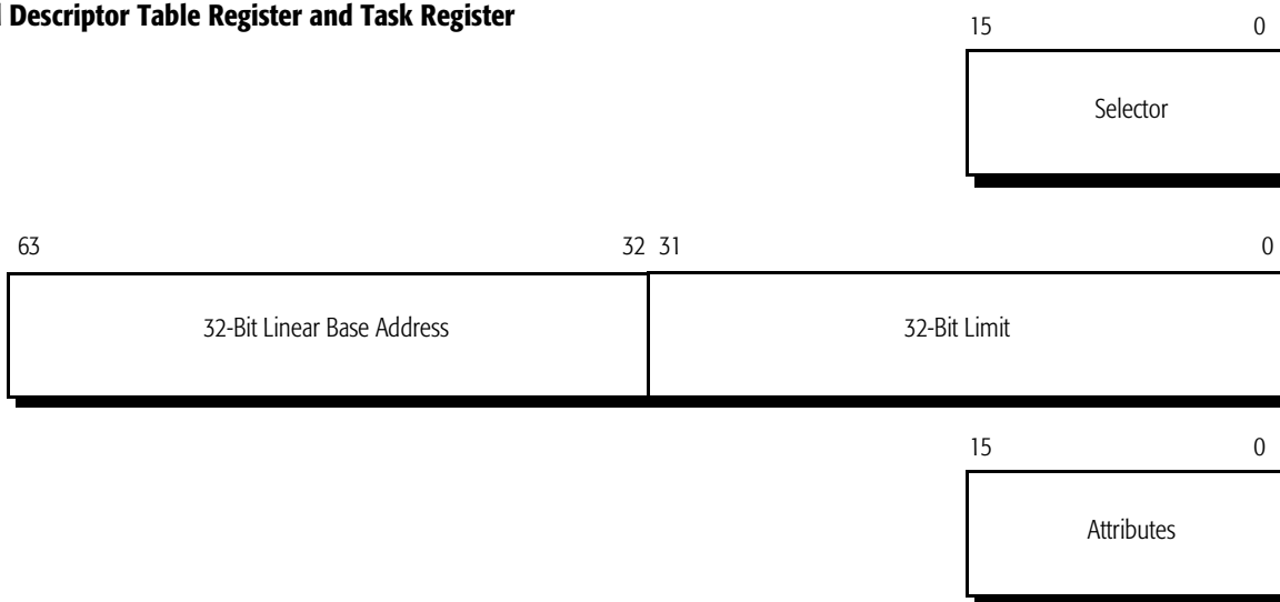
Figure 43. Memory Management Registers
