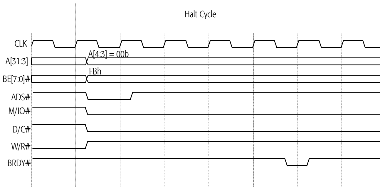
Figure 73. Basic Special Bus Cycle (Halt Cycle)
