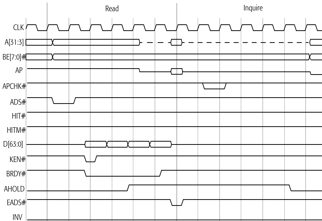
Figure 65. AHOLD-Initiated Inquire Miss
