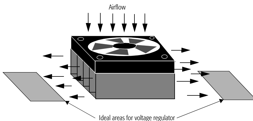
Figure 115. Airflow for a Heatsink with Fan
