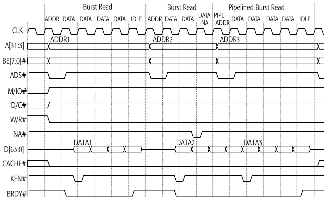
Figure 58. Burst Reads and Pipelined Burst Reads
