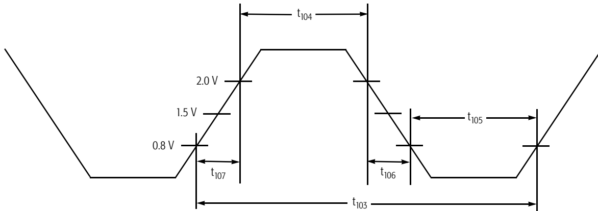
Figure 107. TCK Waveform
