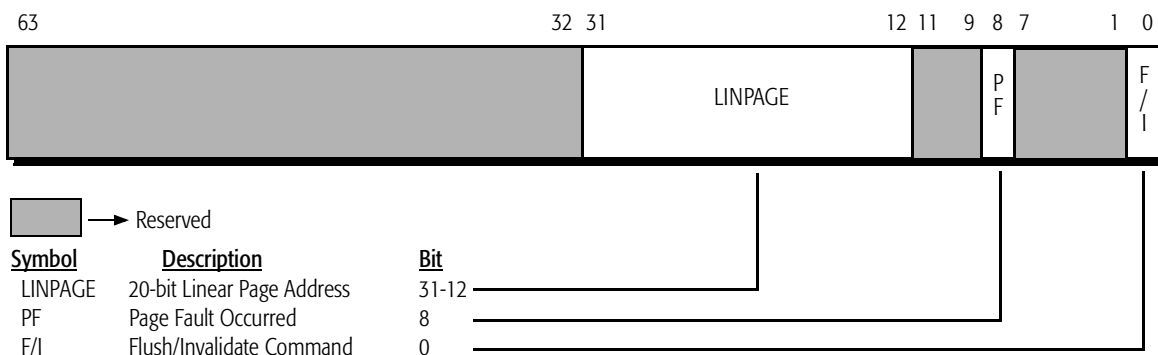
Figure 39. Page Flush/Invalidate Register (PFIR)—MSR C000_0088h
