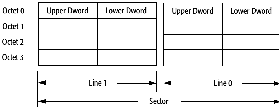
Figure 88. L2 Cache Sector and Line Organization
