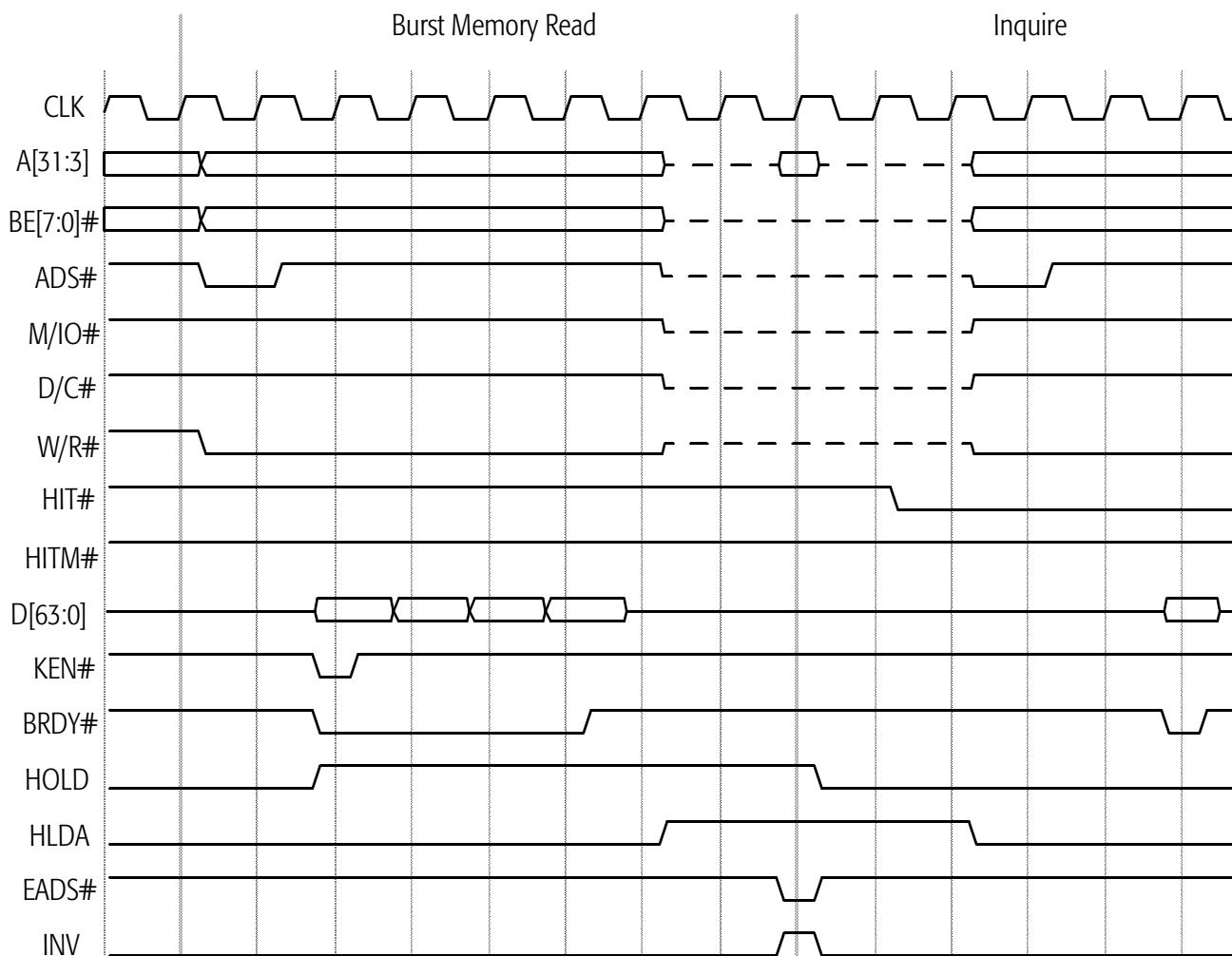
Figure 63. HOLD-Initiated Inquire Hit to Shared or Exclusive Line
