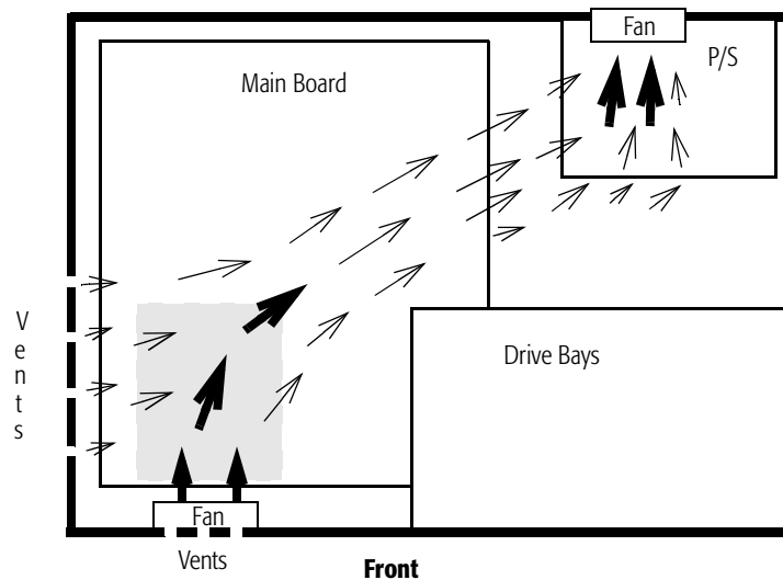
Figure 116. Airflow Path in a Dual-Fan System
