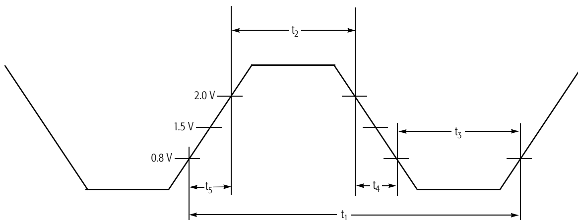
Figure 101. CLK Waveform
