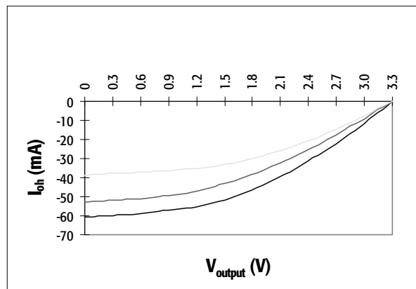
Figure 100. Pullup V/I Curves
