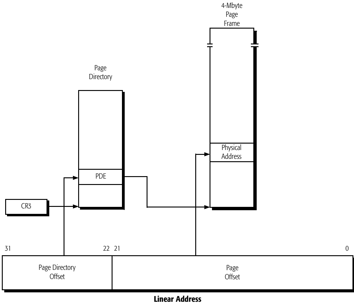
Figure 46. 4-Mbyte Paging Mechanism
