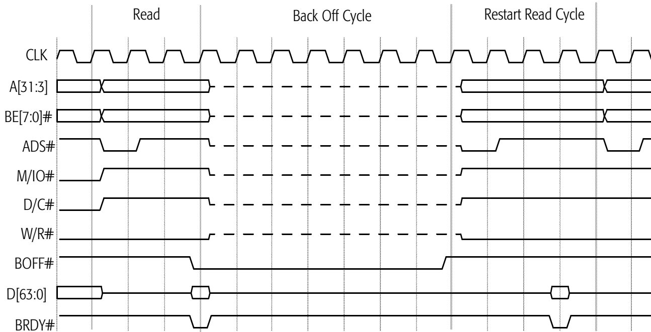
Figure 69. BOFF# Timing
