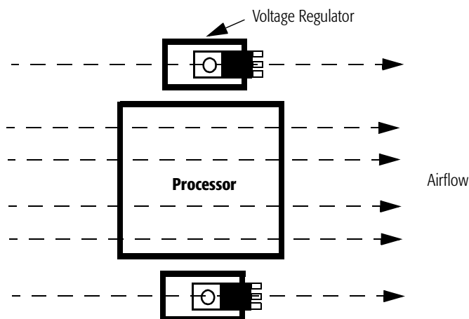
Figure 114. Voltage Regulator Placement
