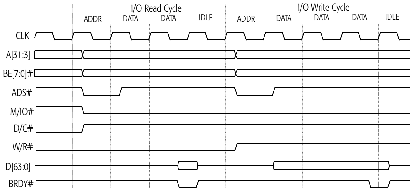
Figure 60. Basic I/O Read and Write
