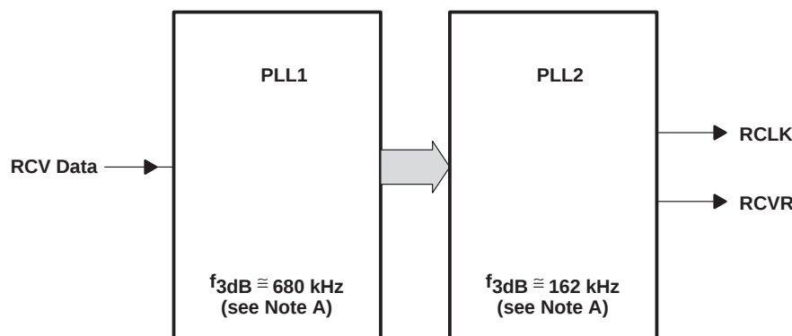
Figure 3. Dual PLL Arrangement
