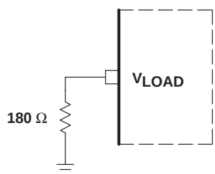
(c) I_{ref} TEST CIRCUIT
