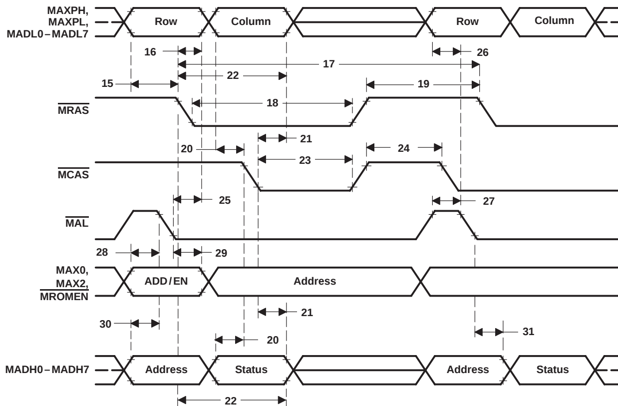
Figure 12. Memory-Bus Timing: Clocks, \overline{\text{MRAS}} , \overline{\text{MCAS}} , and \overline{\text{MAL}} to ADDRESS
