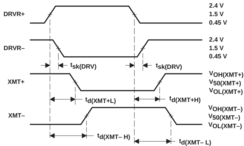
Figure 7. Transmitter Timing
