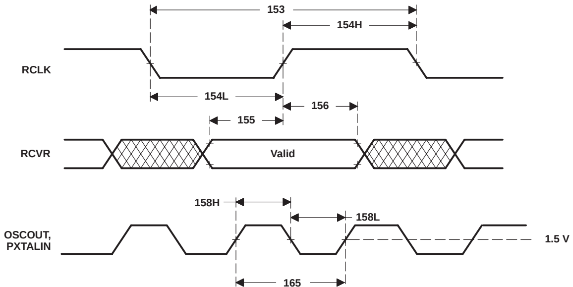
Figure 17. Ring-Interface Timing
