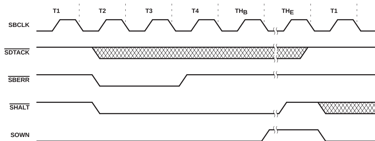
Figure 39. 68xxx-Mode Bus-Halt and Retry, Rerun Cycle With Delayed Start
