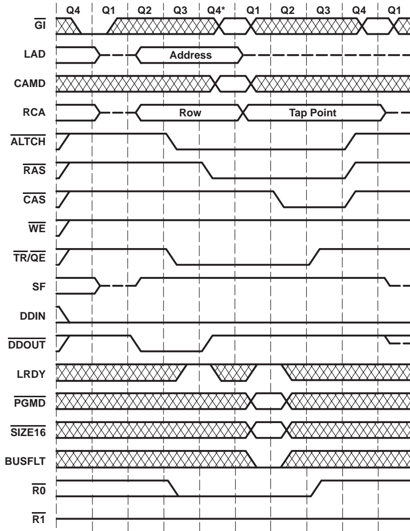
Figure 15. Memory-to-Split-Serial-Data-Register Cycle (VRAM Split-Register Read Transfer)
