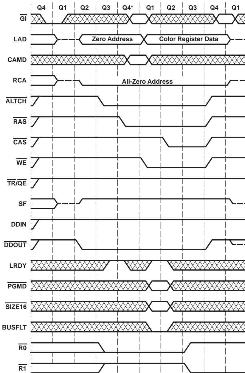
Figure 10. Load-Color-Latch Cycle
