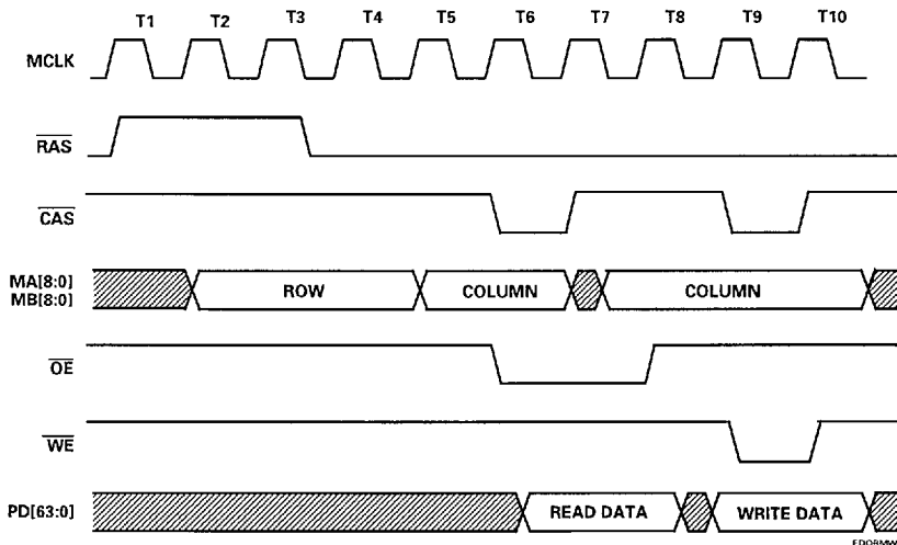
Figure 3-4. EDO Mode Read/Modify Write Timing
