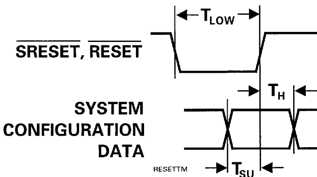
Figure 4-4. Reset Timing
