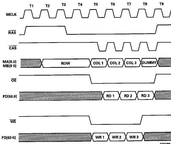
Figure 3-5. 1 Cycle EDO Read/Write Timing
