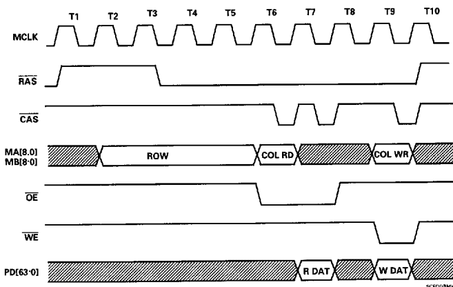
Figure 3-6. 1 Cycle EDO Read/Modify/Write Timing
