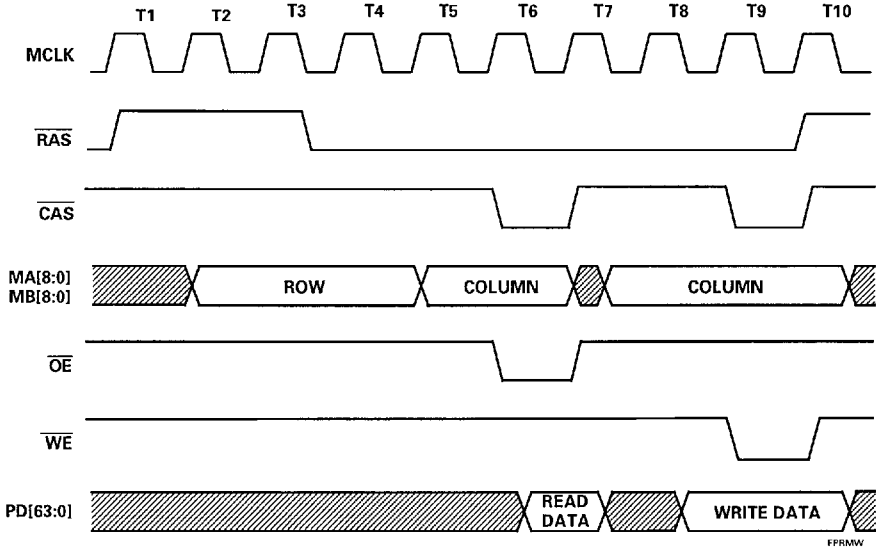
Figure 3-3. Fast Page Mode Read/Modify Write Timing
