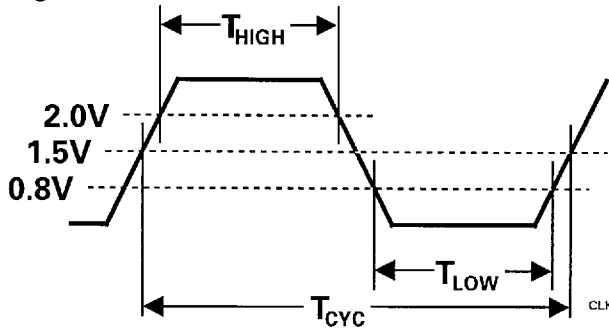
Figure 4-1. Clock Waveform Timing
