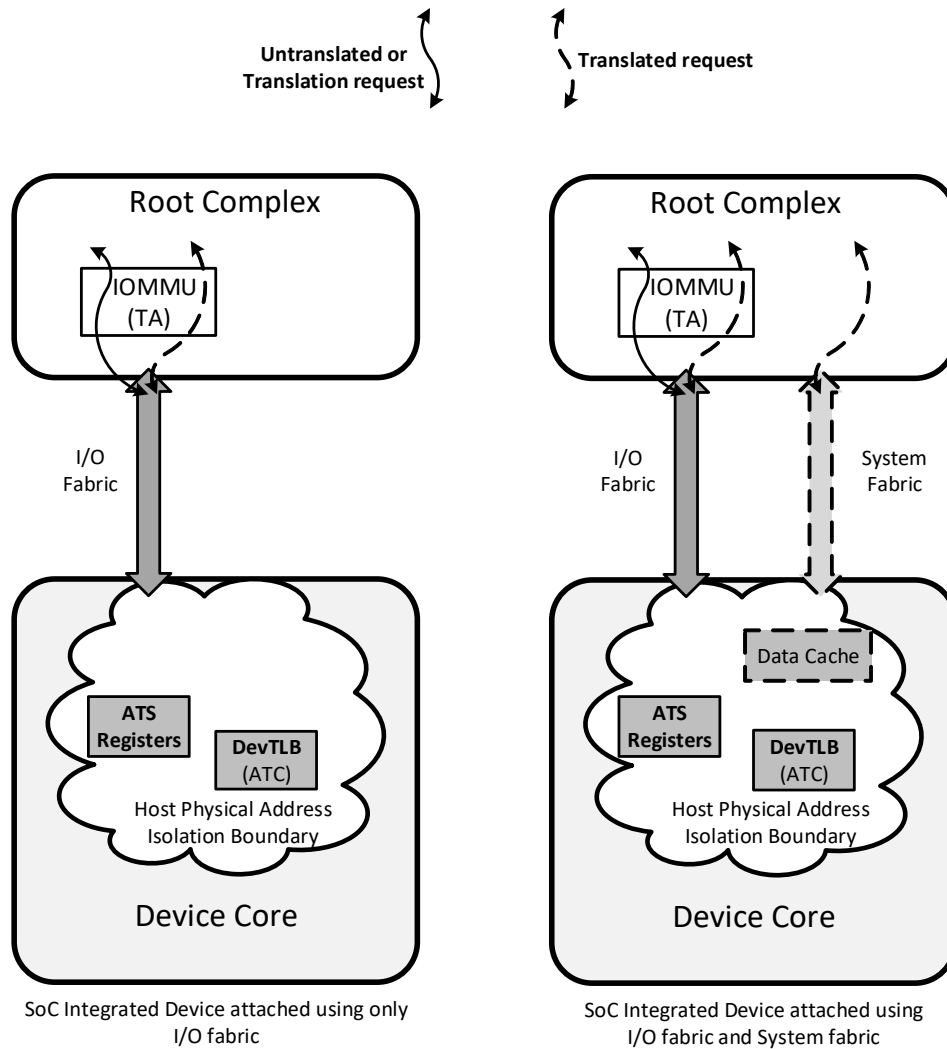
Figure 4-2. DevTLB in SoC Integrated Devices
