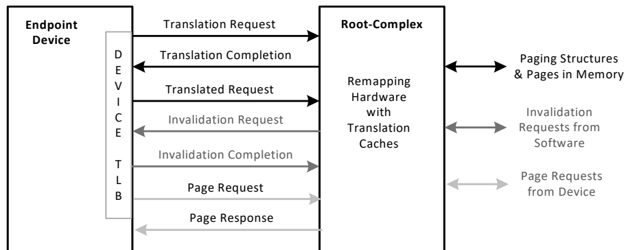
Figure 4-1. Device-TLB Operation
