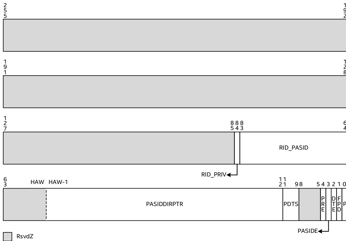
Figure 9-4. Scalable-Mode Context-Entry Format
