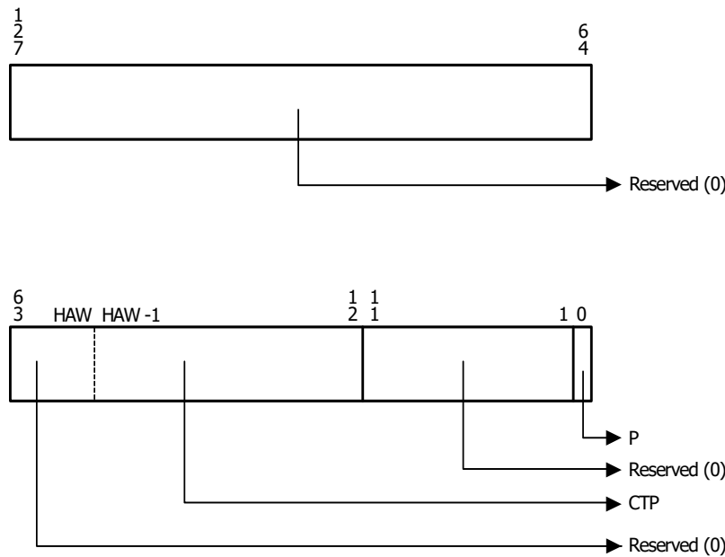
Figure 9-31. Root-Entry Format
