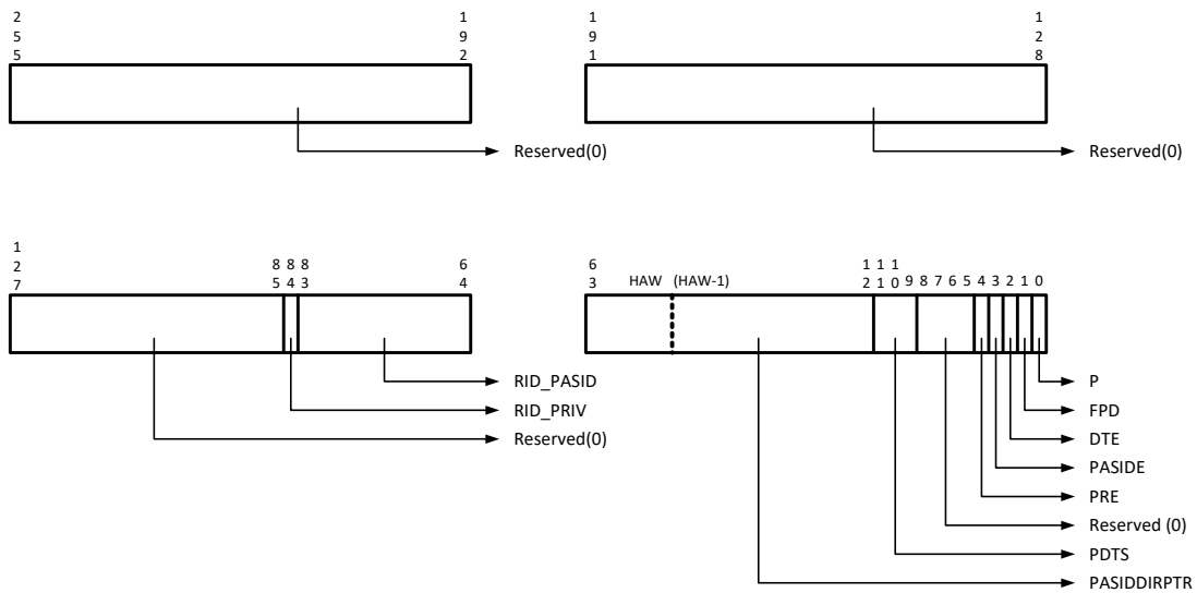
Figure 9-34. Scalable-Mode Context-Entry Format
