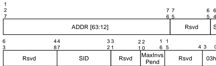
Figure 6-26. Device-TLB Invalidate Descriptor
