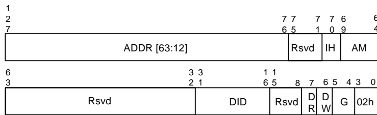
Figure 6-24. IOTLB Invalidate Descriptor
