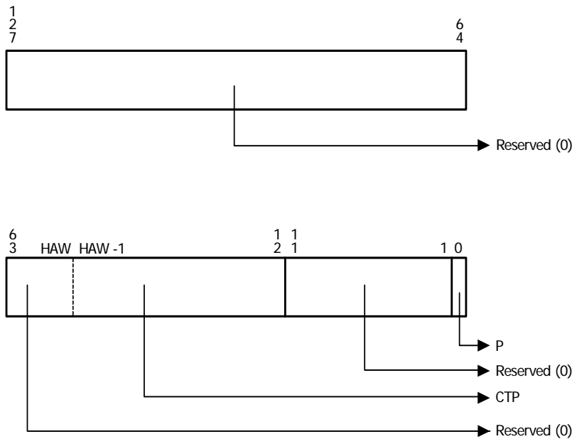
Figure 9-34. Root-Entry Format
