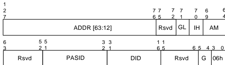
Figure 6-25. Extended IOTLB Invalidate Descriptor
