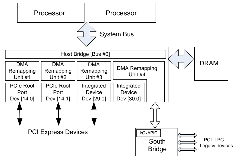
Figure 8-33. Hypothetical Platform Configuration
