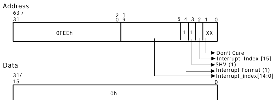
Figure 5-18. MSI-X Programming
