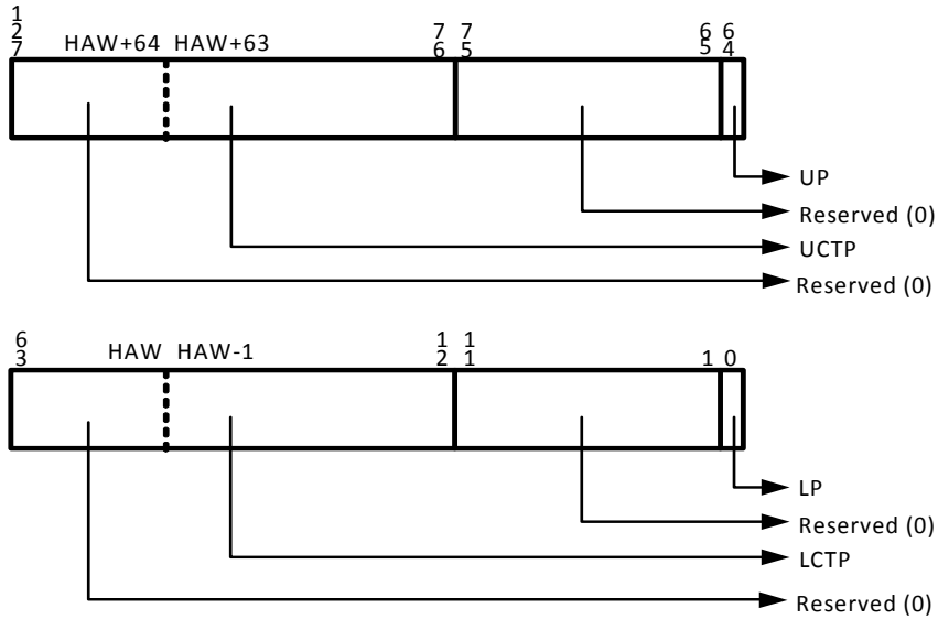
Figure 9-35. Extended-Root-Entry Format
