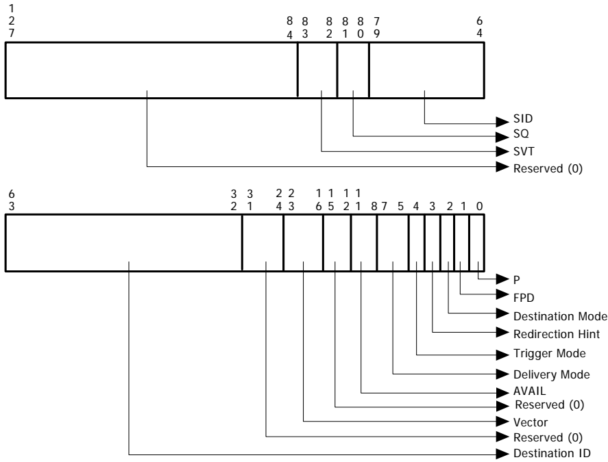
Figure 9-43. Interrupt Remapping Table Entry Format
