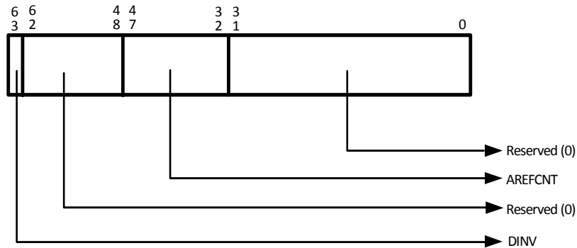
Figure 9-39. PASID-State Entry Format
