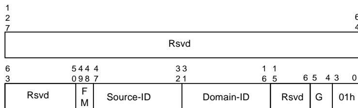
Figure 6-22. Context-cache Invalidate Descriptor
