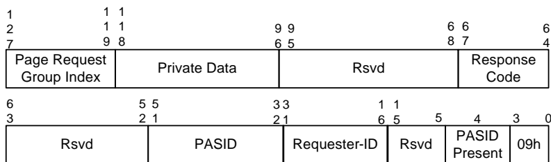
Figure 7-31. Page Group Response Descriptor
