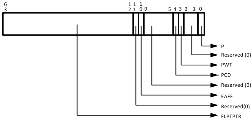
Figure 9-38. PASID Entry Format
