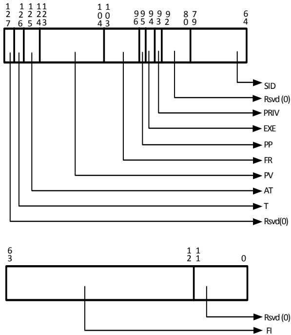
Figure 9-42. Fault-Record Format
