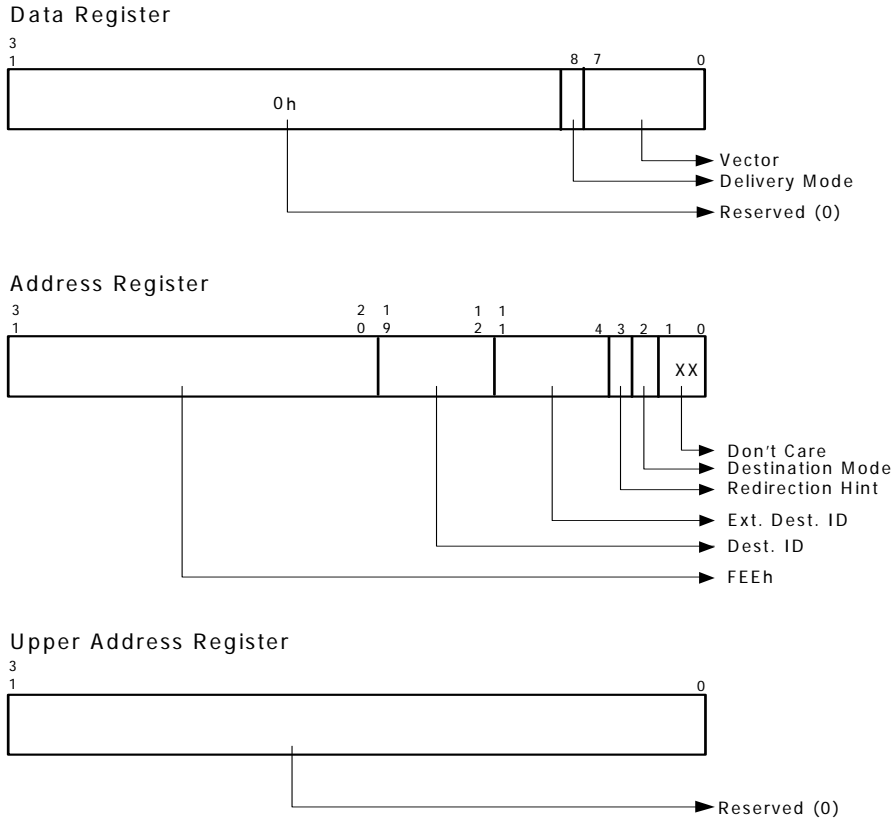
Figure 5-21. Remapping Hardware Interrupt Programming on Itanium®
