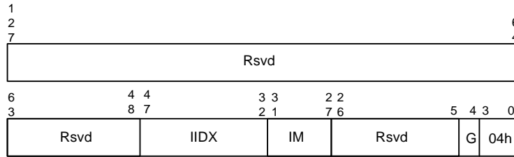
Figure 6-28. Interrupt Entry Cache Invalidate Descriptor
