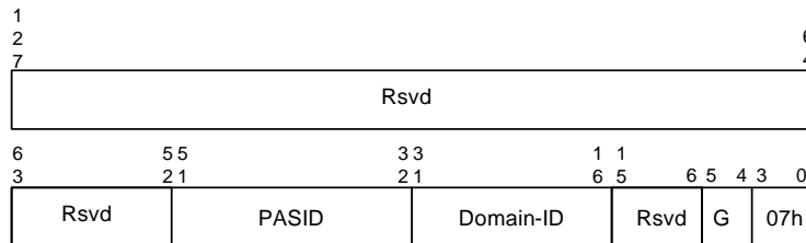
Figure 6-23. PASID-cache Invalidate Descriptor
