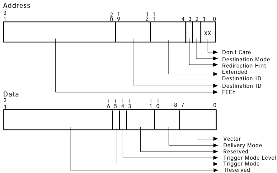
Figure 5-16. Interrupt Requests on Itanium® Platforms
