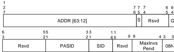
Figure 6-27. Extended Device-TLB Invalidate Descriptor
