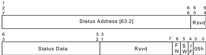
Figure 6-29. Invalidation Wait Descriptor
