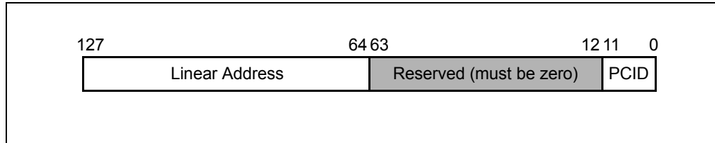
Figure 3-23. INVPCID Descriptor
