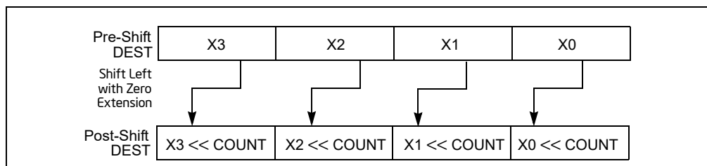
Figure 4-17. PSSLW, PSLLD, and PSLQ Instruction Operation Using 64-bit Operand
