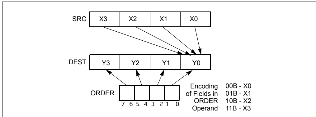
Figure 4-8. PSHUFD Instruction Operation
