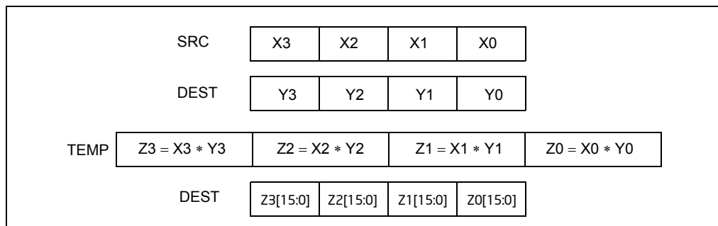
Figure 4-5. PMULLU Instruction Operation Using 64-bit Operands
