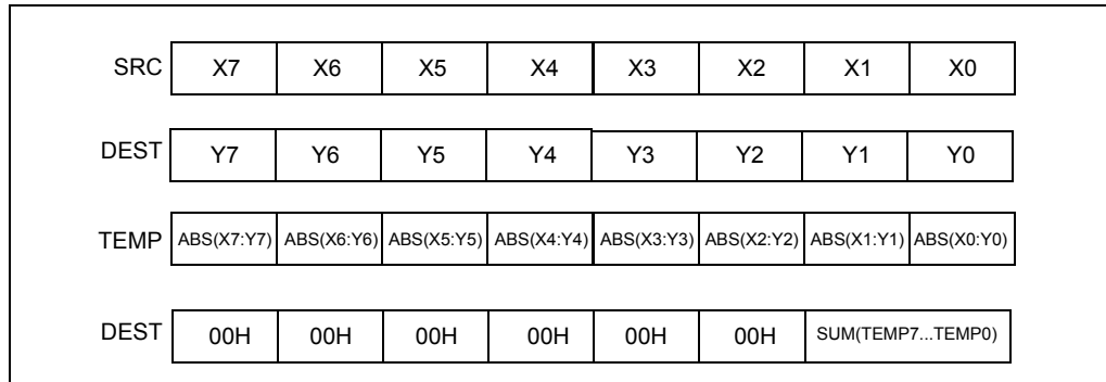
Figure 4-6. PSADBw Instruction Operation Using 64-bit Operands
