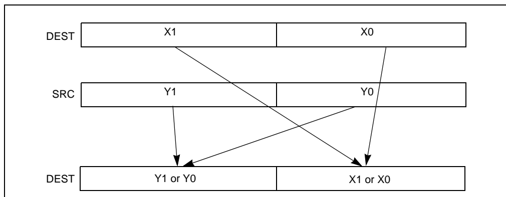
Figure 4-14. SHUFPD Shuffle Operation
