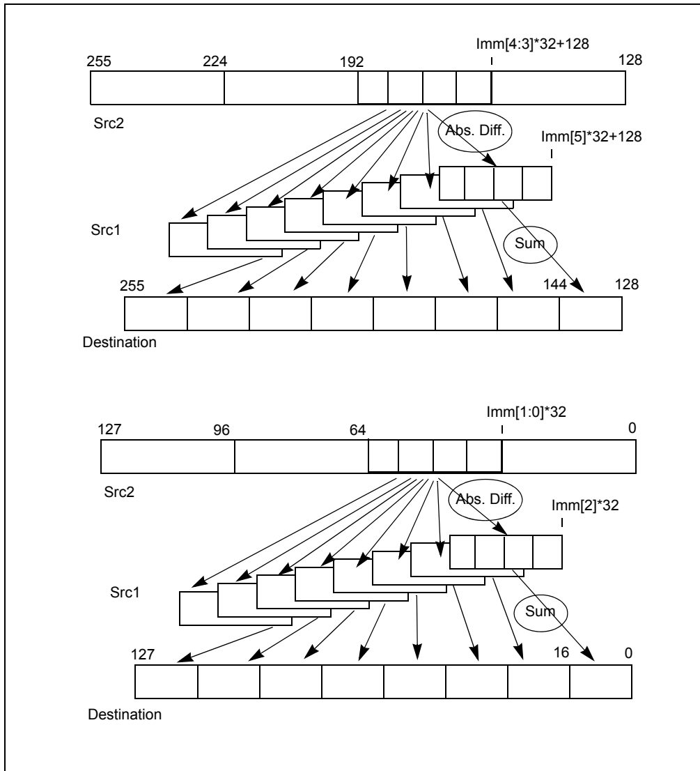
Figure 3-27. VMPSADBW Operation
