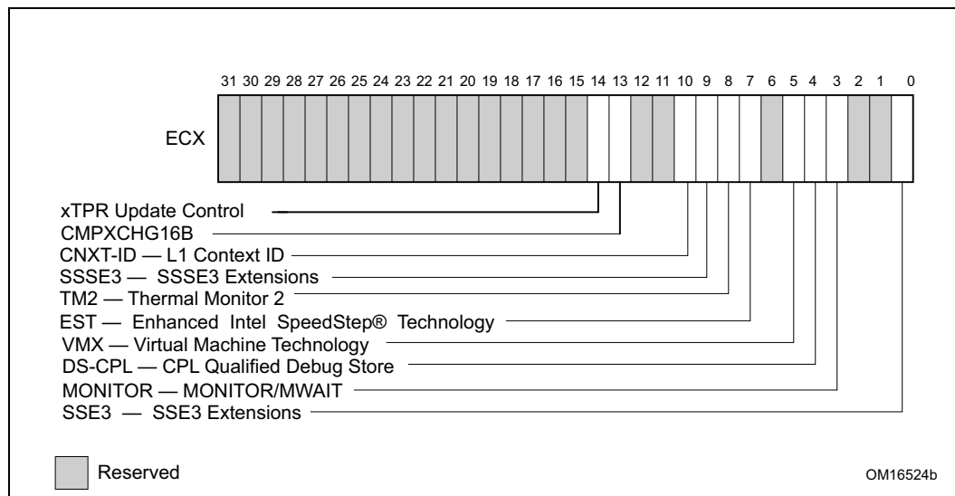
Figure 3-6. Extended Feature Information Returned in the ECX Register
