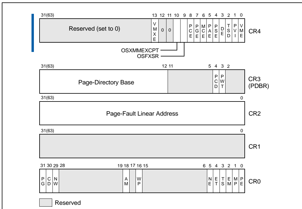
Figure 2-14. Control Registers
