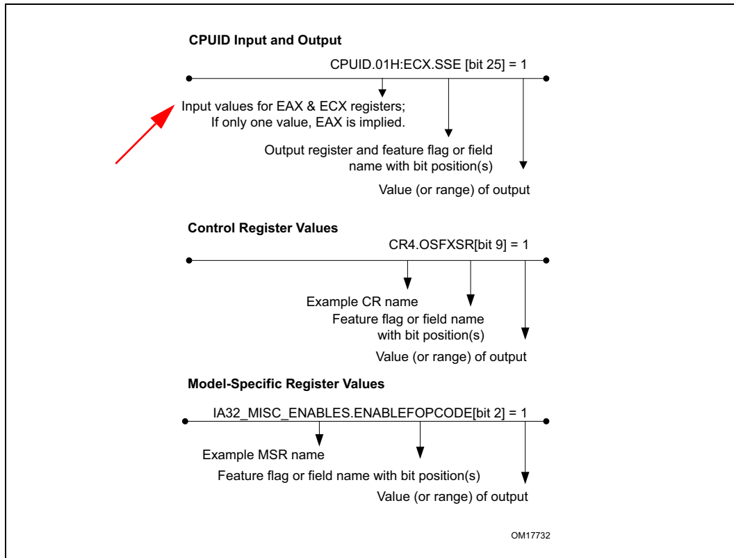
Figure 18-11. Syntax for CPUID, CR, and MSR Data Presentation
