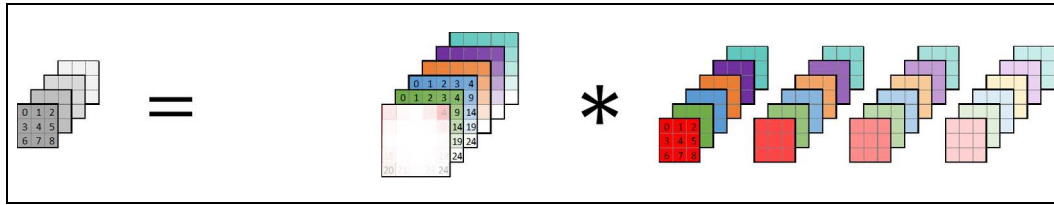
Figure 8-4. Convolution Operation
