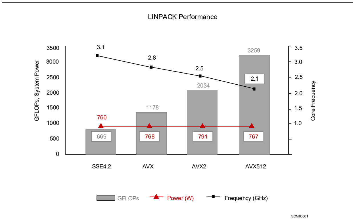
Figure 2-7. LINPACK Performance
