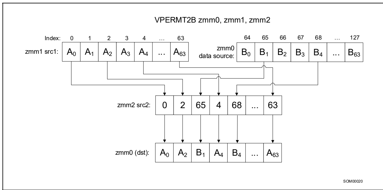
Figure 18-17. VPERMT2B Instruction Operation
