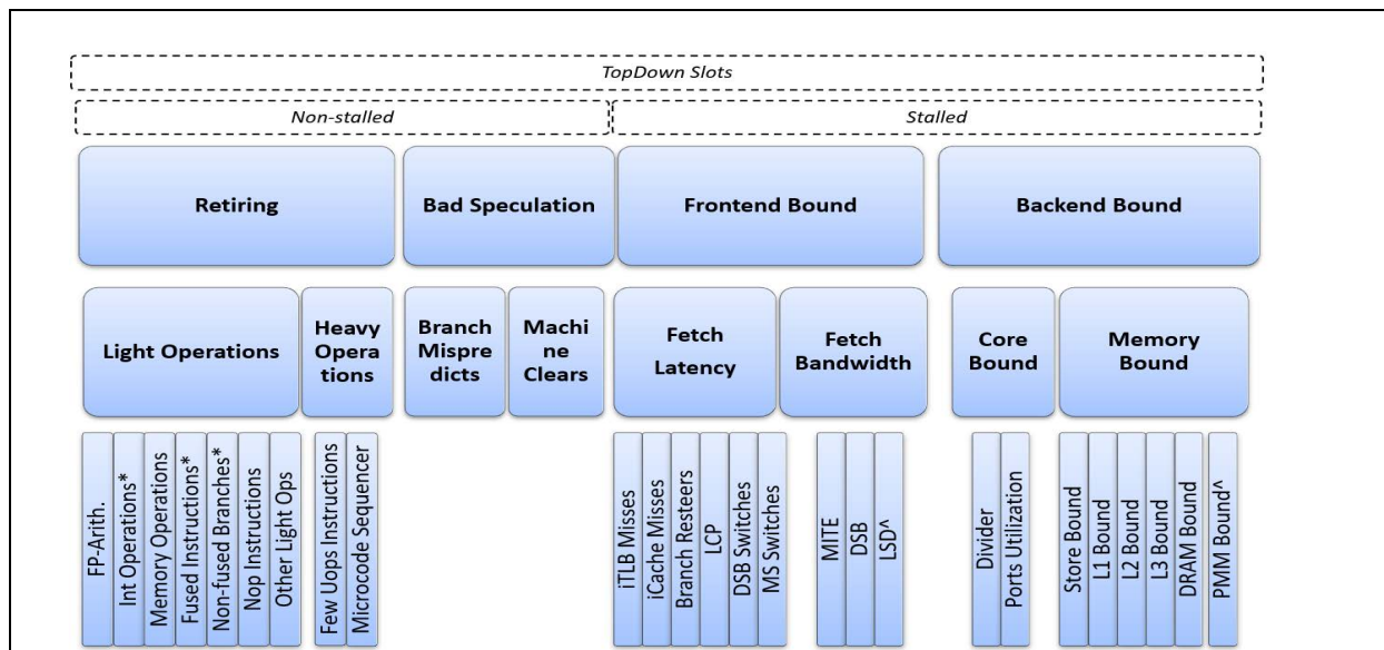
Figure B-1. General TMA Hierarchy for Out-of-Order Microarchitectures
