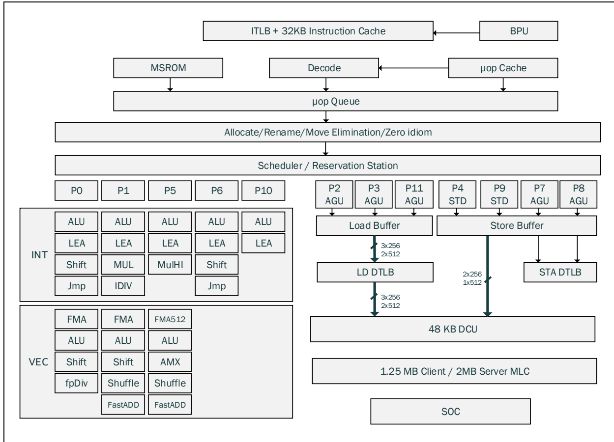
Figure 2-1. Processor Core Pipeline Functionality of the Golden Cove Microarchitecture
