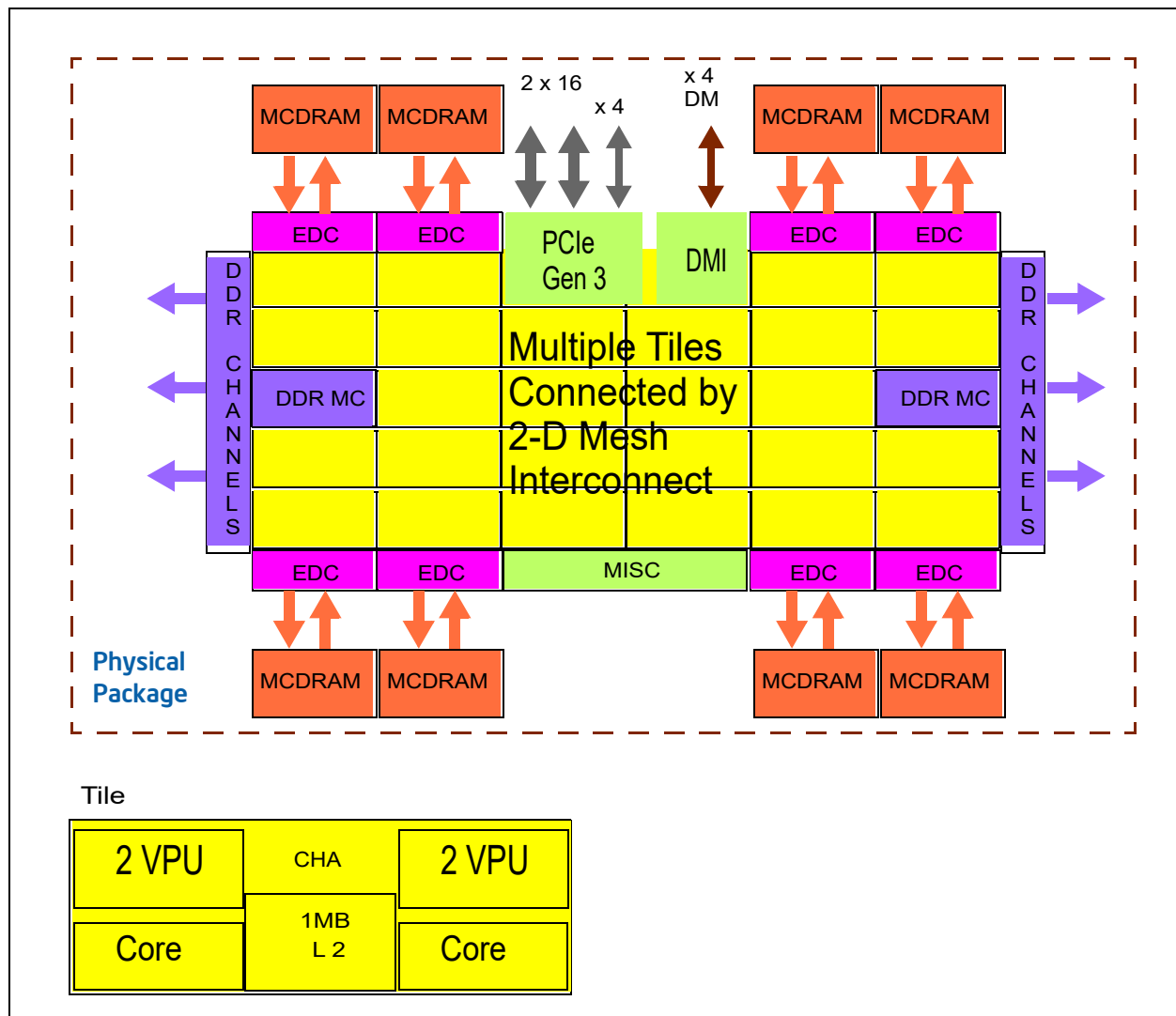
Figure 23-1. Tile-Mesh Topology of the Knights Landing Microarchitecture
