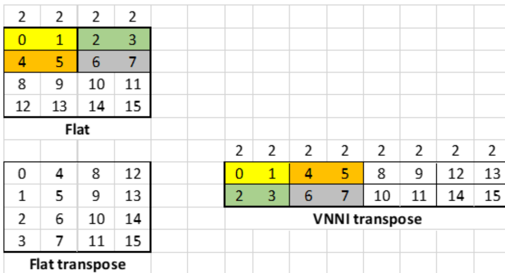
Figure 20-18. Flat-to-VNNI transpose of WORDs is equivalent to Flat-to-Flat transpose of DWORDs
