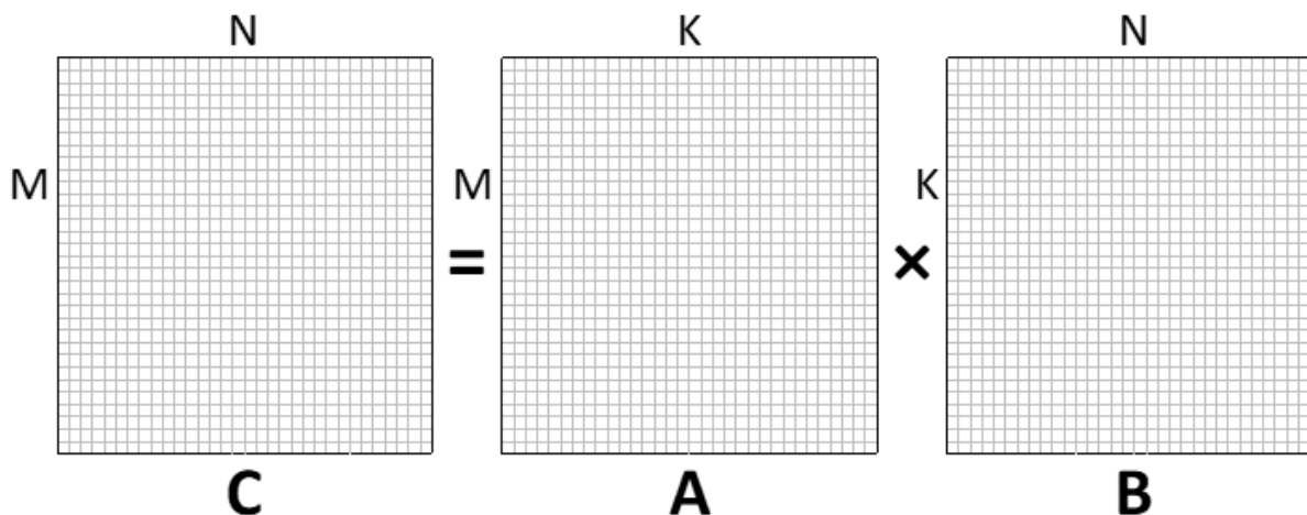
Figure 20-1. Matrix Notation
