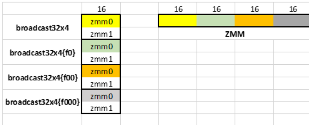
Figure 20-17. The Implementation of loading eight quarter-cache lines into two ZMM registers
