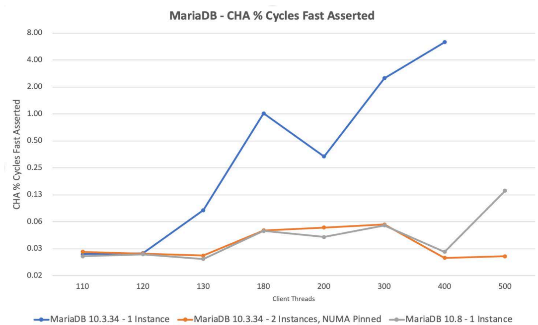
Figure 3-3. MariaDB - CHA % Cycles Fast Asserted
