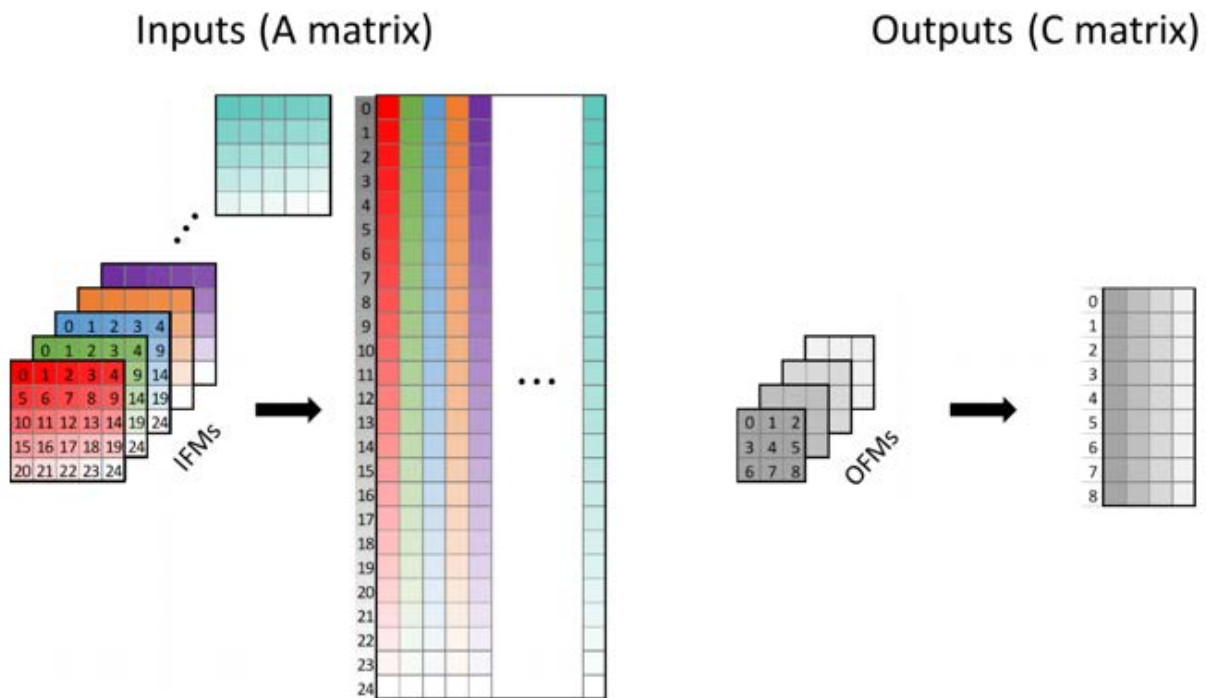
Figure 20-5. Activations layout
