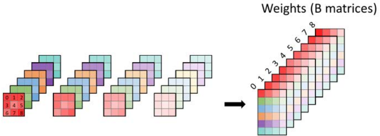
Figure 20-6. Weights Re-Layout
