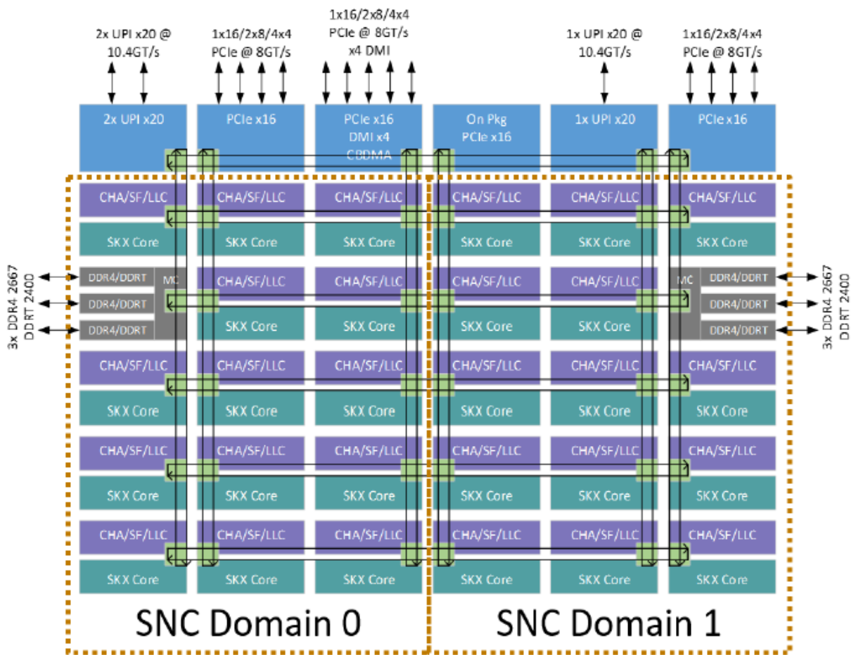
Figure 10-1. Example of SNC Configuration
