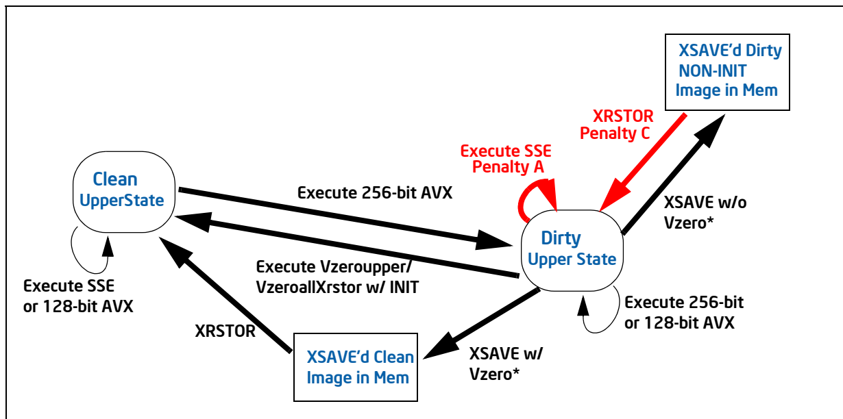
Figure 15-2. AVX-SSE Transitions in the Skylake Microarchitecture
