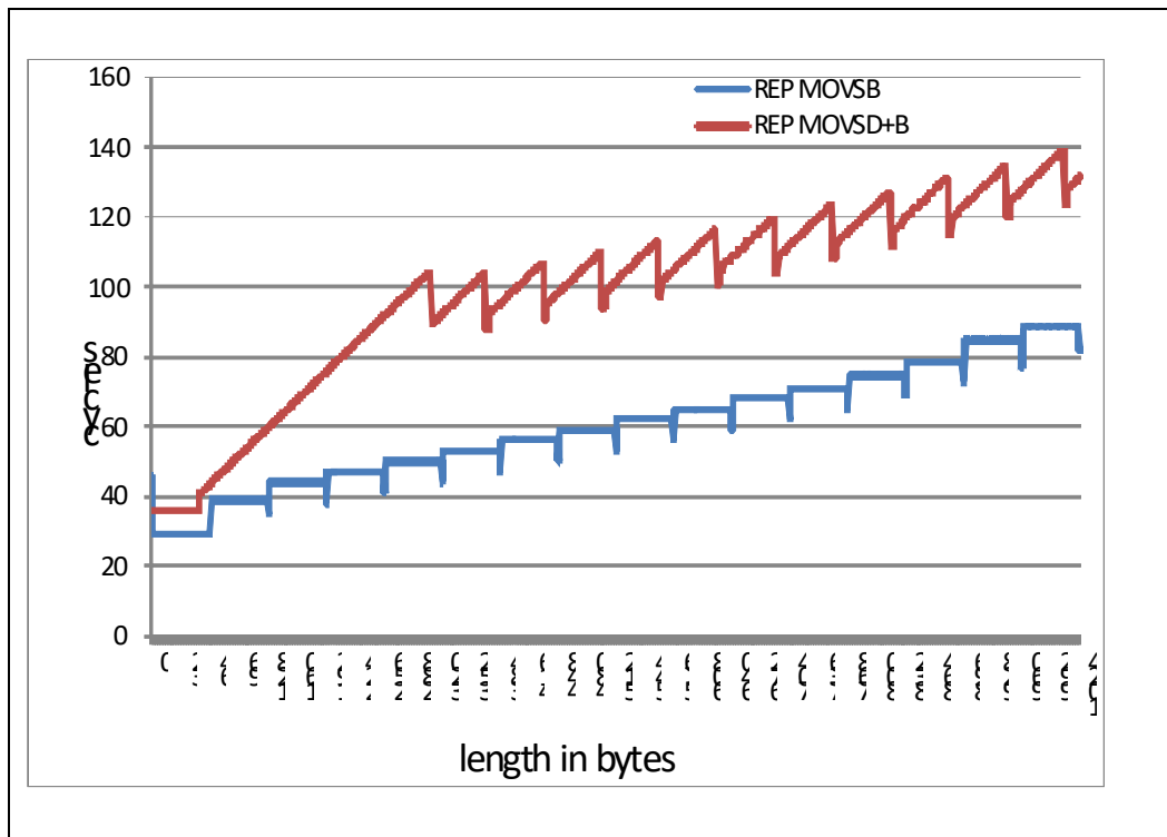
Figure 3-2. Memcpy Performance Comparison for Lengths up to 2KB
