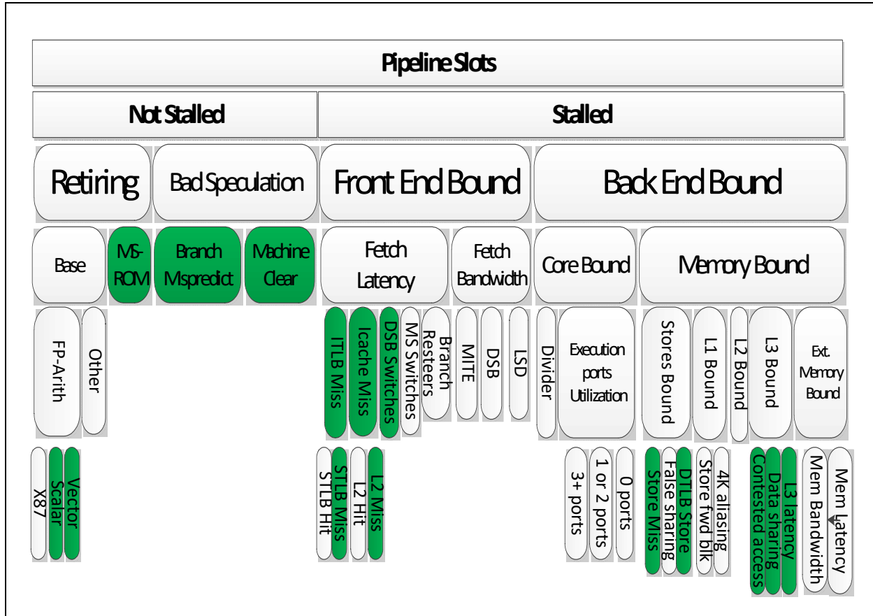
Figure B-3. TMA Hierarchy and Precise Events in Skylake
