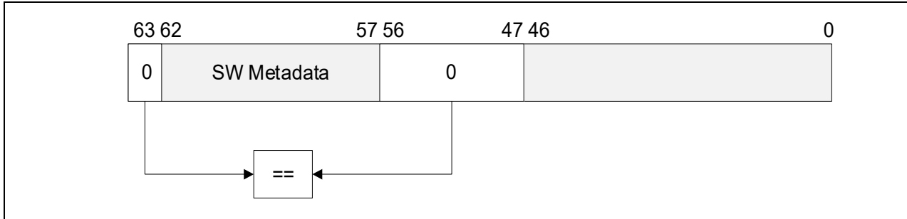
Figure 10-3. Canonicity Check When LAM57 is Enabled for User Pointers with 4-Level Paging
