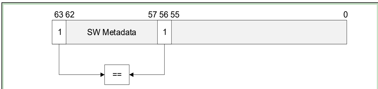
Figure 14-4. Canonality Check When LAM57 is Enabled for Supervisor Pointers with 5-Level Paging
