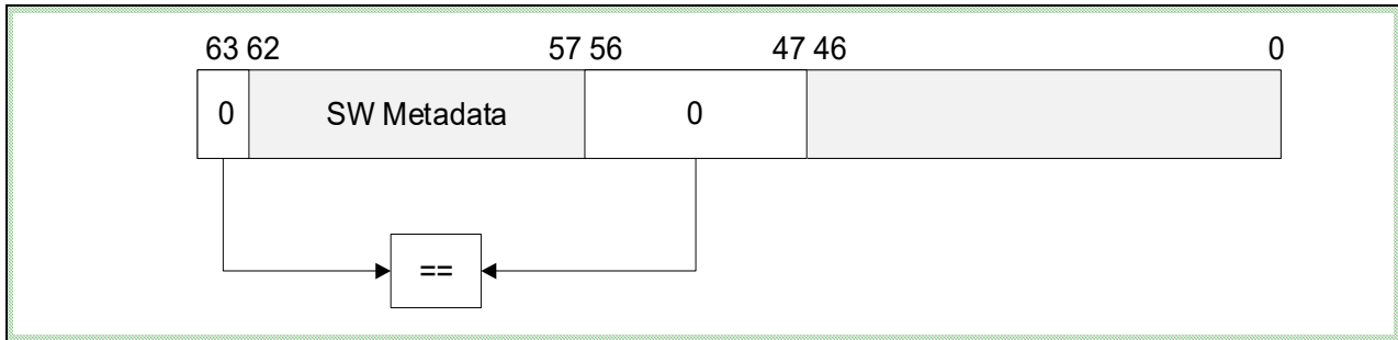
Figure 14-3. Canonality Check When LAM57 is Enabled for User Pointers with 4-Level Paging
