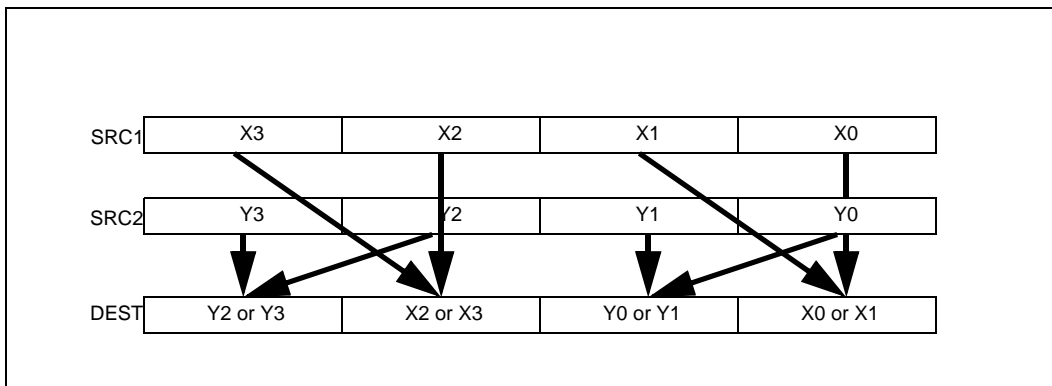
Figure 5-37. VSHUFPD Operation
