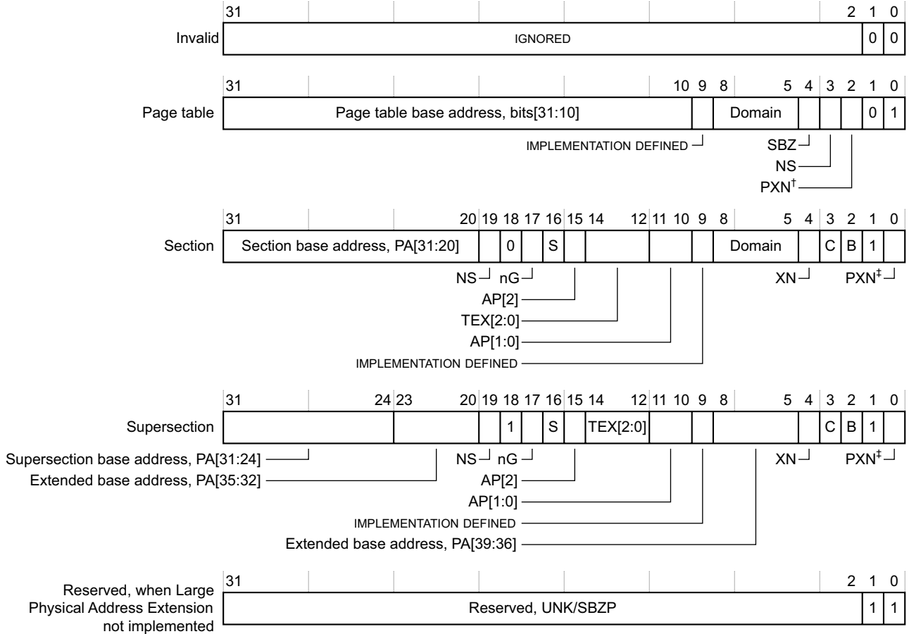
Figure B3-4 Short-descriptor first-level descriptor formats
