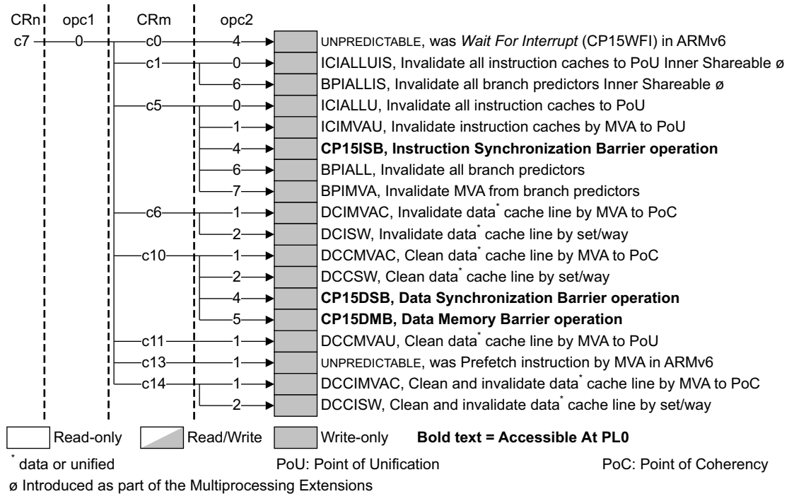
Figure B5-7 CP15 c7 registers in a PMSA implementation
