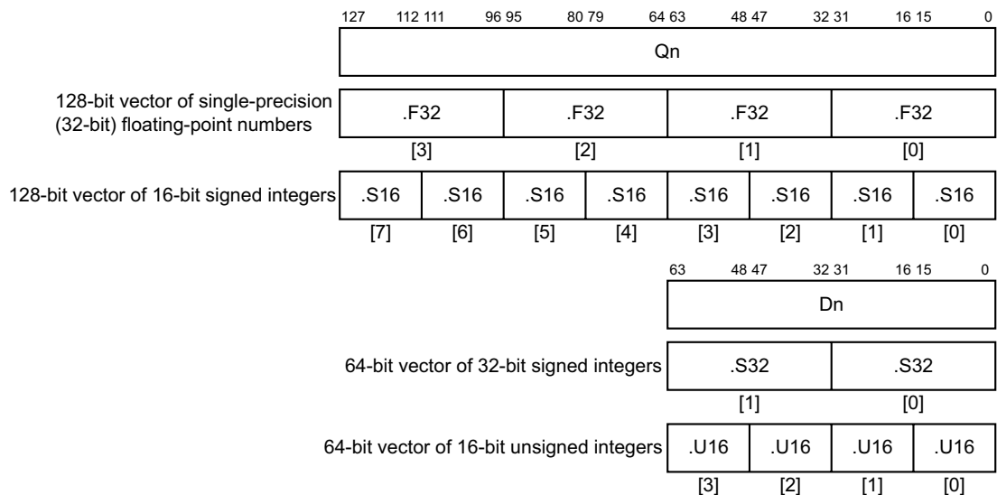
Figure A2-3 Examples of Advanced SIMD vectors
