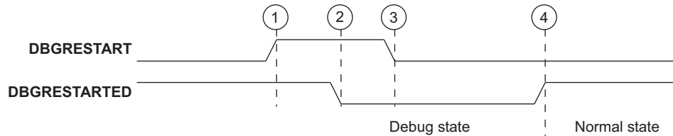
Figure A-2 DBGRESTART / DBGRESTARTED handshake
