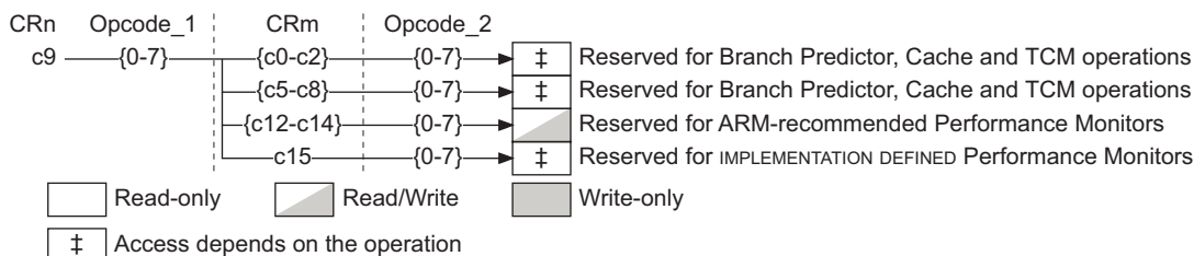
Figure B4-12 Permitted CP15 c9 register encodings
