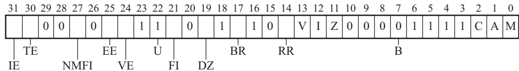
Figure B4-6 SCTLR format, ARMv7-R (PMSAv7)
