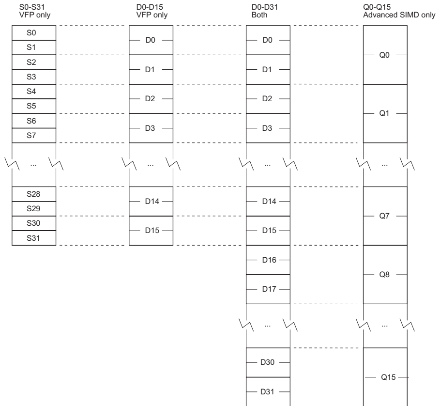
Figure A2-1 Advanced SIMD and VFPv3 register set
