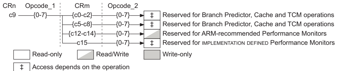
Figure B3-22 Permitted CP15 c9 encodings
