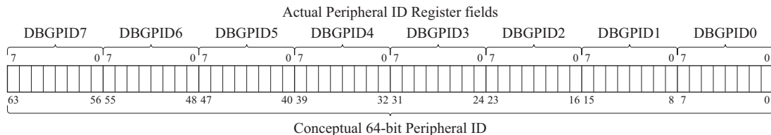
Figure C10-1 Mapping between Debug Peripheral ID Registers and a 64-bit Peripheral ID value
