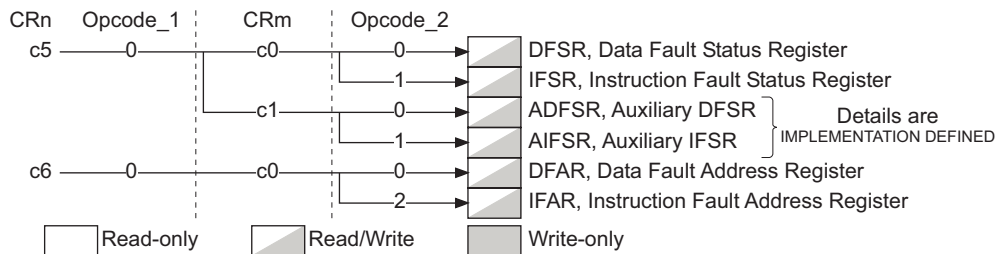
Figure B3-16 CP15 c5 and c6 registers in a VMSA implementation
