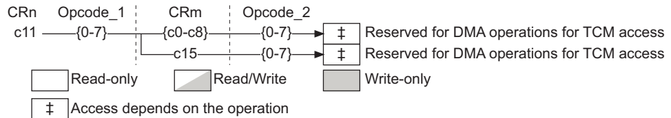
Figure B3-24 Permitted CP15 c11 encodings
