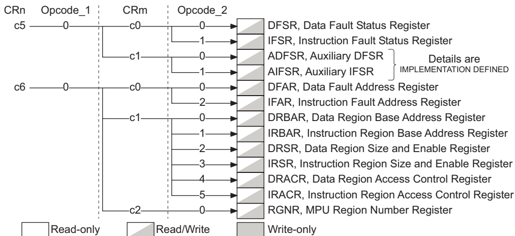
Figure B4-8 CP15 c5 and c6 registers in a PMSA implementation
