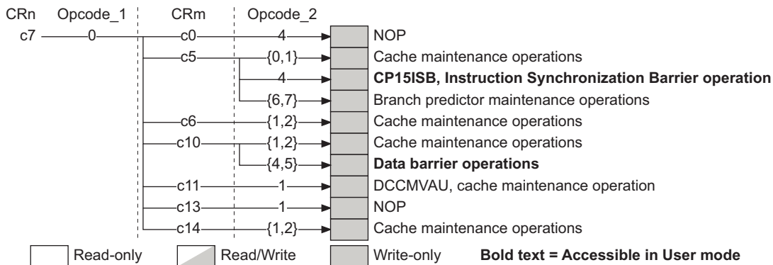
Figure B4-9 CP15 c7 registers in a PMSA implementation
