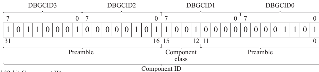
Figure C10-3 Mapping between Debug Component ID Registers and the 32-bit Component ID value
