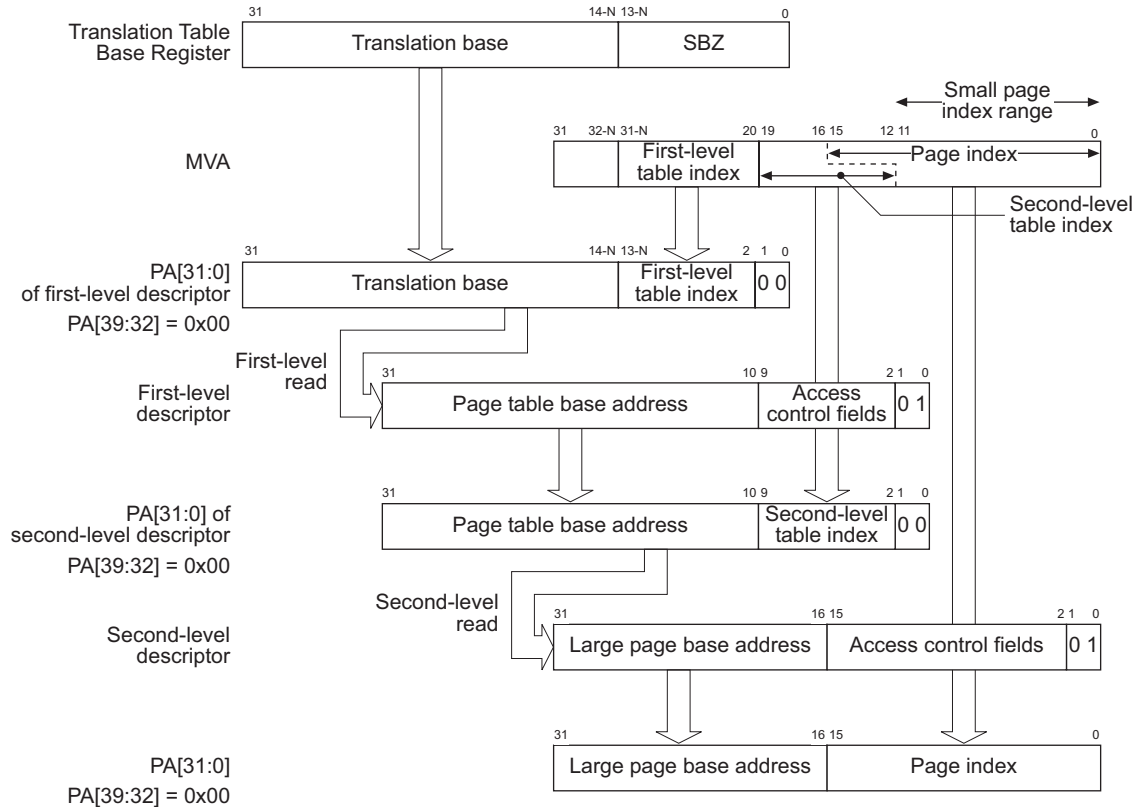
Figure B3-7 Large page address translation
