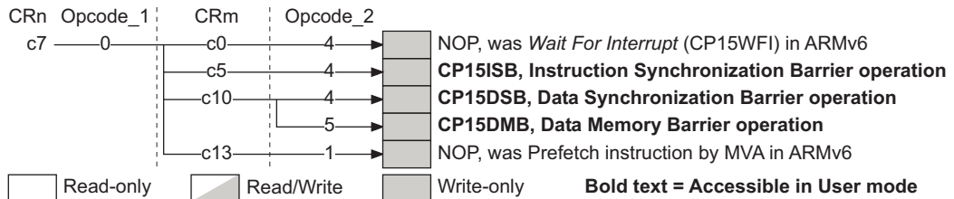
Figure B4-11 c7 Miscellaneous operations
