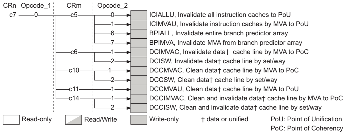
Figure B3-18 CP15 c7 Cache and branch predictor maintenance operations
