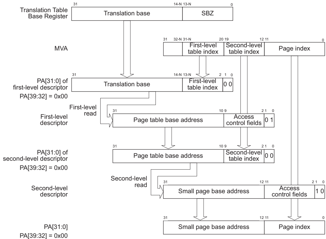
Figure B3-6 Small page address translation
