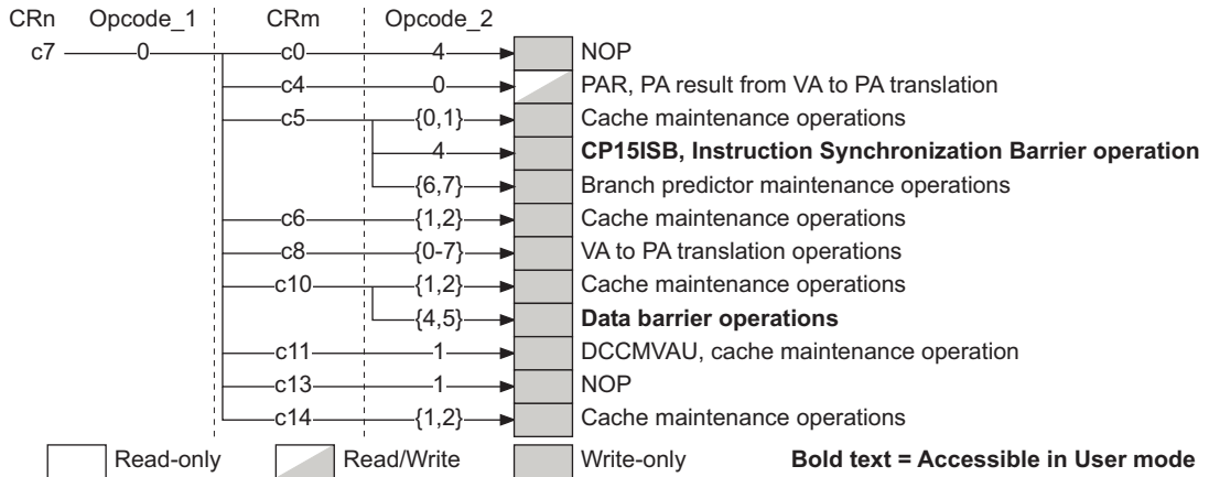
Figure B3-17 CP15 c7 registers in a VMSA implementation
