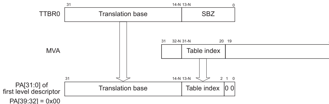
Figure B3-2 Accessing the translation table first-level descriptors based on TTBR0
