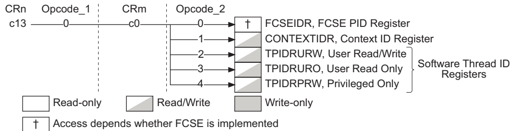
Figure B3-26 CP15 c13 registers in a VMSA implementation
