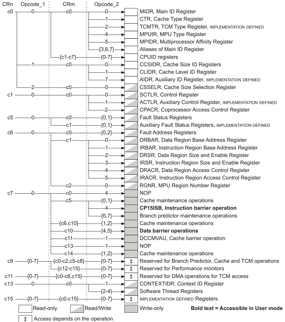
Figure B4-3 CP15 registers in a PMSA implementation
