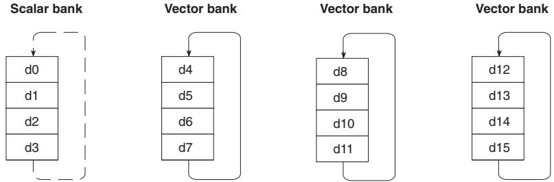
Figure F-3 Register banks, 16 double-precision register VFP
