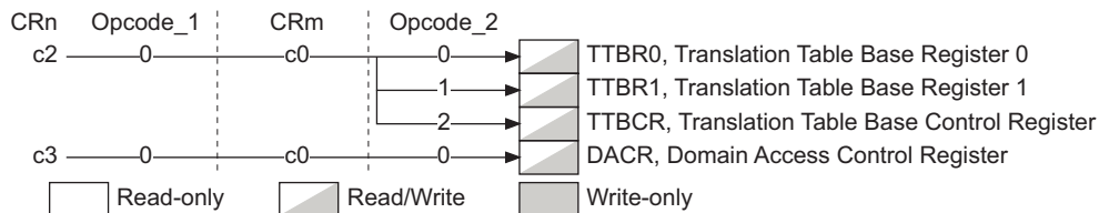
Figure B3-15 CP15 c2 and c3 registers
