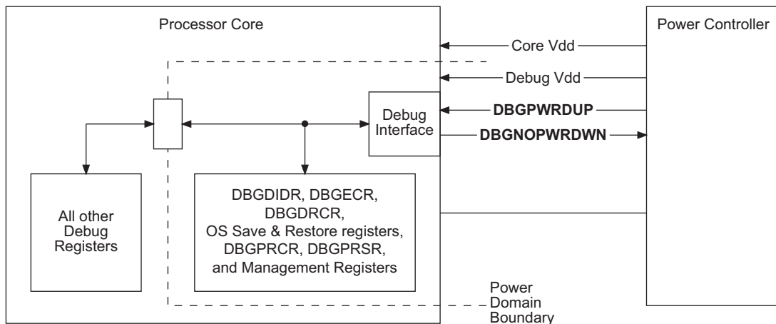
Figure C6-1 Recommendation for power domain split between core and debug
