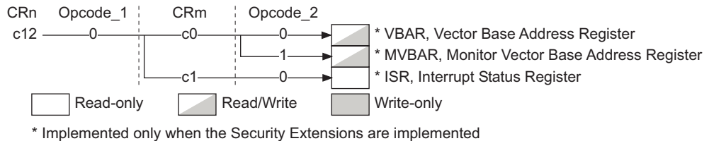
Figure B3-25 Security Extensions CP15 c12 registers
