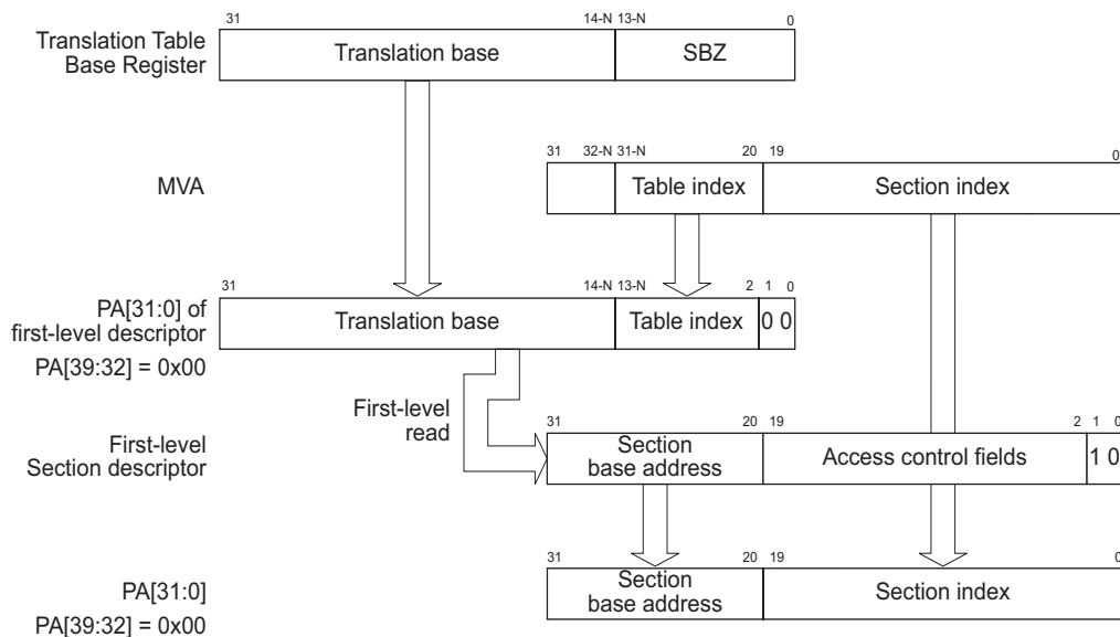
Figure B3-4 Section address translation
