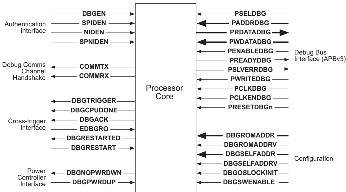
Figure A-3 Recommended external debug interface, including APBv3 slave port
