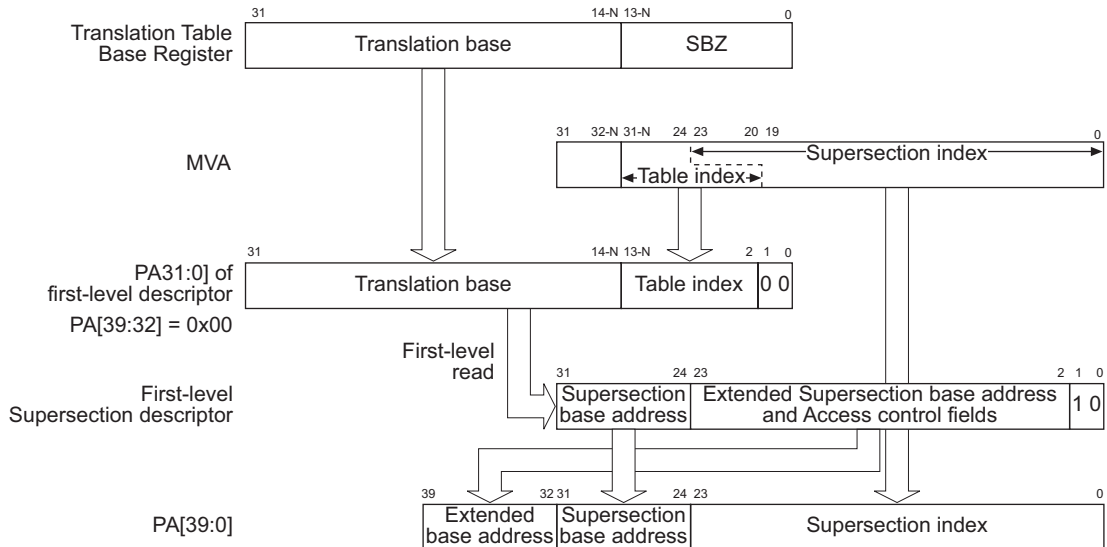
Figure B3-5 Supersection address translation
