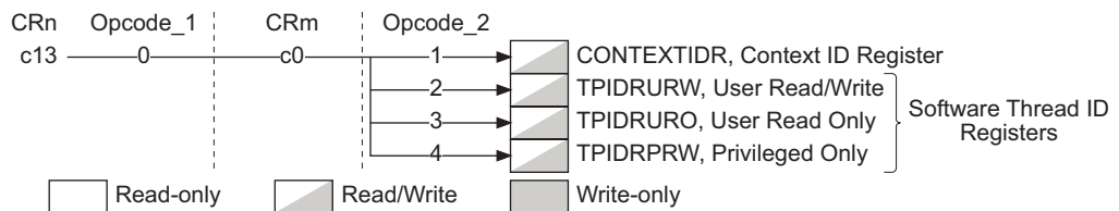
Figure B4-14 CP15 c13 registers in a PMSA implementation
