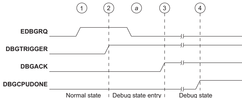
Figure A-1 External debug request handshake using DBGTRIGGER, DBGACK and DBGCPUDONE
