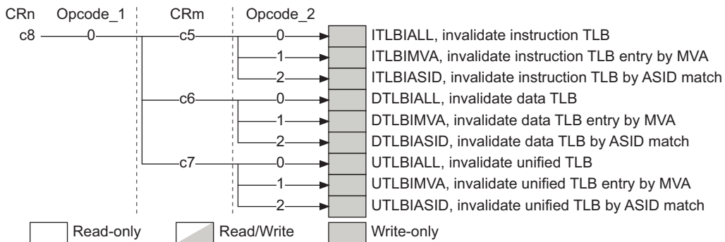
Figure B3-21 CP15 c8 operations
