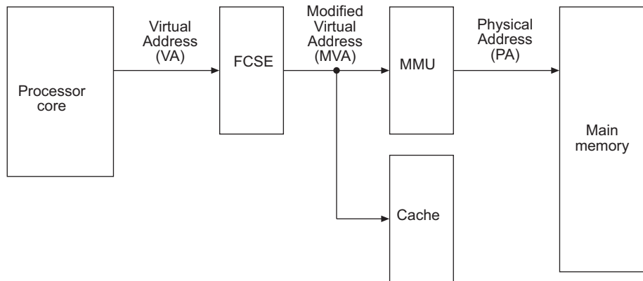
Figure E-1 Address flow in MMU memory system with FCSE
