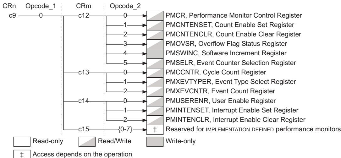
Figure C9-1 Recommended CP15 performance monitors, in register c9
