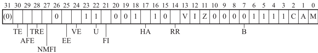
Figure B3-13 SCTLR format, ARMv7-A (VMSAv7)
