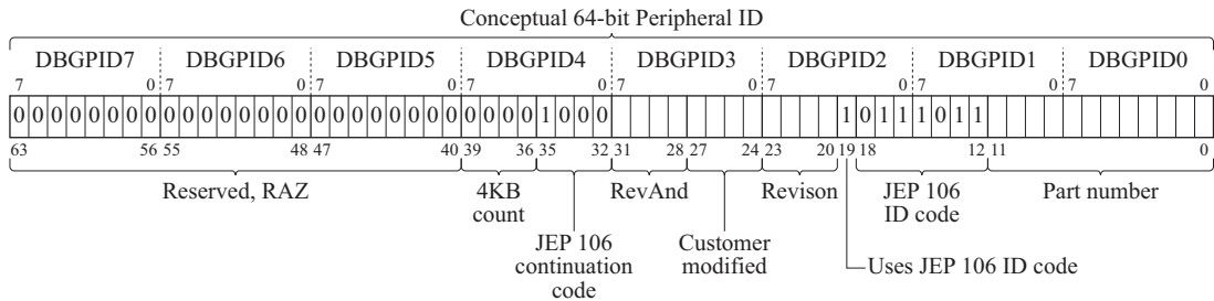
Figure C10-2 Peripheral ID fields, with values for a design by ARM Limited
