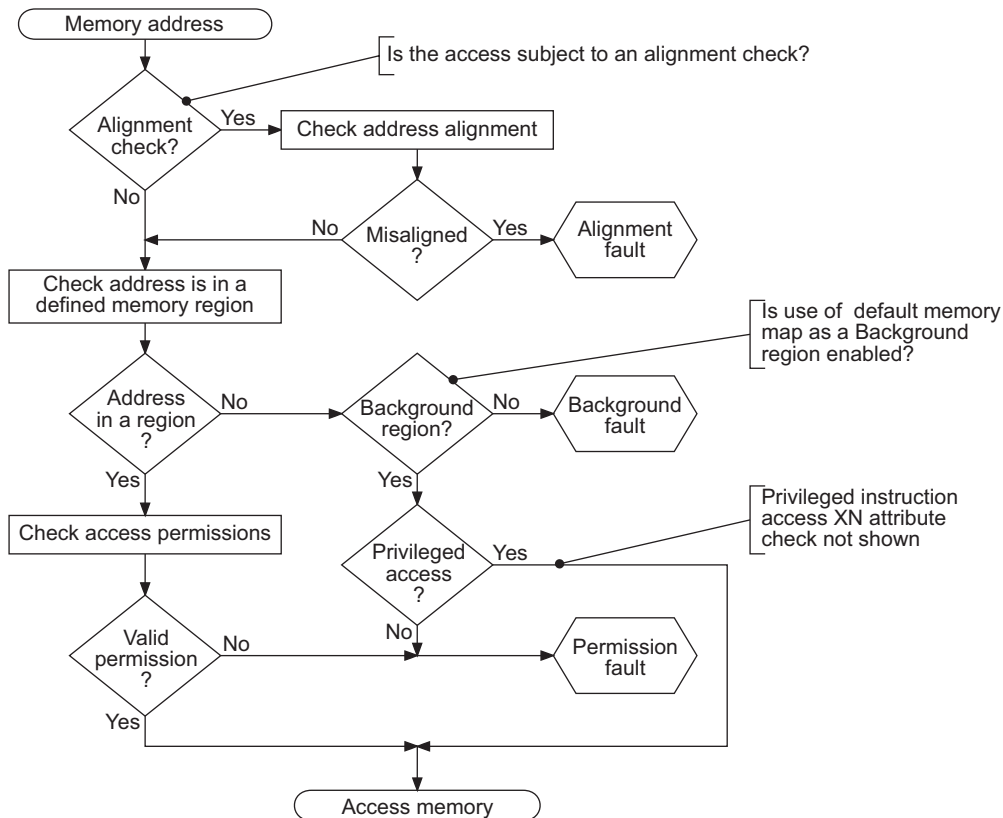
Figure B4-2 MPU fault checking sequence
