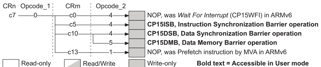
Figure B3-20 CP15 c7 Miscellaneous operations
