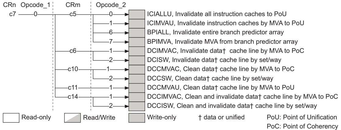
Figure B4-10 CP15 c7 Cache and branch predictor maintenance operations
