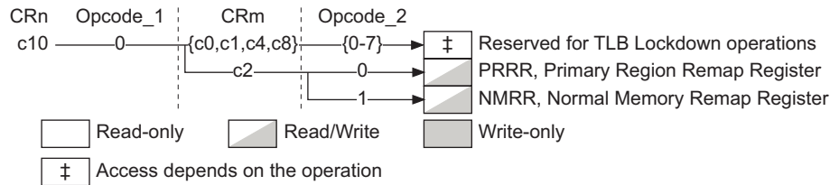
Figure B3-23 CP15 c10 registers
