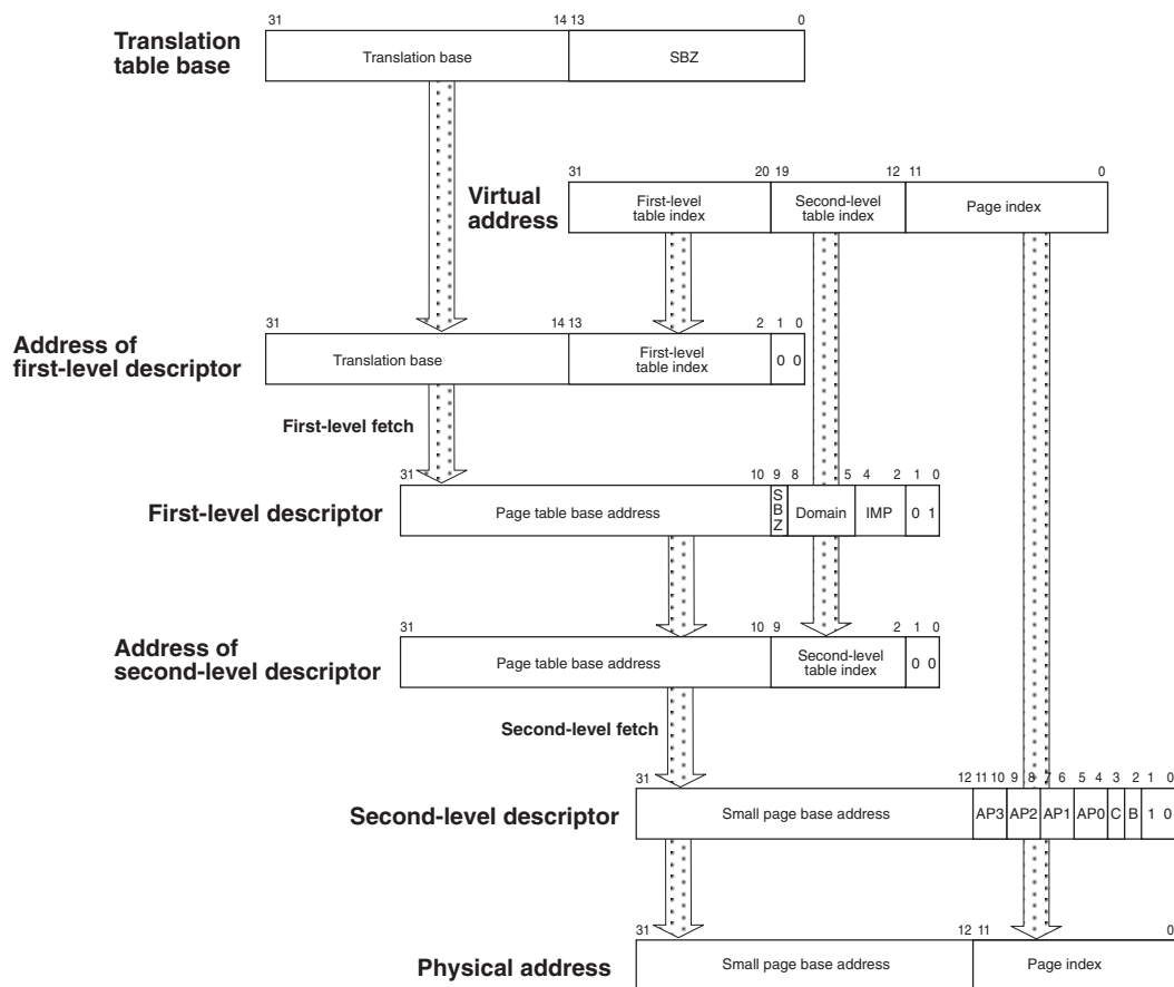
Figure 3-7 Small page translation in a coarse second-level table
