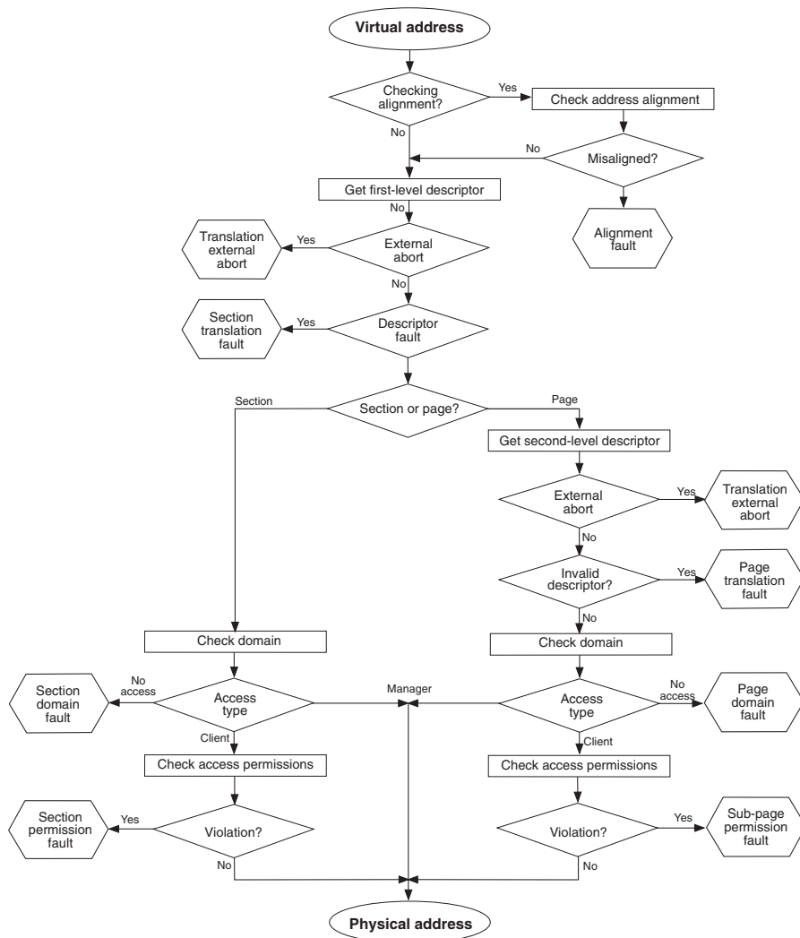
Figure 3-9 Sequence for checking faults
