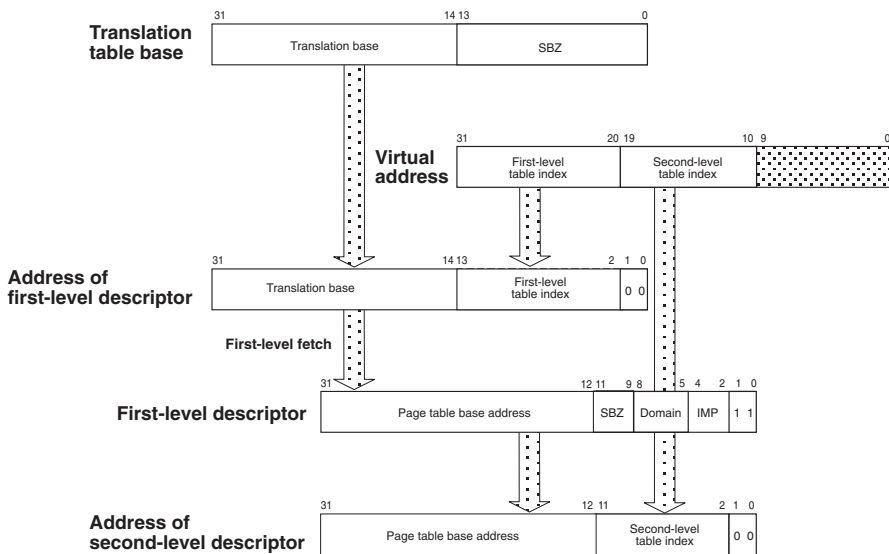
Figure 3-5 Accessing fine page table second-level descriptors
