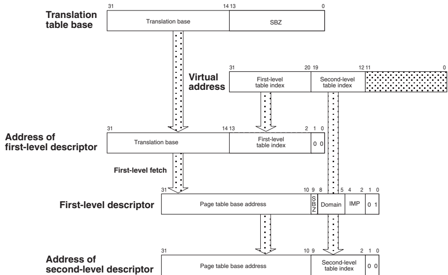
Figure 3-4 Accessing coarse page table second-level descriptors
