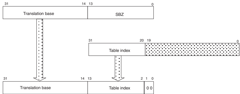
Figure 3-2 Accessing the translation table first-level descriptors
