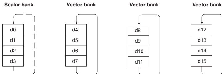
Figure 5-2 Double-precision register banks
