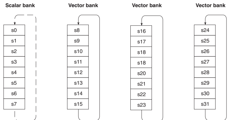
Figure 5-1 Single-precision register banks
