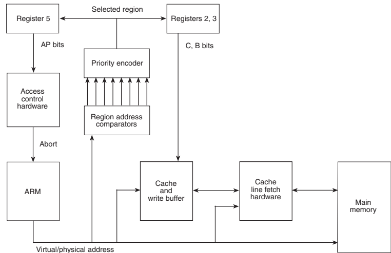
Figure 4-1 Cached Protection Unit memory system overview
