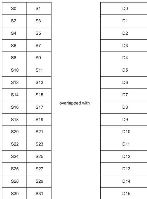
Figure 2-1 VFP general-purpose registers
