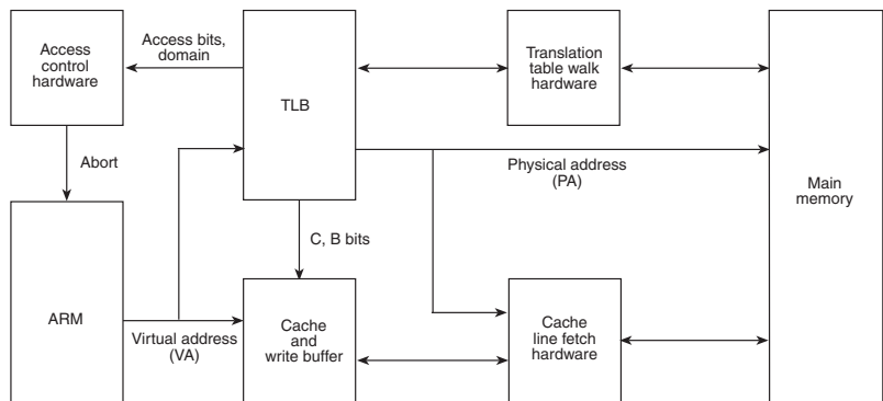
Figure 3-1 Cached MMU memory system overview
