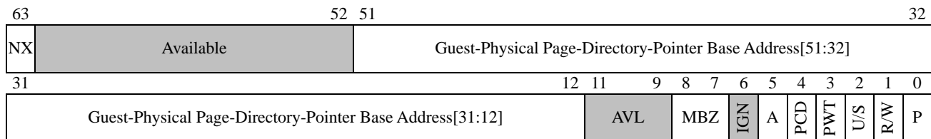
Figure 38: AMD64 Long Mode 1-Gbyte PML4E Format
