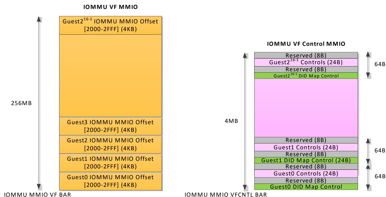
Figure 80: IOMMU Virtual Function Control MMIO and IOMMU Virtual Function MMIO
