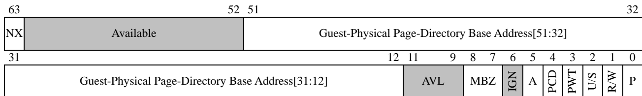
Figure 34: AMD64 Long Mode 2-Mbyte PDPE Format
