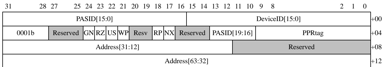
Figure 74: PAGE_SERVICE_REQUEST PPR Log Buffer Entry Format
