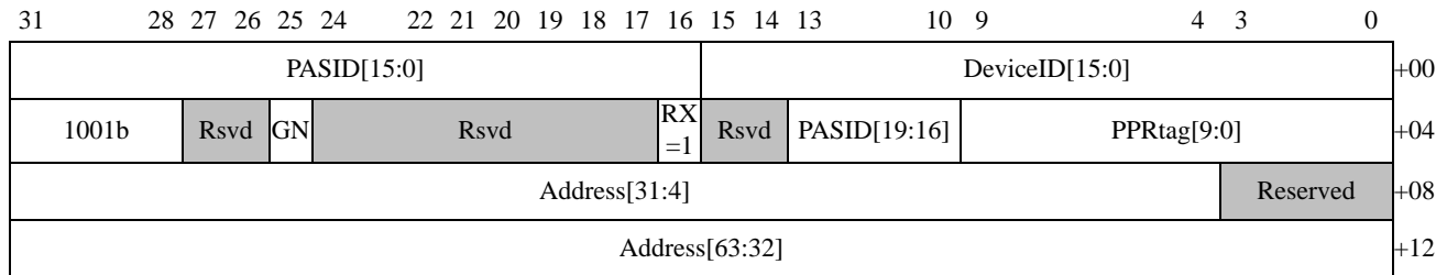
Figure 64: INVALID_PPR_REQUEST Event Log Buffer Entry Format, RX = 1
