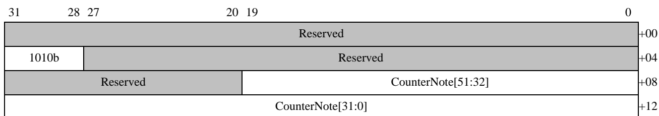
Figure 65: EVENT_COUNTER_ZERO Event Log Buffer Entry Format
