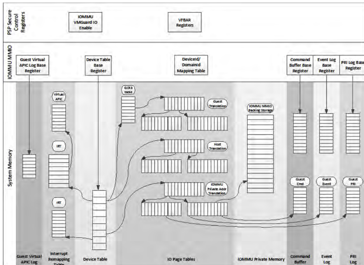
Figure 4: IOMMU Data Structures
