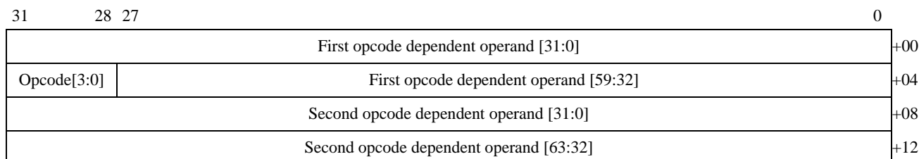
Figure 43: Generic Command Buffer Entry Format
