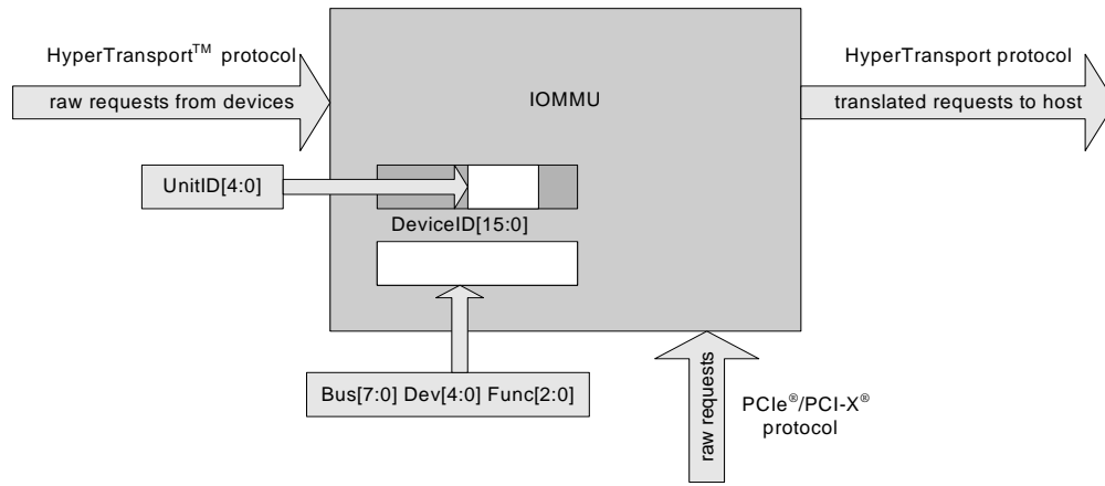
Figure 85: Hybrid IOMMU
