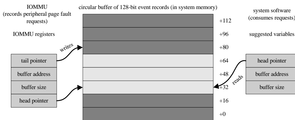
Figure 71: Peripheral Page Request Log in System Memory
