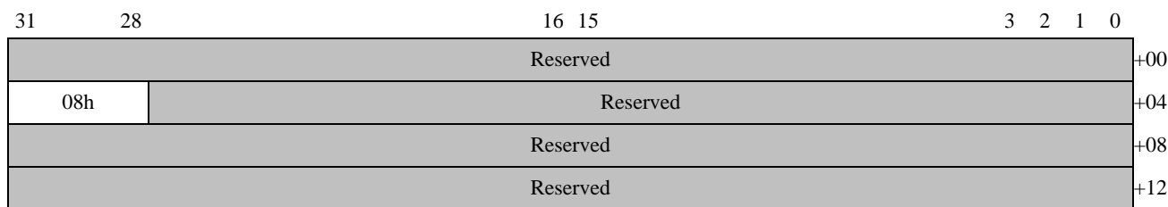
Figure 51: INVALIDATE_IOMMU_ALL Command Format
