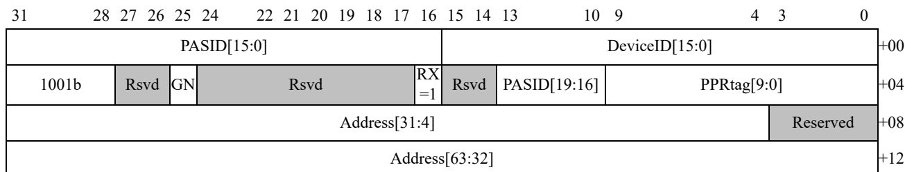
Figure 64: INVALID_PPR_REQUEST Event Log Buffer Entry Format, RX = 1
