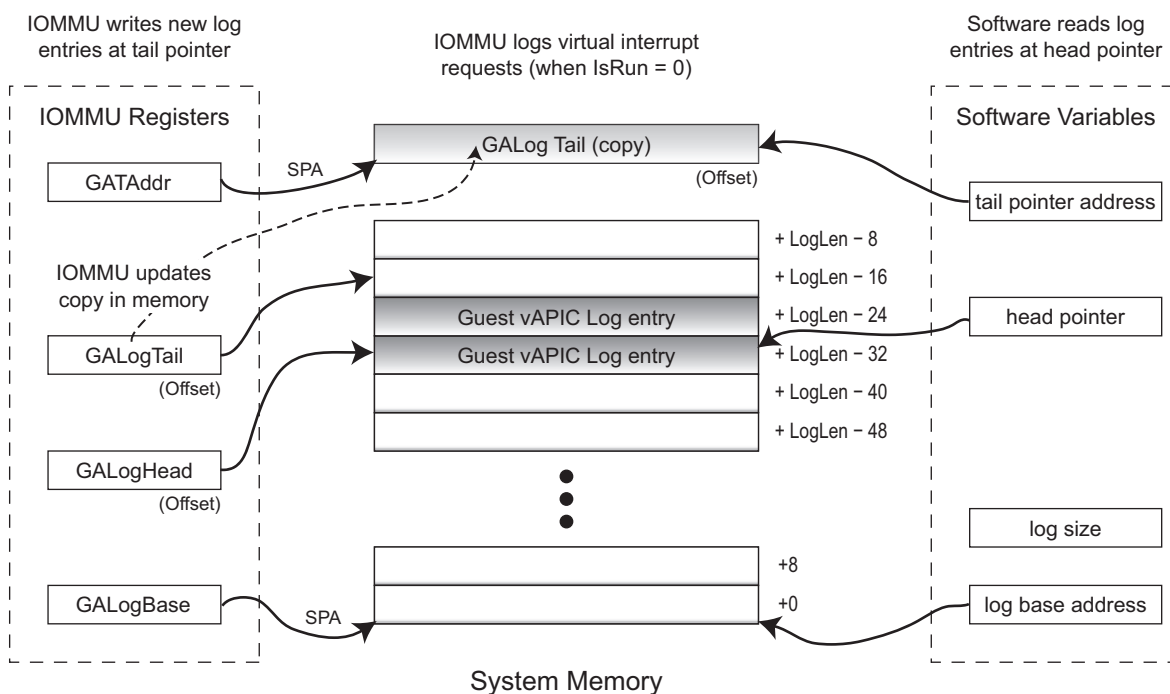
Figure 75: Guest vAPIC Log in System Memory
