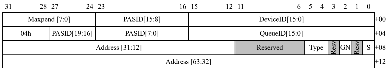
Figure 47: INVALIDATE_IOTLB_PAGES Command Format
