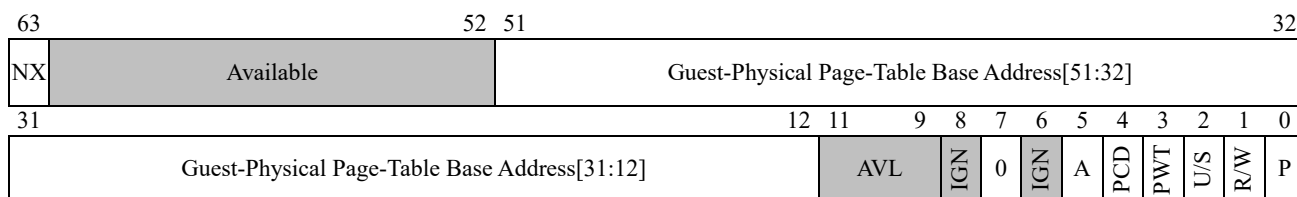
Figure 29: AMD64 Long Mode 4-Kbyte PDE Format
