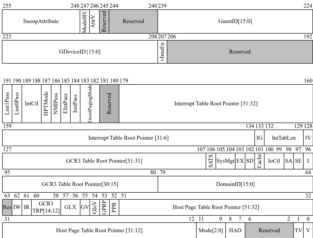
Figure 7: Device Table Entry (DTE) Fields
