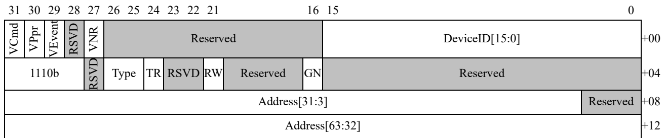
Figure 69: RMP_HARDWARE_ERROR Event Log Buffer Entry Format
