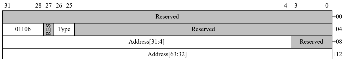
Figure 60: COMMAND_HARDWARE_ERROR Event Log Buffer Entry Format
