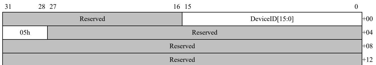
Figure 48: INVALIDATE_INTERRUPT_TABLE Command Format
