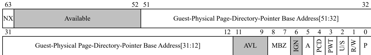
Figure 33: AMD64 Long Mode 2-Mbyte PML4E Format
