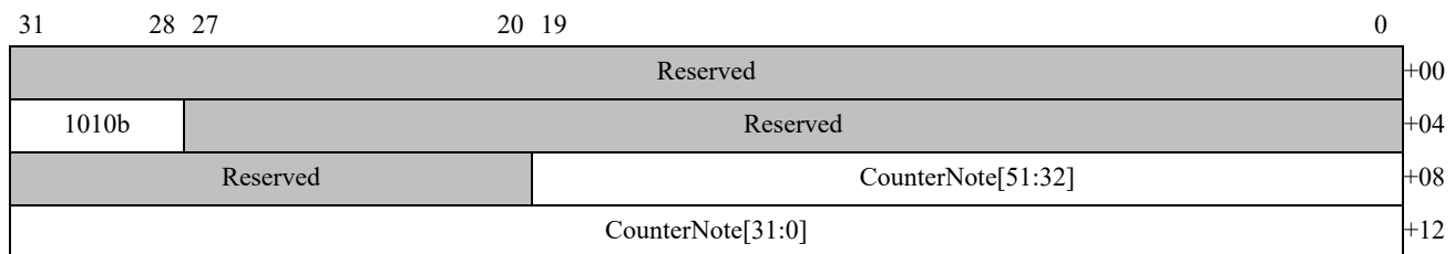
Figure 65: EVENT_COUNTER_ZERO Event Log Buffer Entry Format
