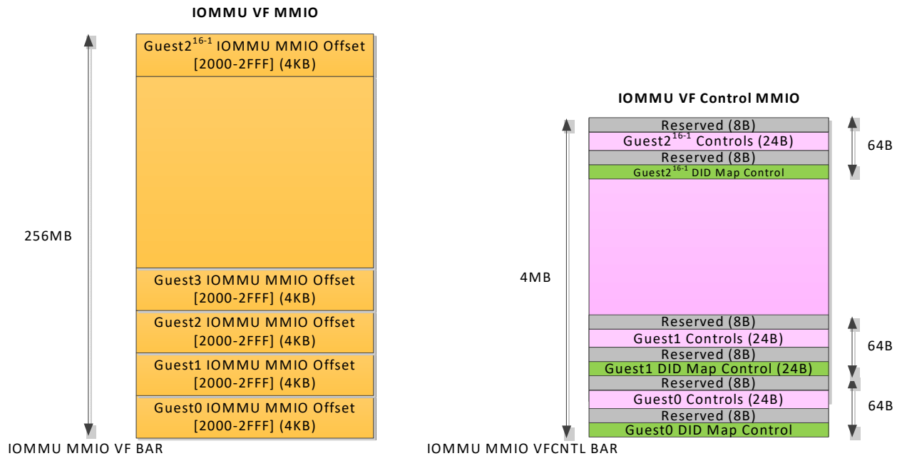
Figure 80: IOMMU Virtual Function Control MMIO and IOMMU Virtual Function MMIO
