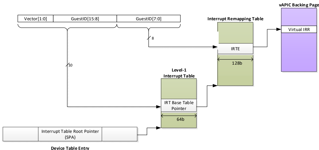
Figure 81: Extended Interrupt Remapping Table
