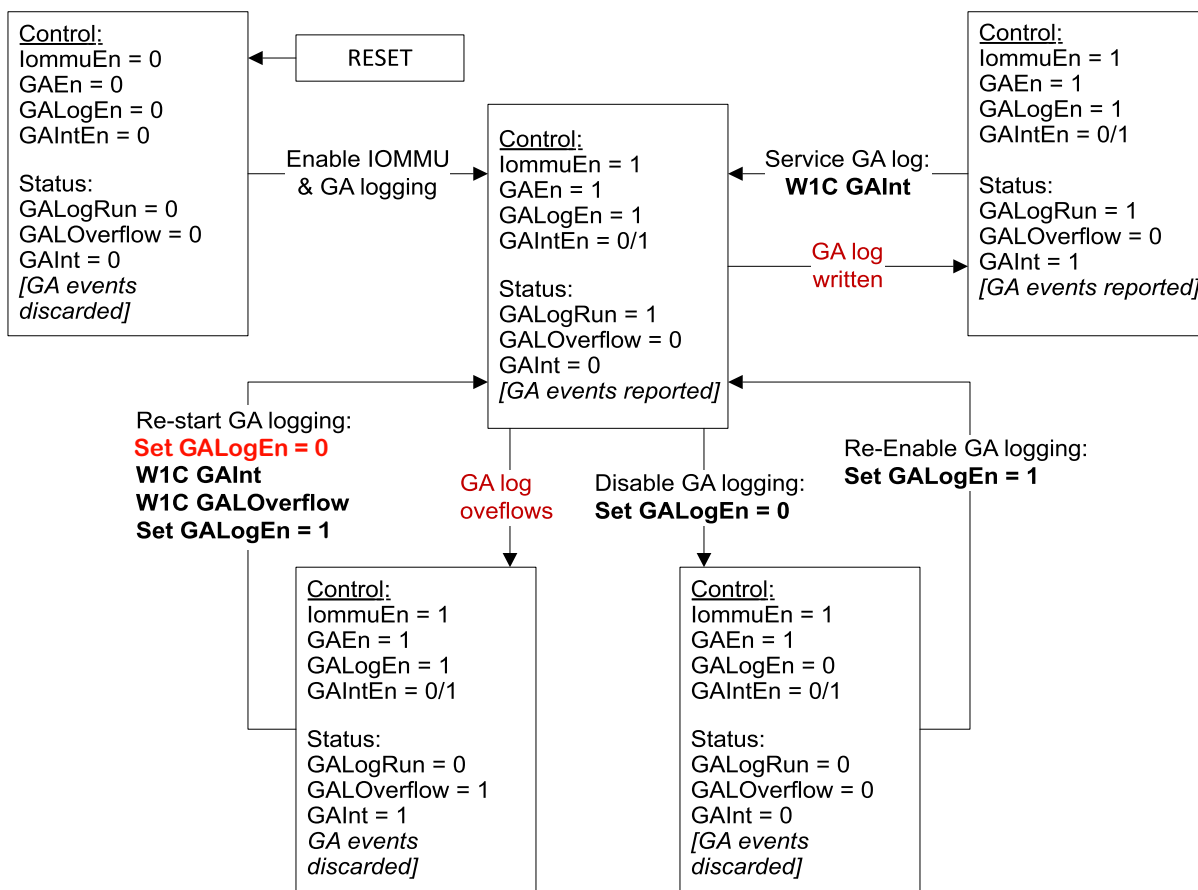
Figure 76: Guest Virtual APIC Log State Diagram
