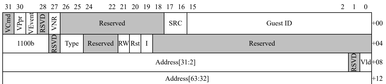
Figure 67: VIOMMU_HARDWARE_ERROR Event Entry Format
