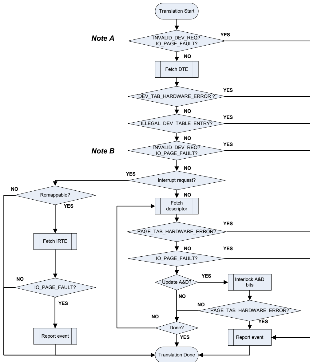
Figure 70: Translation and Remapping Validation Sequence
