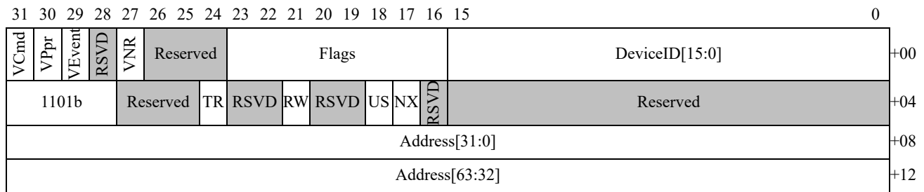
Figure 68: RMP_PAGE_FAULT Event Log Buffer Entry Format
