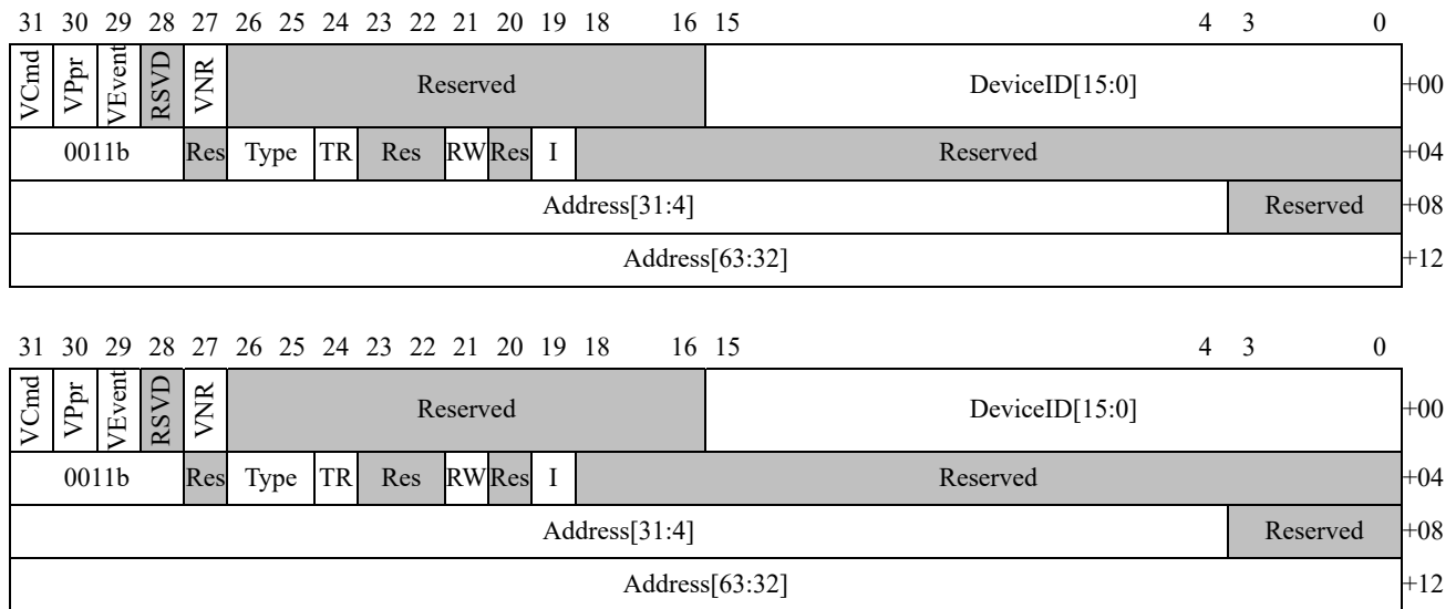
Figure 57: DEV_TAB_HARDWARE_ERROR Event Log Buffer Entry Format
