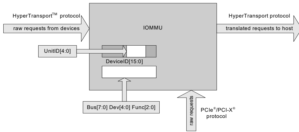
Figure 85: Hybrid IOMMU
