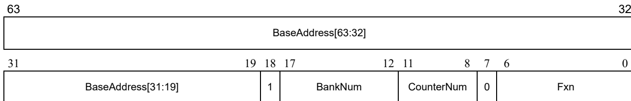
Figure 82: IOMMU Counter Register Address Decode
