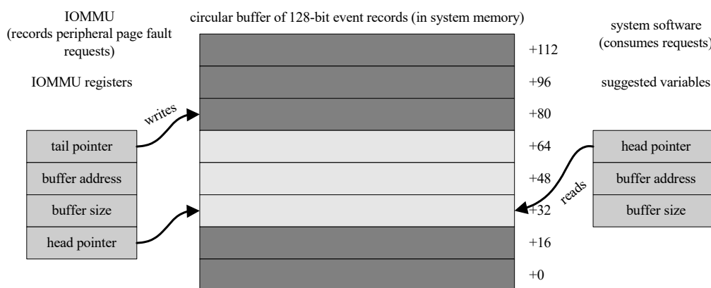
Figure 71: Peripheral Page Request Log in System Memory
