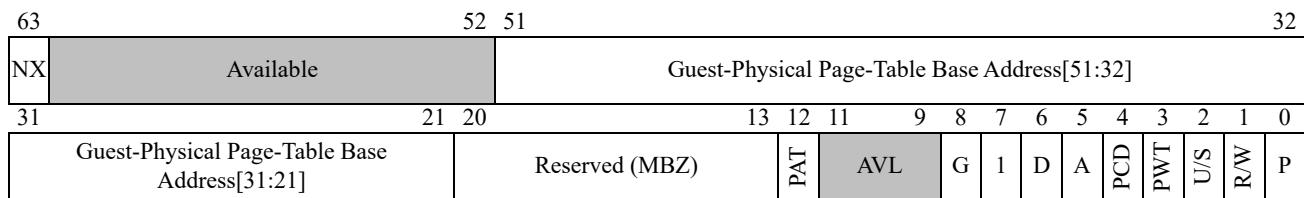
Figure 35: AMD64 Long Mode 2-Mbyte PDE Format
