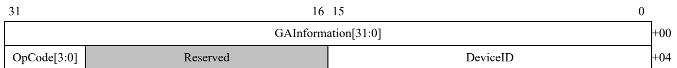
Figure 77: Generic Guest Virtual APIC Log Buffer Entry Format
