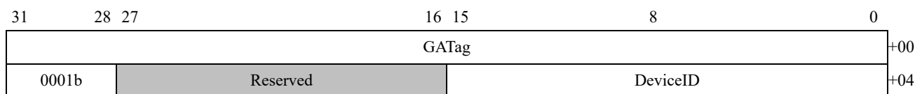
Figure 78: GA_GUEST_NR Log Buffer Entry Format
