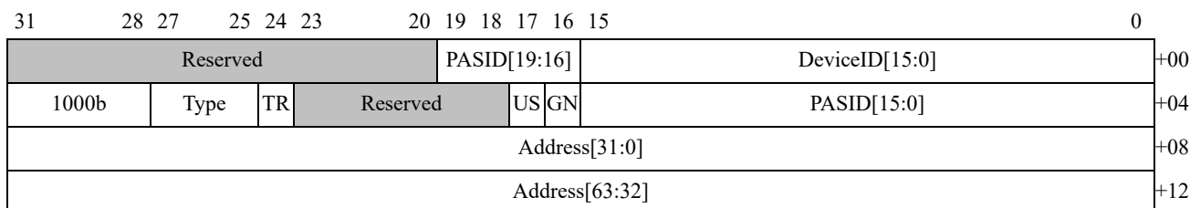
Figure 62: INVALID_DEVICE_REQUEST Event Log Buffer Entry Format
