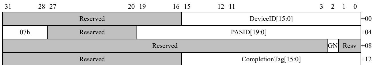
Figure 50: COMPLETE_PPR_REQUEST Command Format
