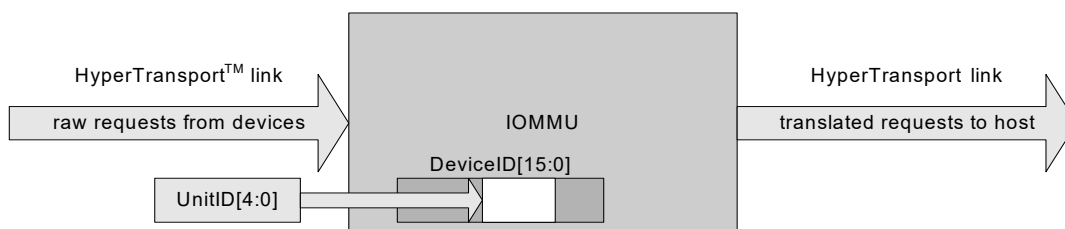
Figure 83: IOMMU in a Tunnel
