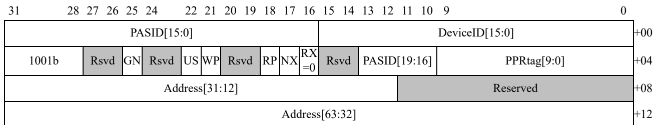
Figure 63: INVALID_PPR_REQUEST Event Log Buffer Entry Format, RX = 0
