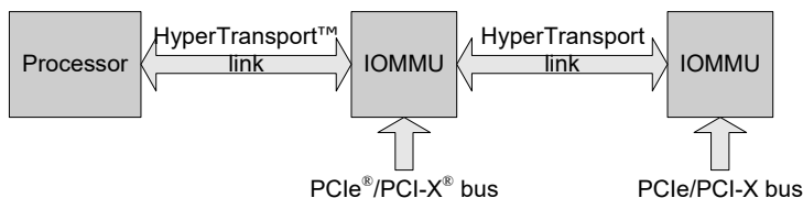
Figure 86: Chained Hybrid IOMMU in a Large System
