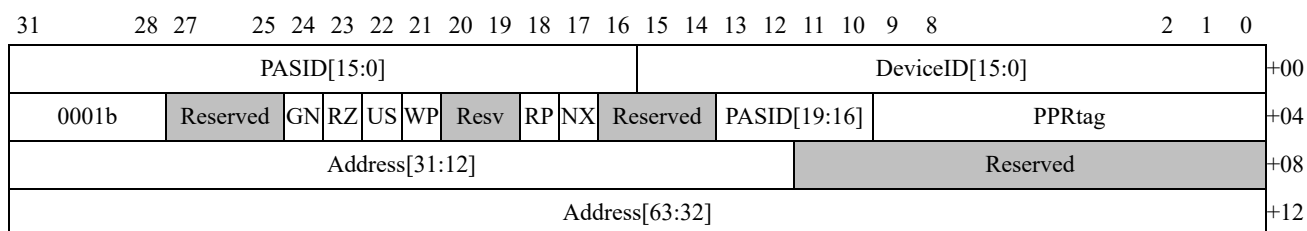
Figure 74: PAGE_SERVICE_REQUEST PPR Log Buffer Entry Format
