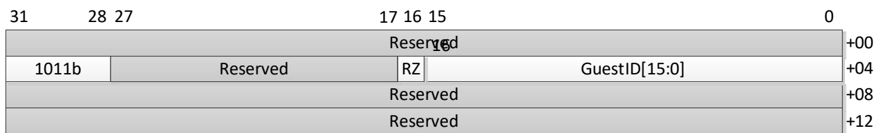
Figure 66: GUEST_EVENT_FAULT Event Buffer Entry Format
