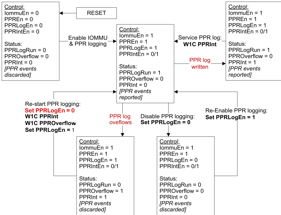
Figure 72: PPR Log State Diagram
