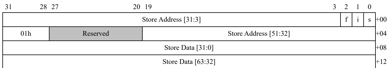
Figure 44: COMPLETION_WAIT Command Format
