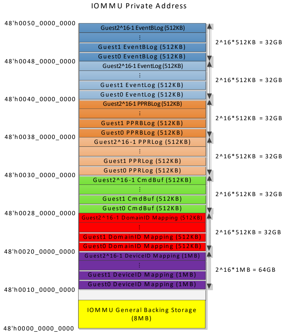
Figure 79: IOMMU Private Address Map
