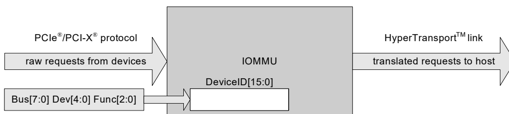
Figure 84: IOMMU in a Peripheral Bus Bridge
