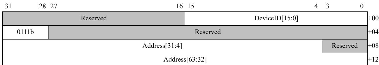
Figure 61: IOTLB_INV_TIMEOUT Event Log Buffer Entry Format
