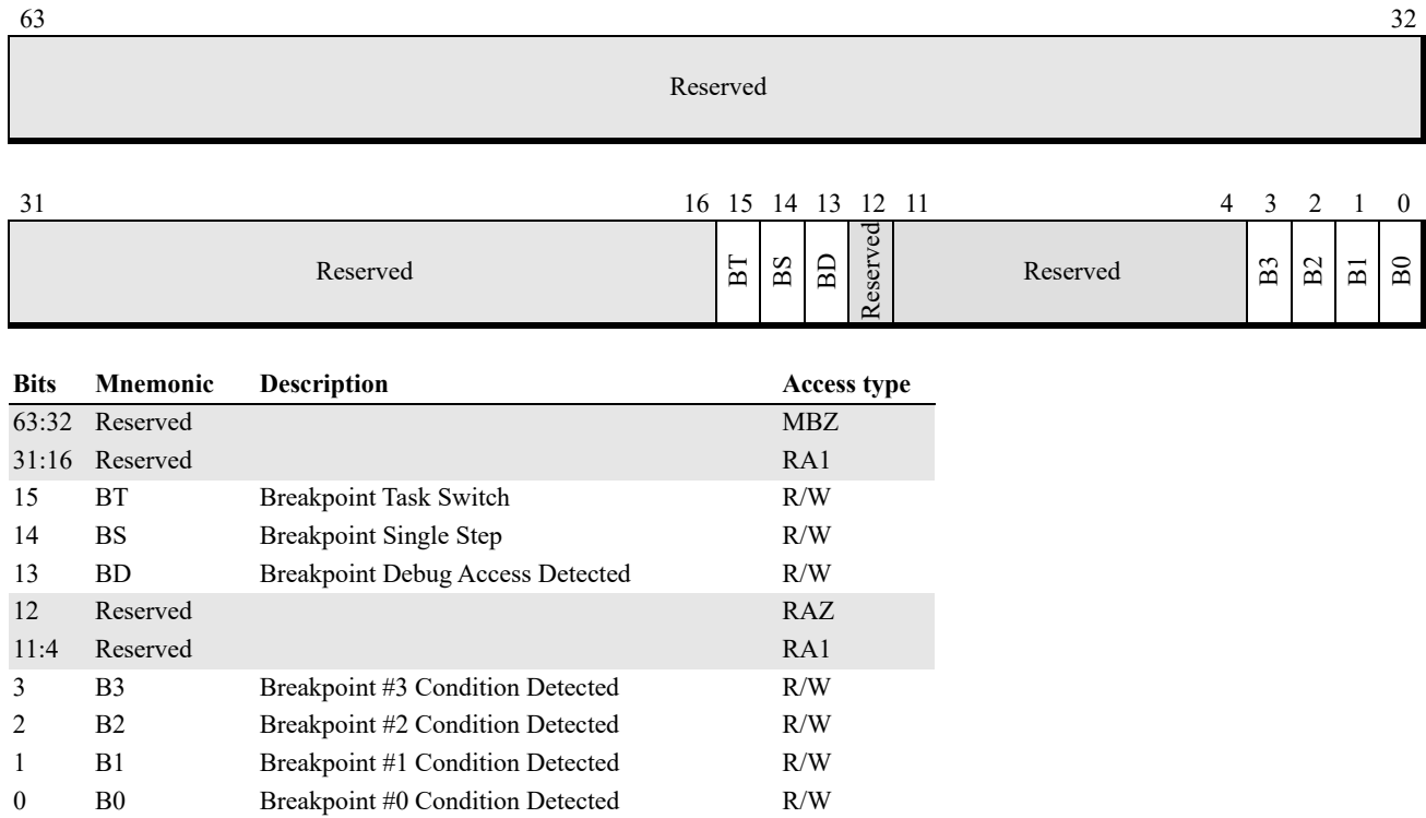
Figure 13-2. Debug-Status Register (DR6)
