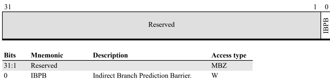
Figure 3-14. PRED_CMD Register (MSR 049h)
