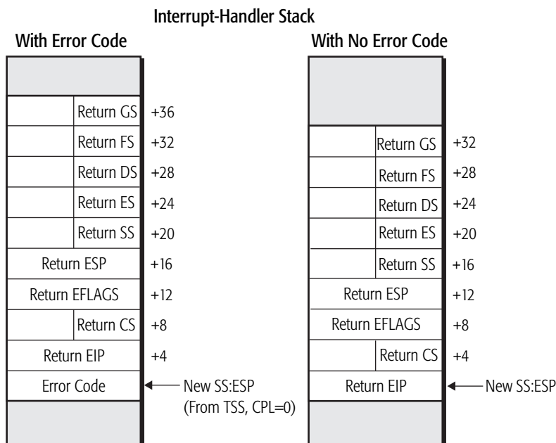
Figure 8-12. Stack After Virtual-8086 Mode Interrupt to Protected Mode
