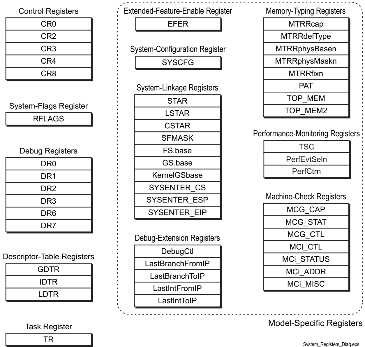
Figure 1-7. System Registers
