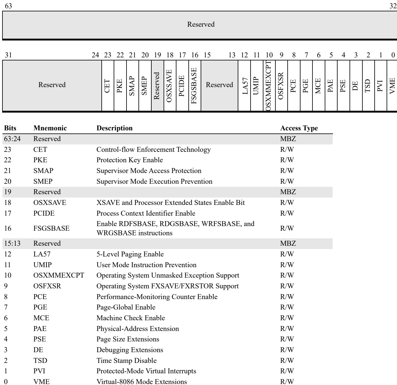
Figure 3-7. CR4 Register
