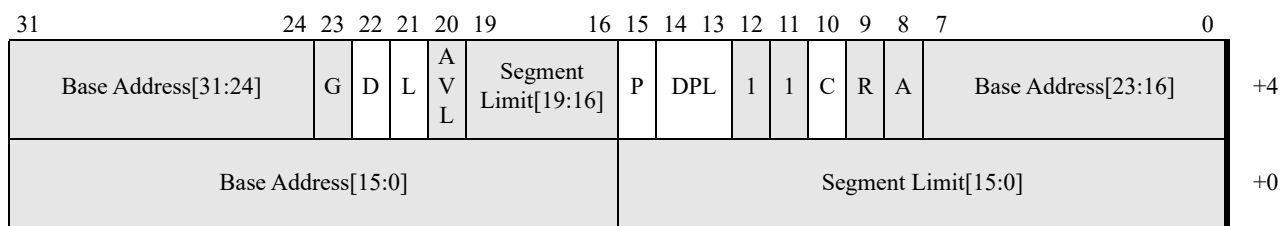
Figure 4-20. Code-Segment Descriptor—Long Mode
