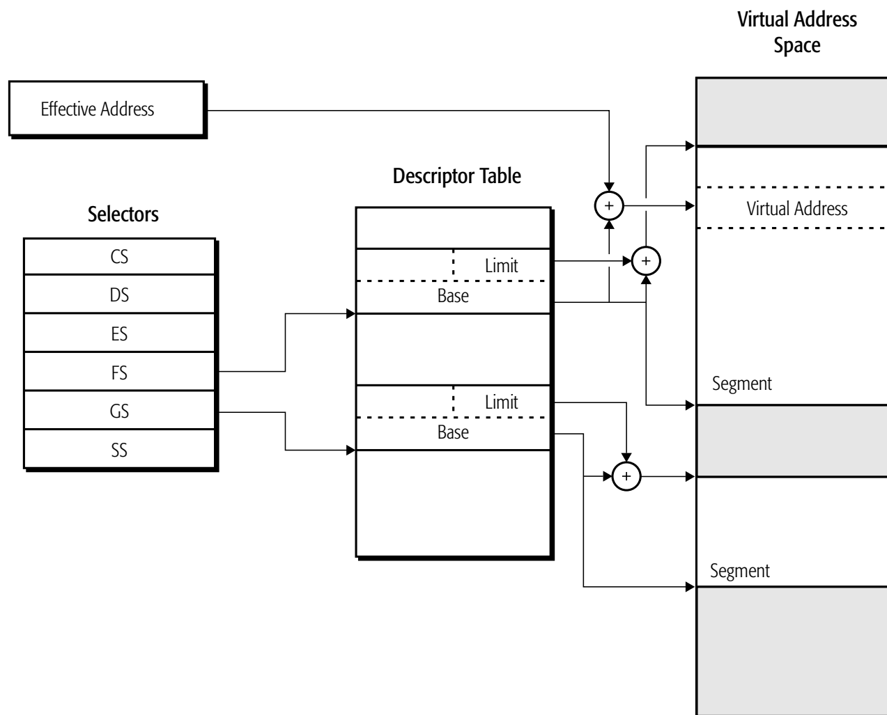
Figure 1-1. Segmented-Memory Model
