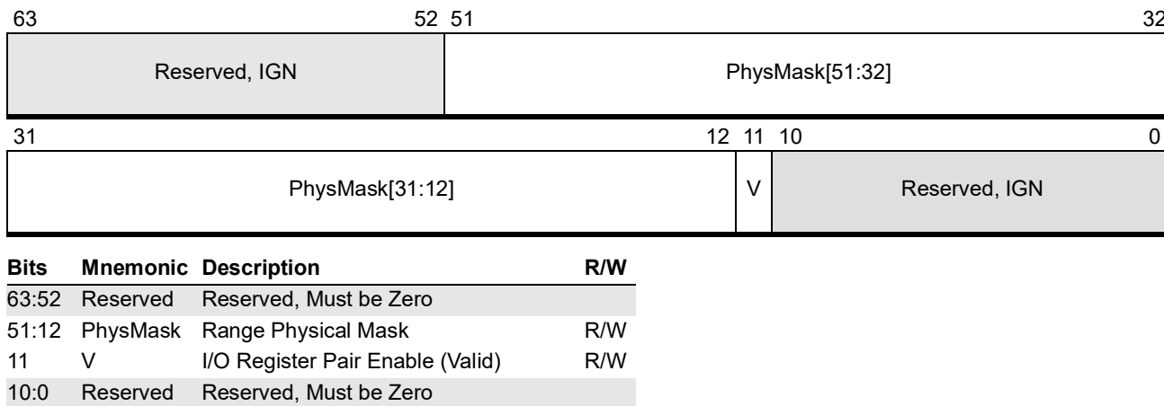
Figure 7-13. IORRMaskn Register
