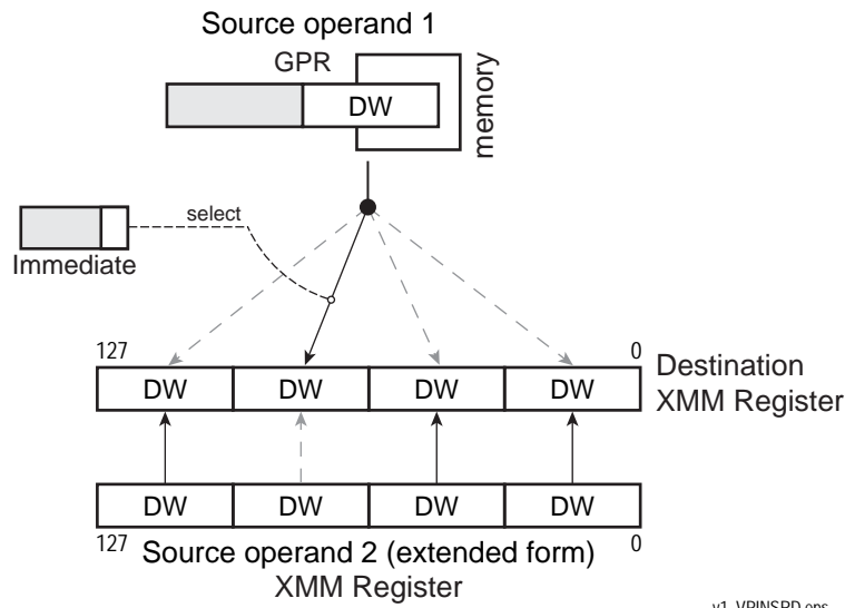
Figure 4-28. (V)PINSRD Operation
