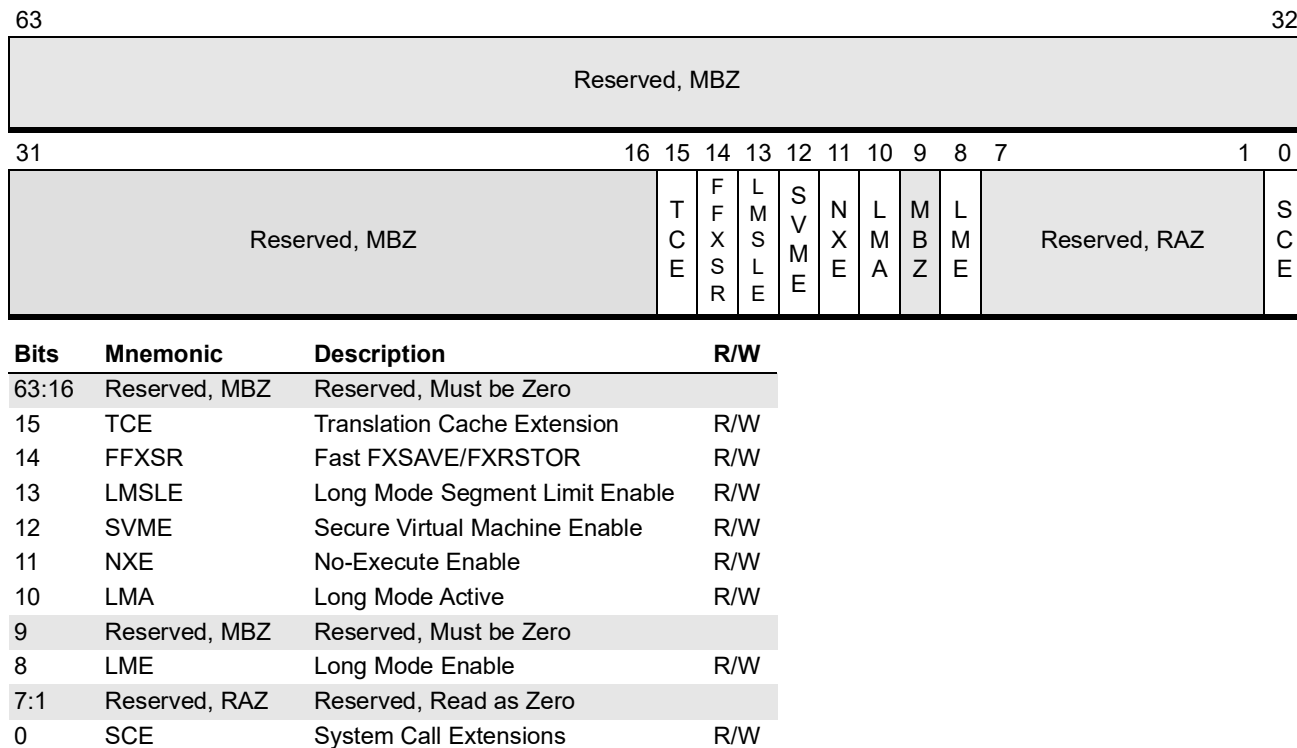
Figure 3-8. Extended Feature Enable Register (EFER)
