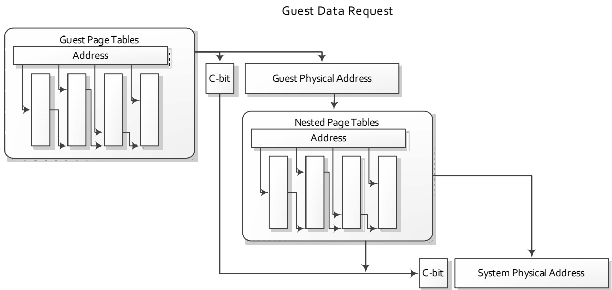
Figure 15-28. Guest Data Request
