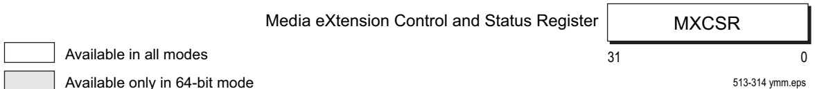
Figure 2-8. SSE Registers
