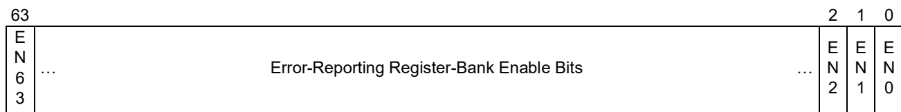
Figure 9-3. MCG_CTL Register
