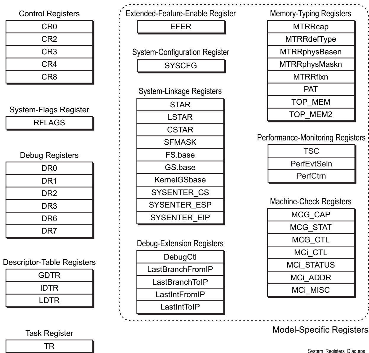
Figure 2-6. System Registers
