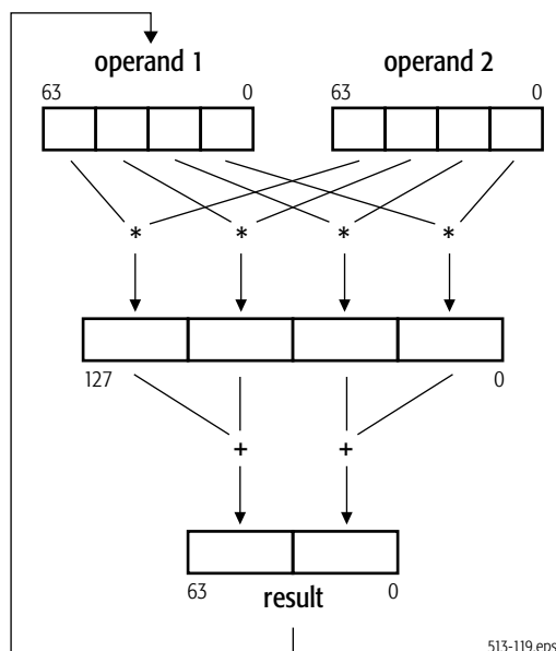
Figure 5-4. Multiply-Add Operation
