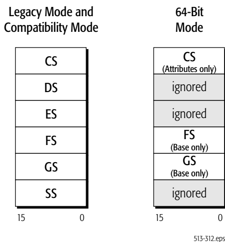
Figure 2-4. Segment Registers
