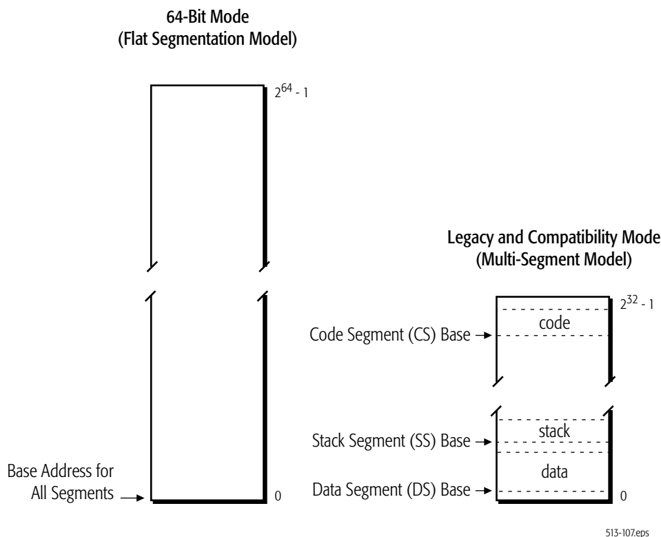
Figure 2-1. Virtual-Memory Segmentation
