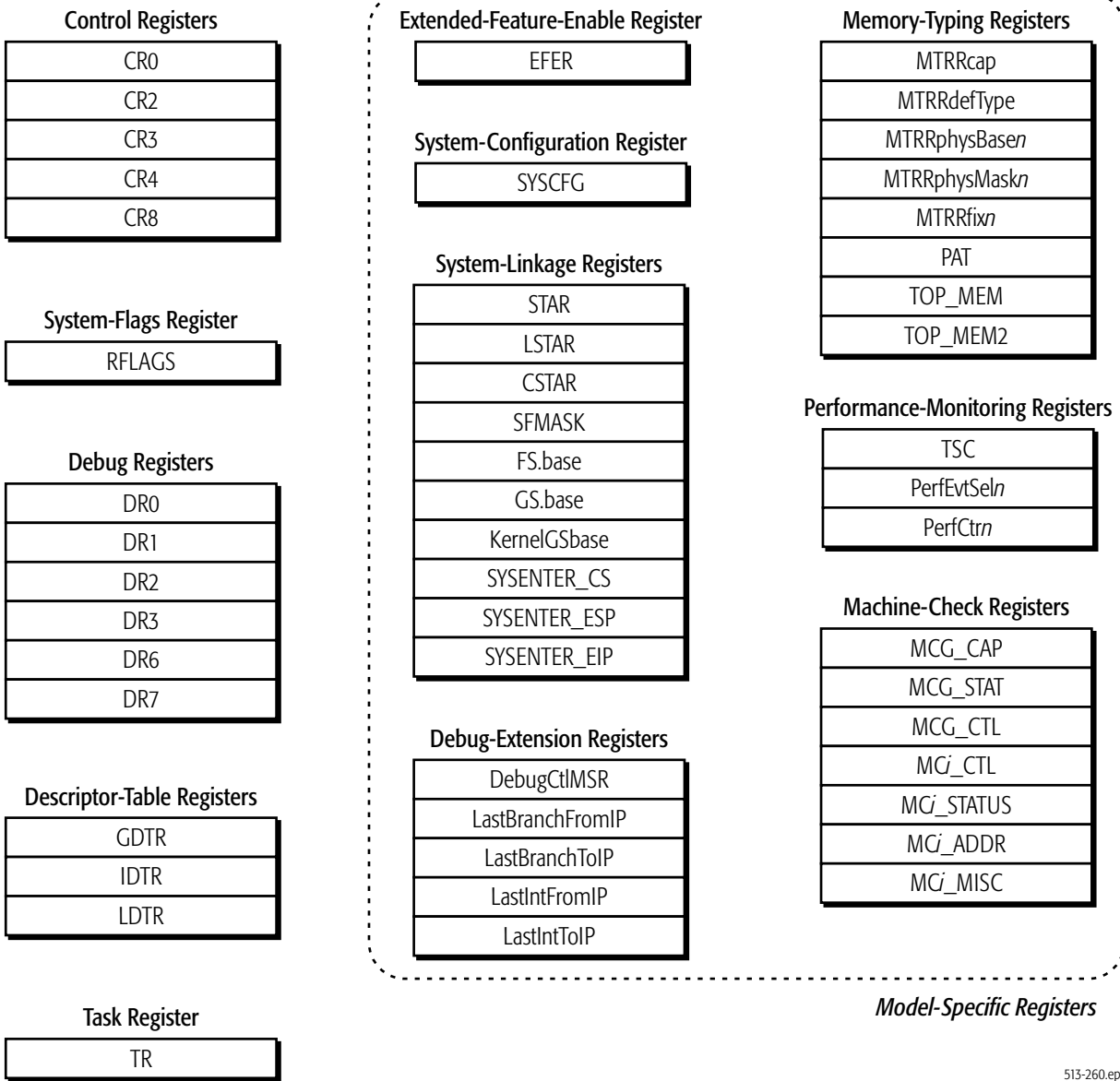
Figure 2-6. System Registers
