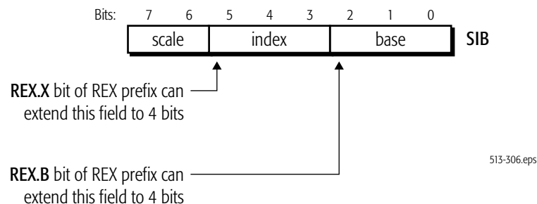
Figure 1-5. SIB-Byte Format
