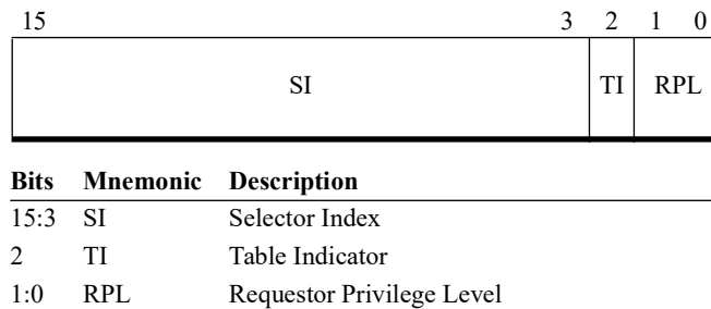
Figure 4-3. Segment Selector
