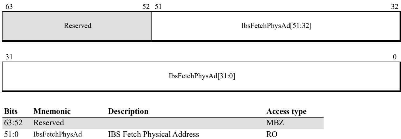
Figure 13-21. IBS Fetch Physical Address Register (IbsFetchPhysAd)
