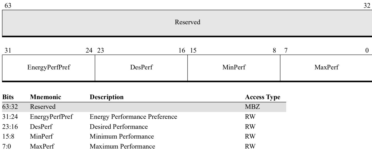
Figure 17-12. CPPC_REQUEST
