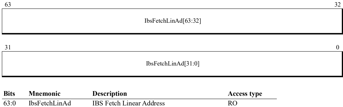
Figure 13-20. IBS Fetch Linear Address Register (IbsFetchLinAd)
