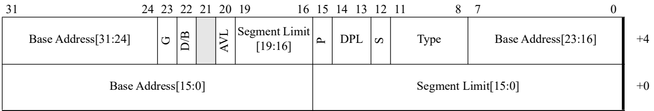
Figure 4-13. Generic Segment Descriptor—Legacy Mode
