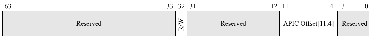
Figure 15-25. EXITINFO1
