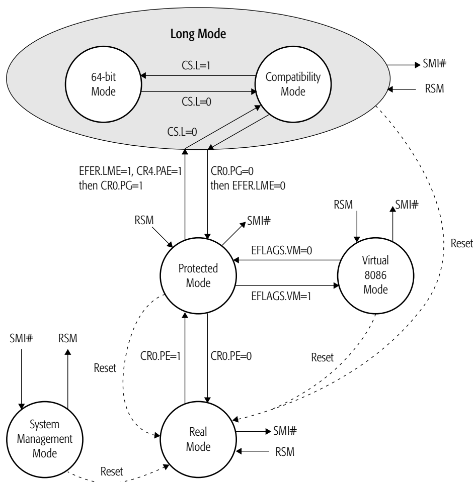
Figure 1-6. Operating Modes of the AMD64 Architecture
