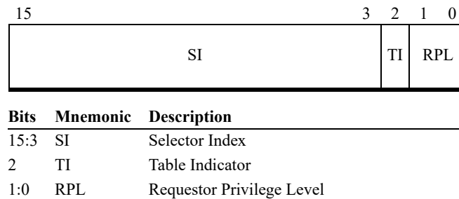
Figure 4-3. Segment Selector
