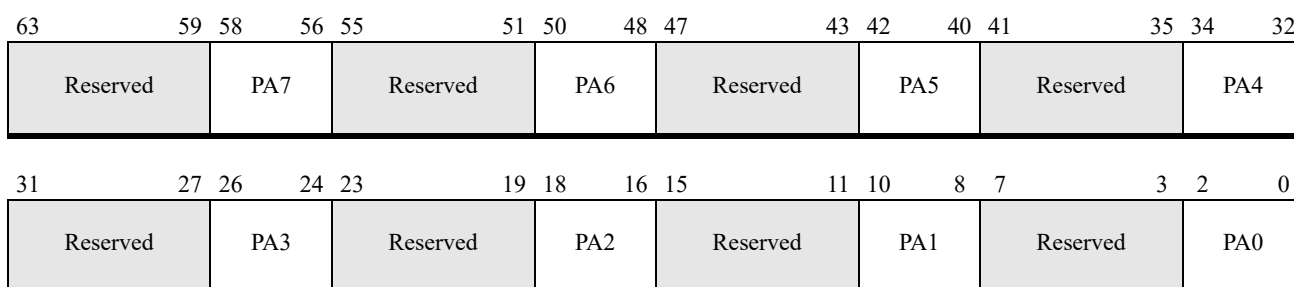
Figure 7-13. PAT Register
