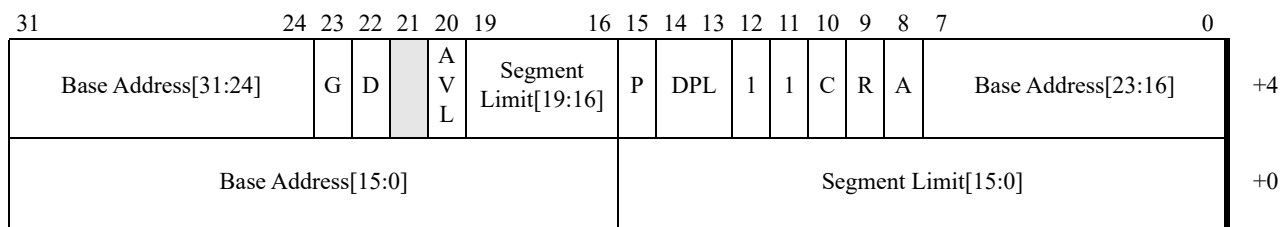
Figure 4-14. Code-Segment Descriptor—Legacy Mode
