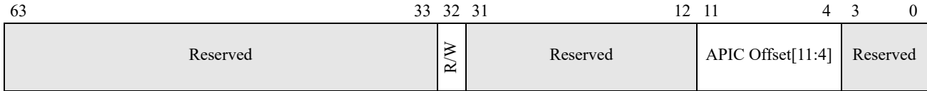
Figure 15-25. EXITINFO1
