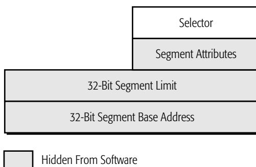
Figure 4-4. Segment-Register Format
