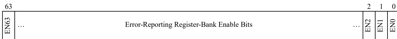
Figure 9-3. MCG_CTL Register
