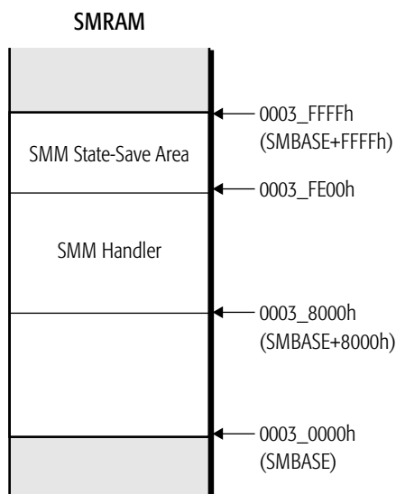
Figure 10-1. Default SMRAM Memory Map
