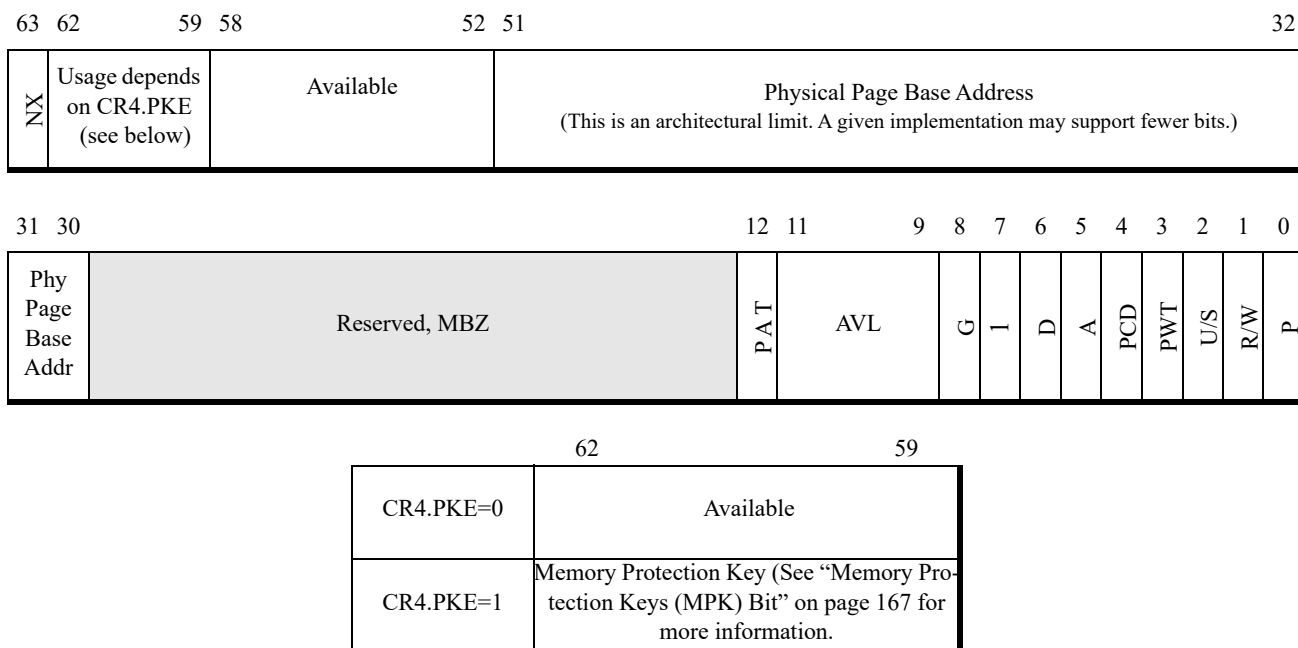
Figure 5-34. 1-Gbyte PDPE—Long Mode
