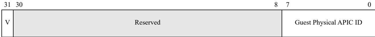
Figure 15-19. Logical APIC ID Table Entry
