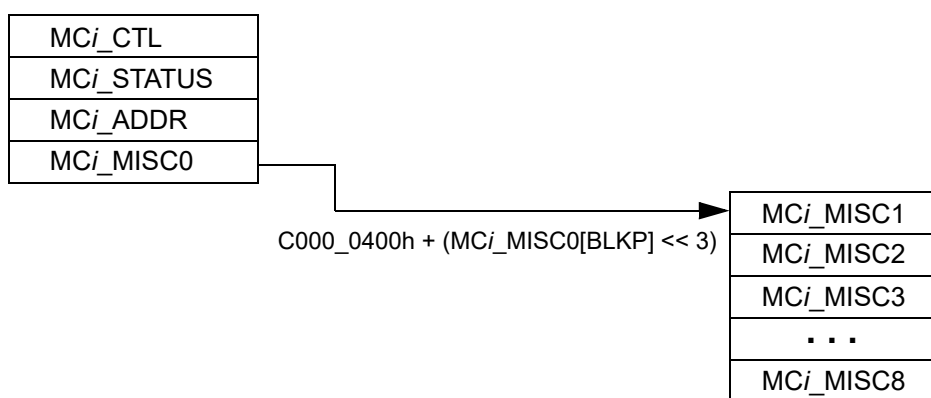
Figure 9-8. MC_i\_MISC1 Addressing
