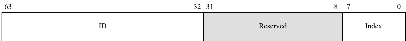
Figure 15-24. EXITINFO2
