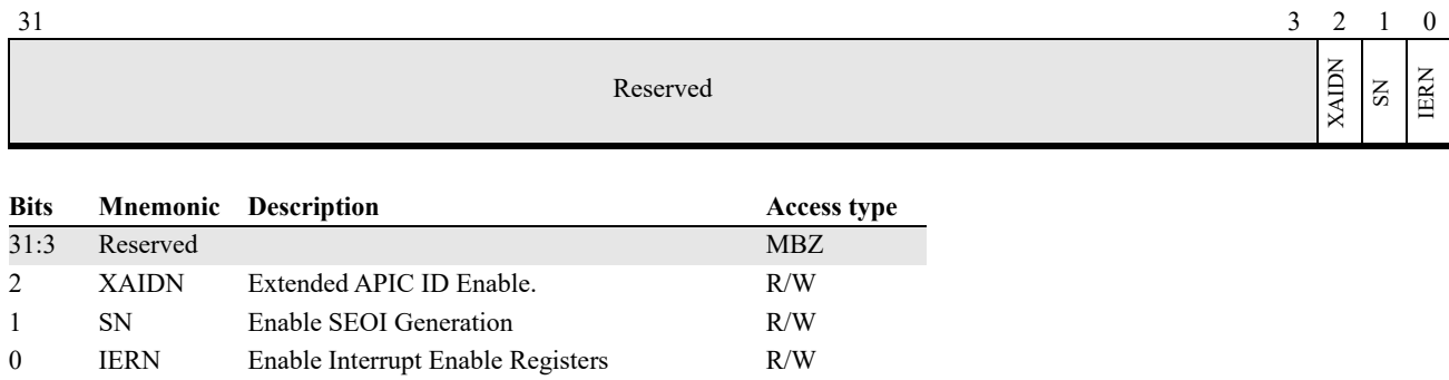
Figure 16-6. Extended APIC Control Register (APIC Offset 410h)
