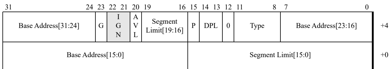
Figure 4-16. LDT and TSS Descriptor—Legacy/Compatibility Modes
