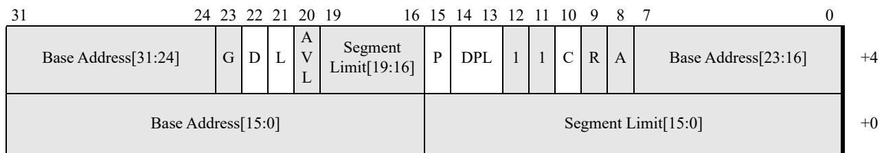
Figure 4-20. Code-Segment Descriptor—Long Mode
