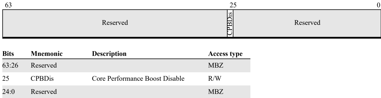
Figure 17-4. Core Performance Boost (MSR C001_0015h)
