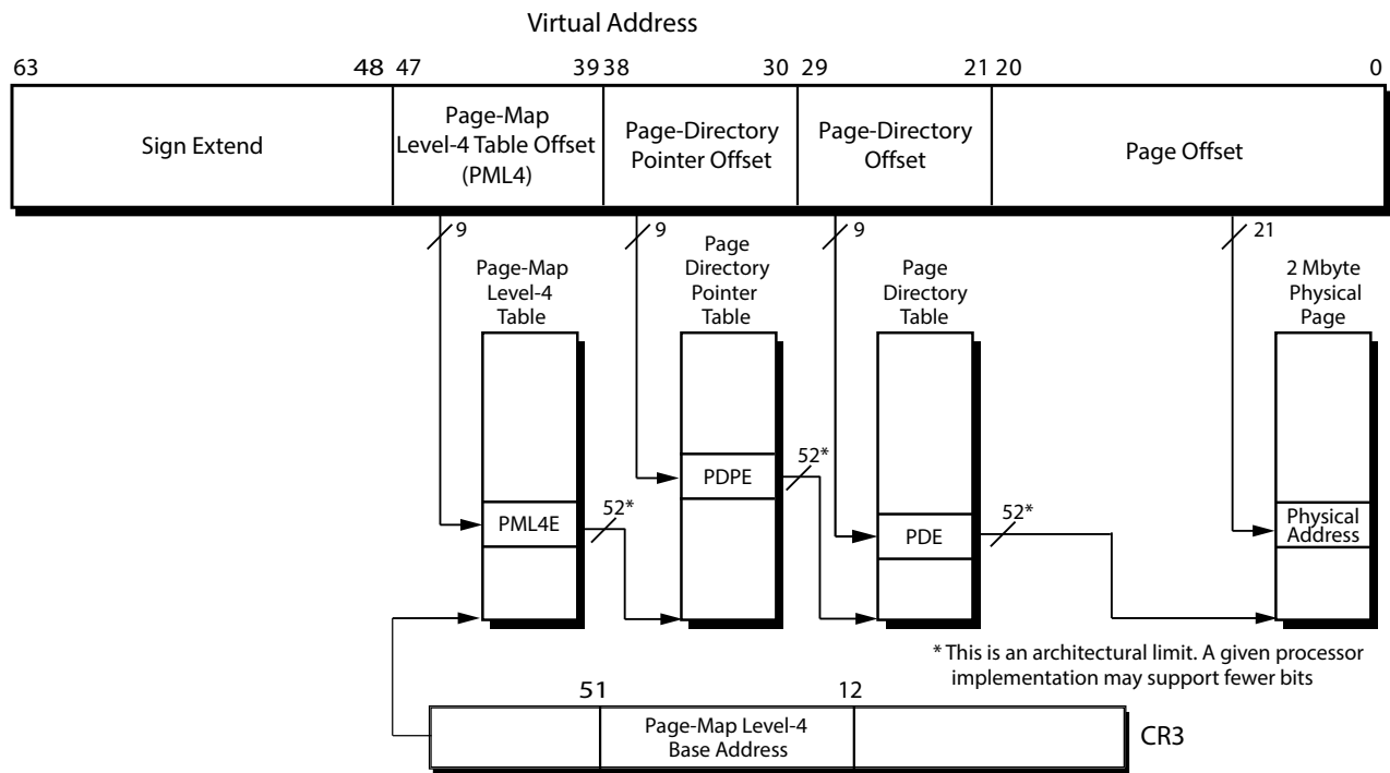
Figure 5-24. 2-Mbyte Page Translation—Long Mode 4-Level Paging
