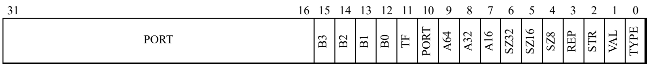
Figure 10-6. I/O Instruction Restart Dword
