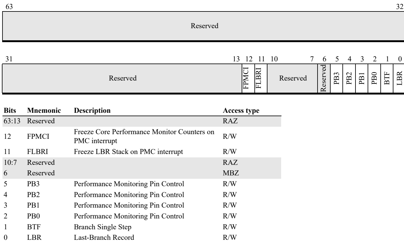
Figure 13-4. Debug-Control MSR (DebugCtl)
