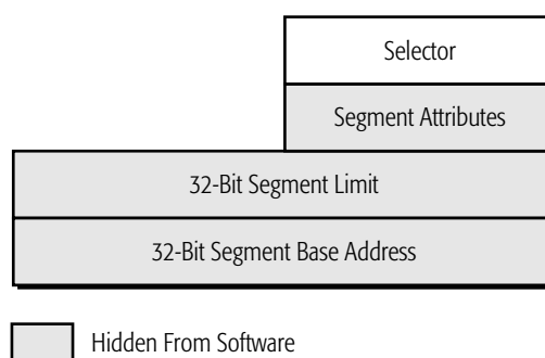
Figure 4-4. Segment-Register Format
