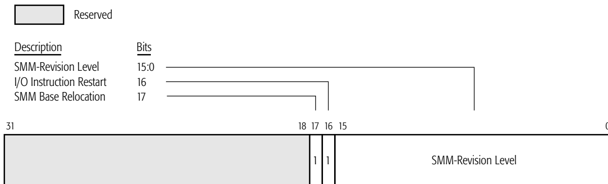
Figure 10-3. SMM-Revision Identifier
