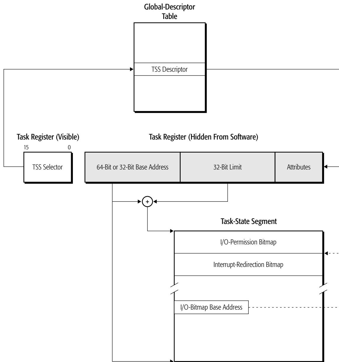
Figure 12-1. Task-Management Resources
