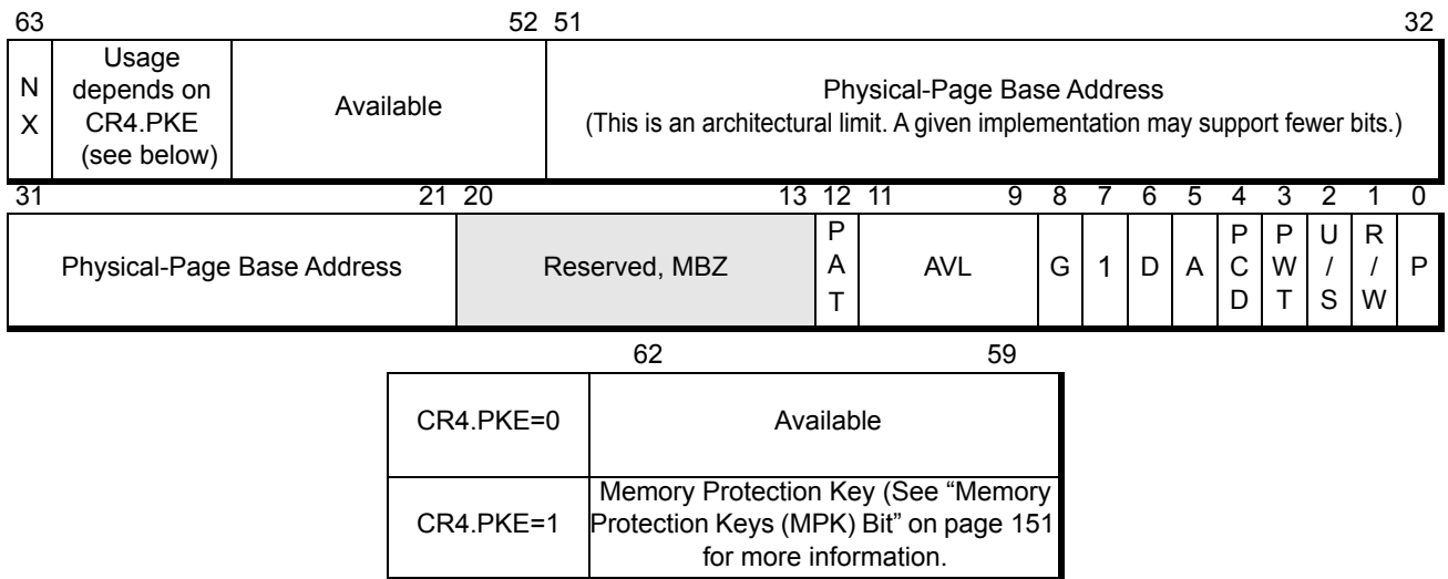
Figure 5-25. 2-Mbyte PDE—Long Mode
