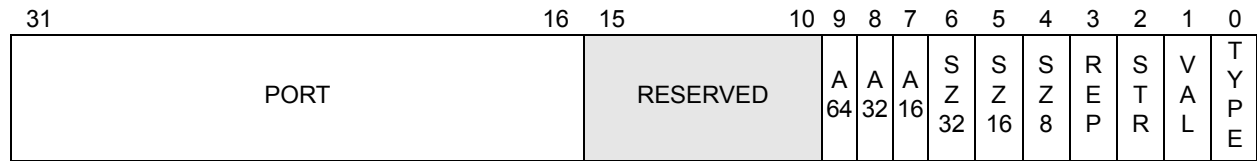
Figure 10-6. I/O Instruction Restart Dword
