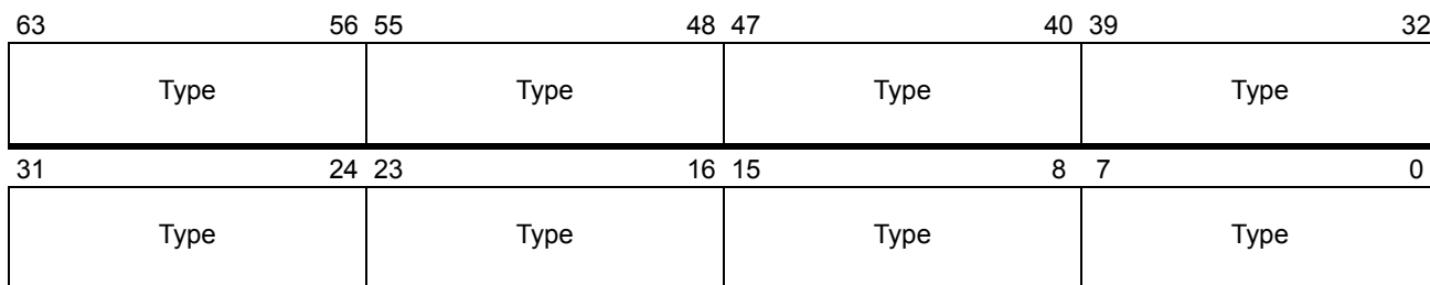
Figure 7-5. Fixed-Range MTRR
