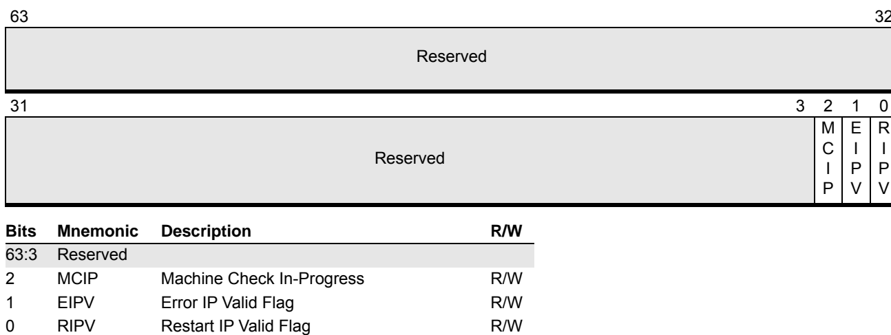
Figure 9-2. MCG_STATUS Register
