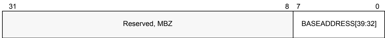
Figure 15-9. Format of DEV_BASE_HI[n] Registers
