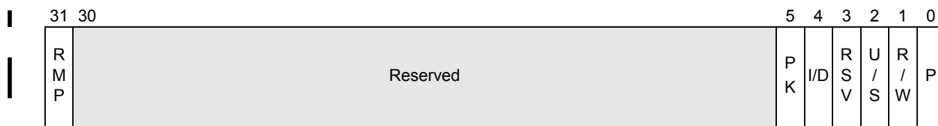
Figure 8-3. Page-Fault Error Code
