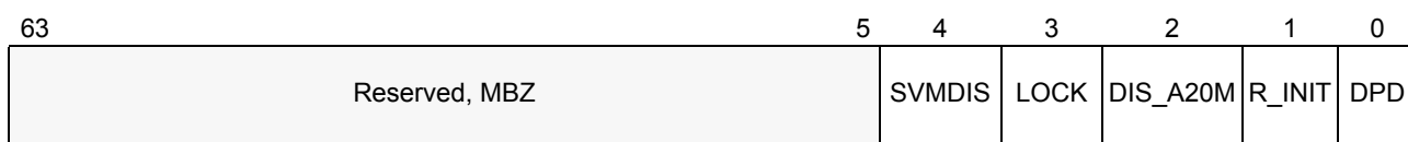
Figure 15-25. Layout of VM_CR MSR (C001_0114h)
