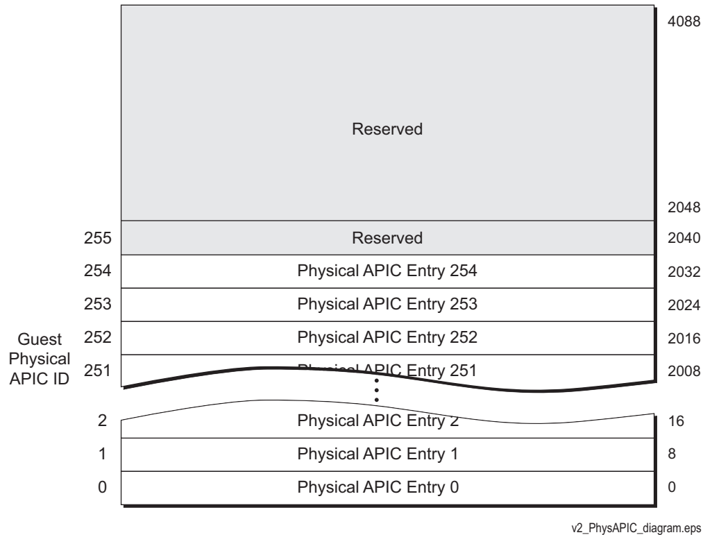
Figure 15-18. Physical APIC Table in Memory.
