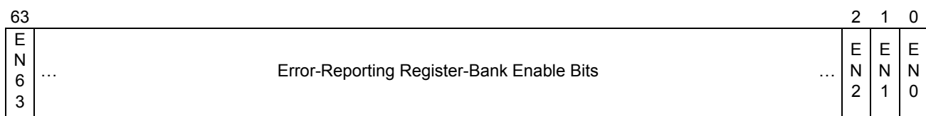
Figure 9-5. MCi_CTL Register
