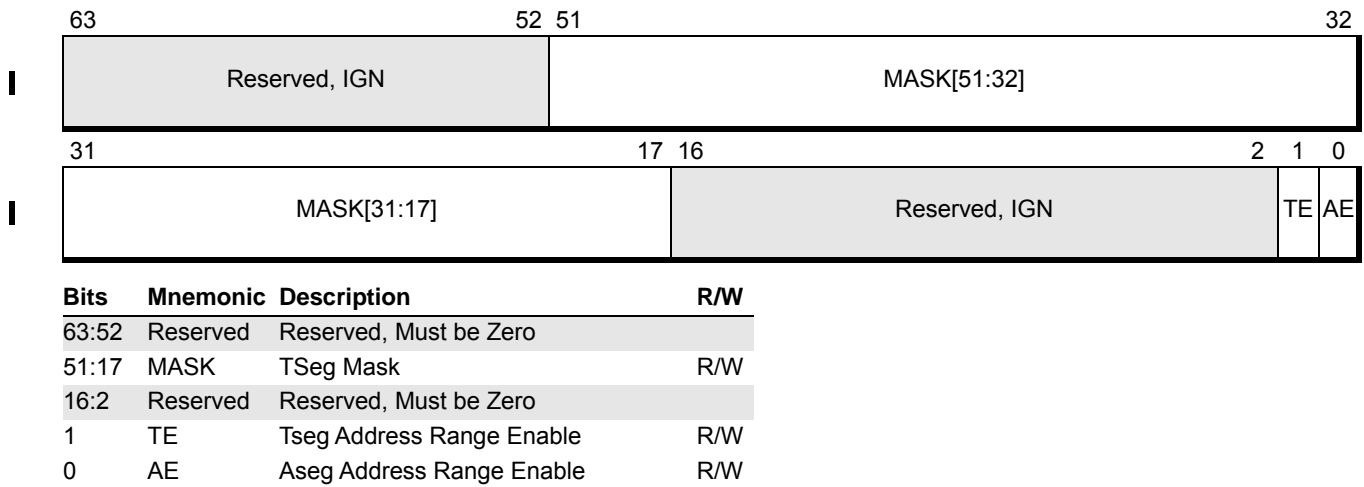
Figure 10-5. SMM_MASK Register Format
