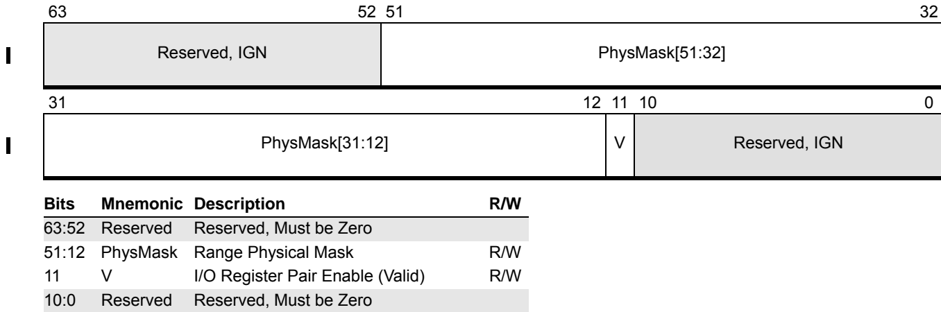
Figure 7-13. IORRMaskn Register
