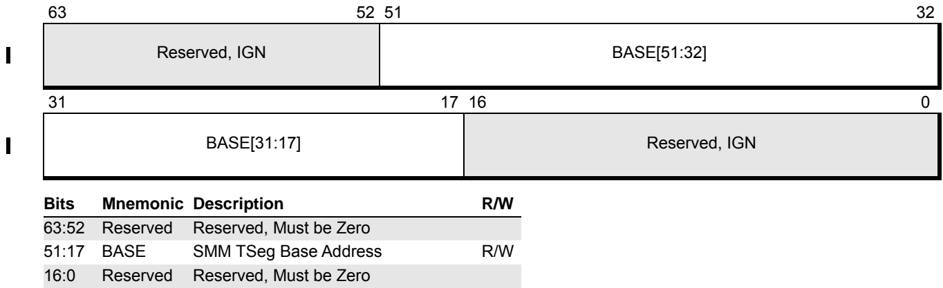
Figure 10-4. SMM_ADDR Register Format
