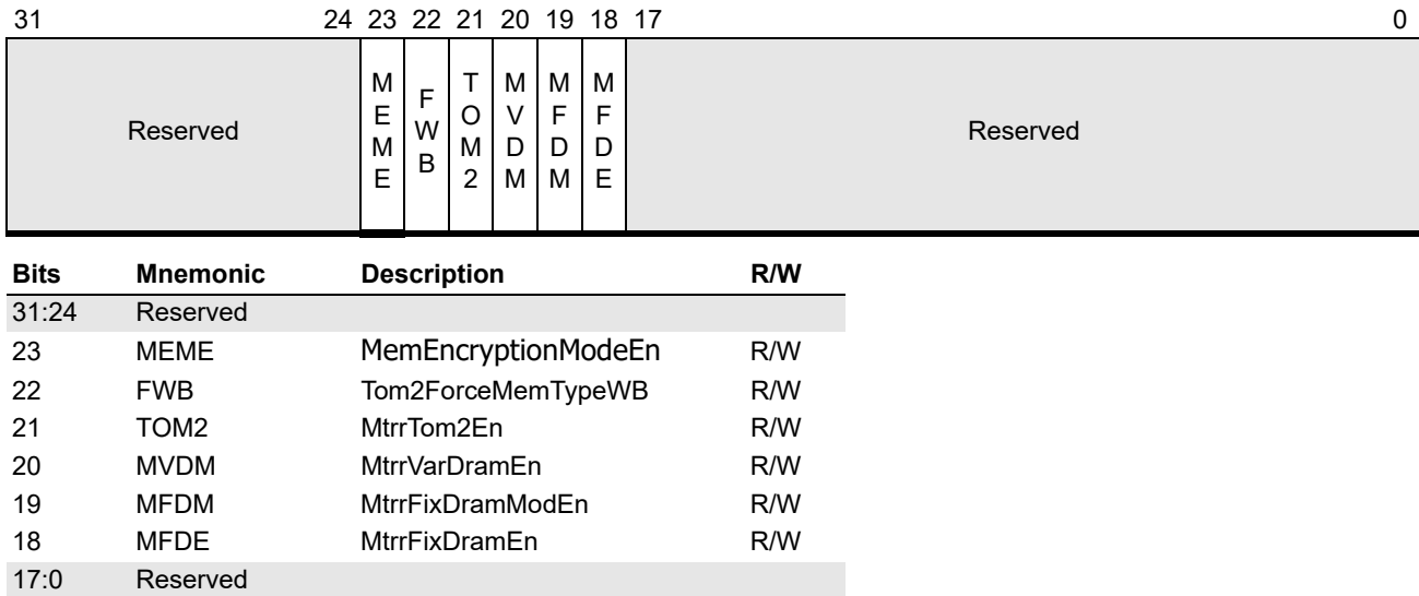
Figure 3-10. System-Configuration Register (SYSCFG)
