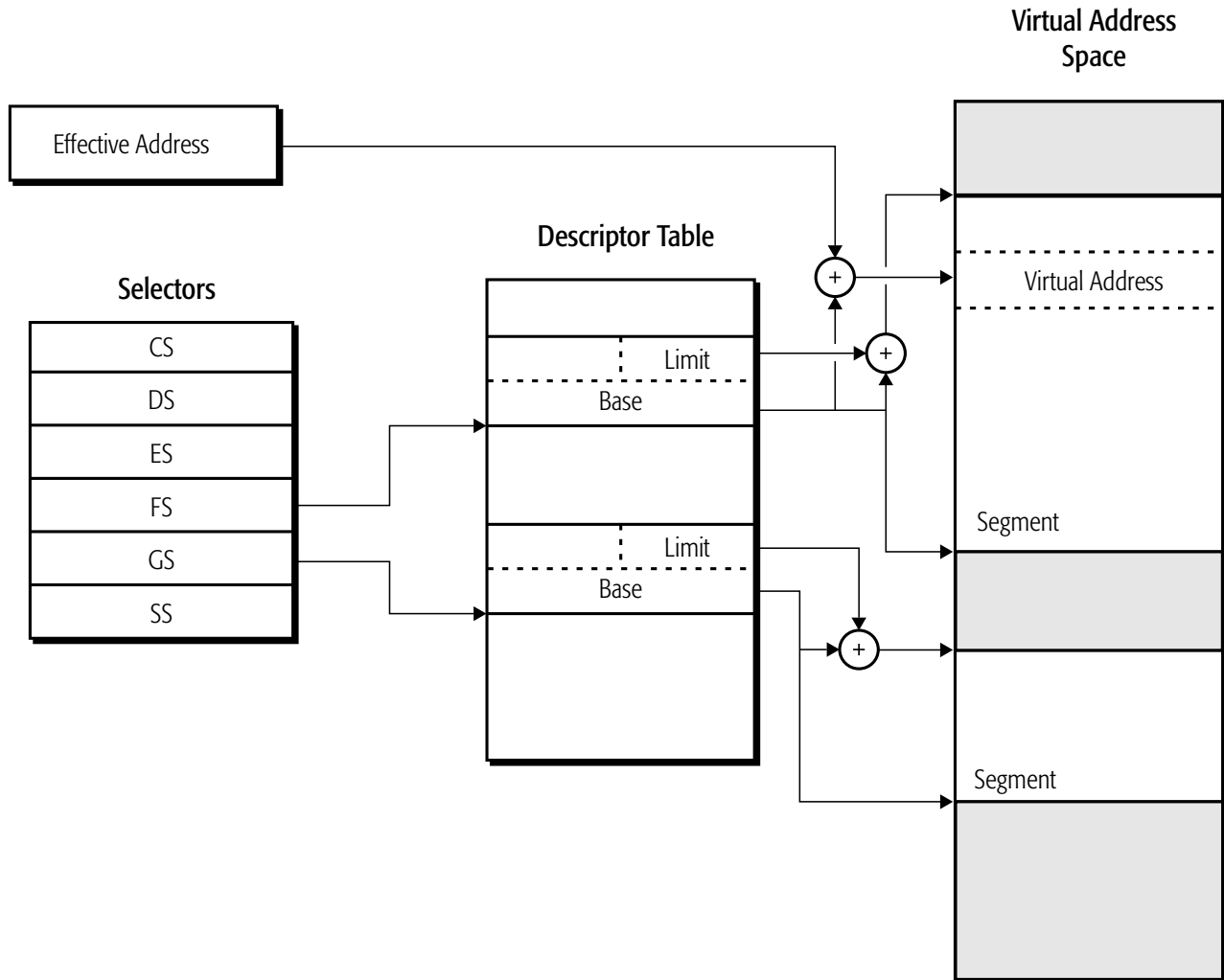
Figure 1-1. Segmented-Memory Model
