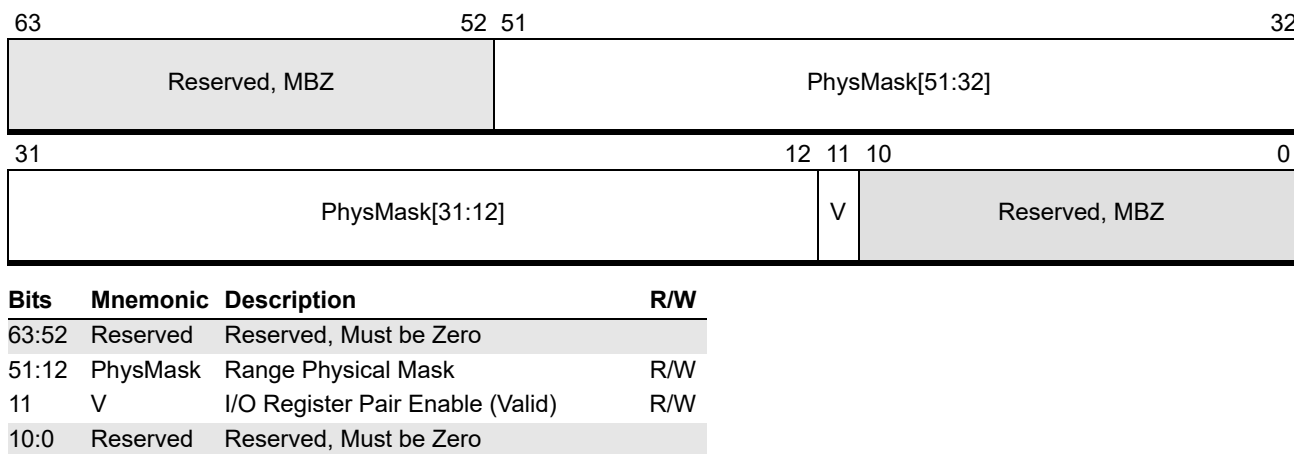
Figure 7-13. IORRMaskn Register
