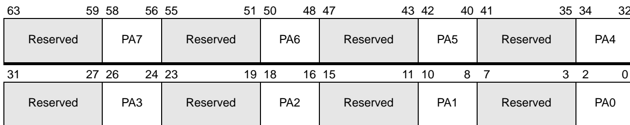
Figure 7-10. PAT Register
