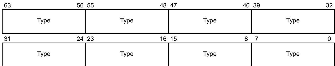
Figure 7-5. Fixed-Range MTRR
