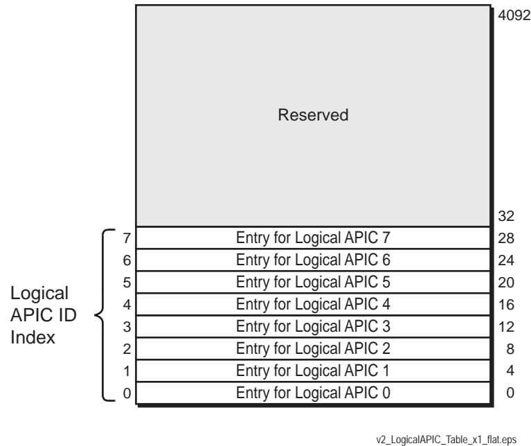
Figure 15-20. Logical APIC ID Table Format, Flat Mode.
