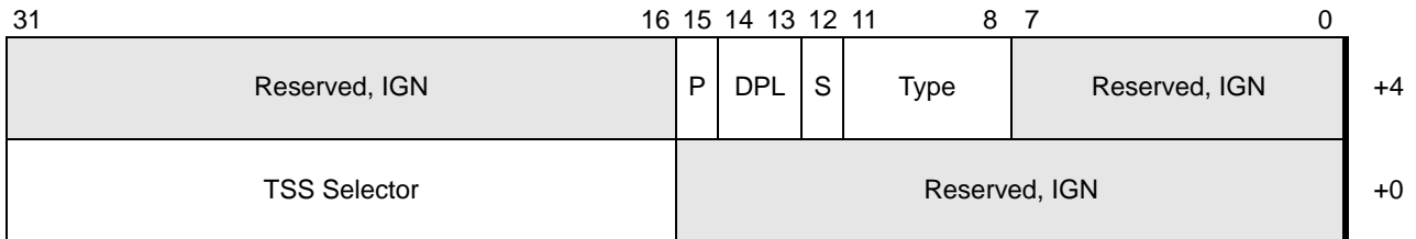
Figure 12-9. Task-Gate Descriptor, Legacy Mode Only
