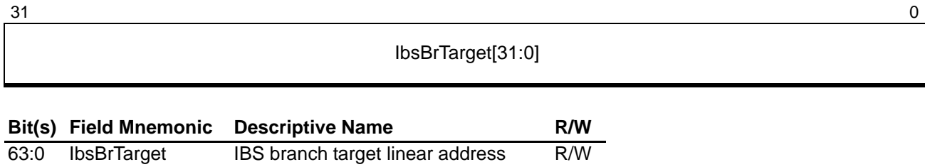
Figure 13-20. IBS Branch Target Address Register (lbsBrTarget)
