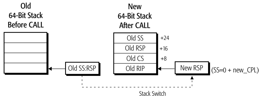
Figure 4-35. Stack Switch—Long Mode
