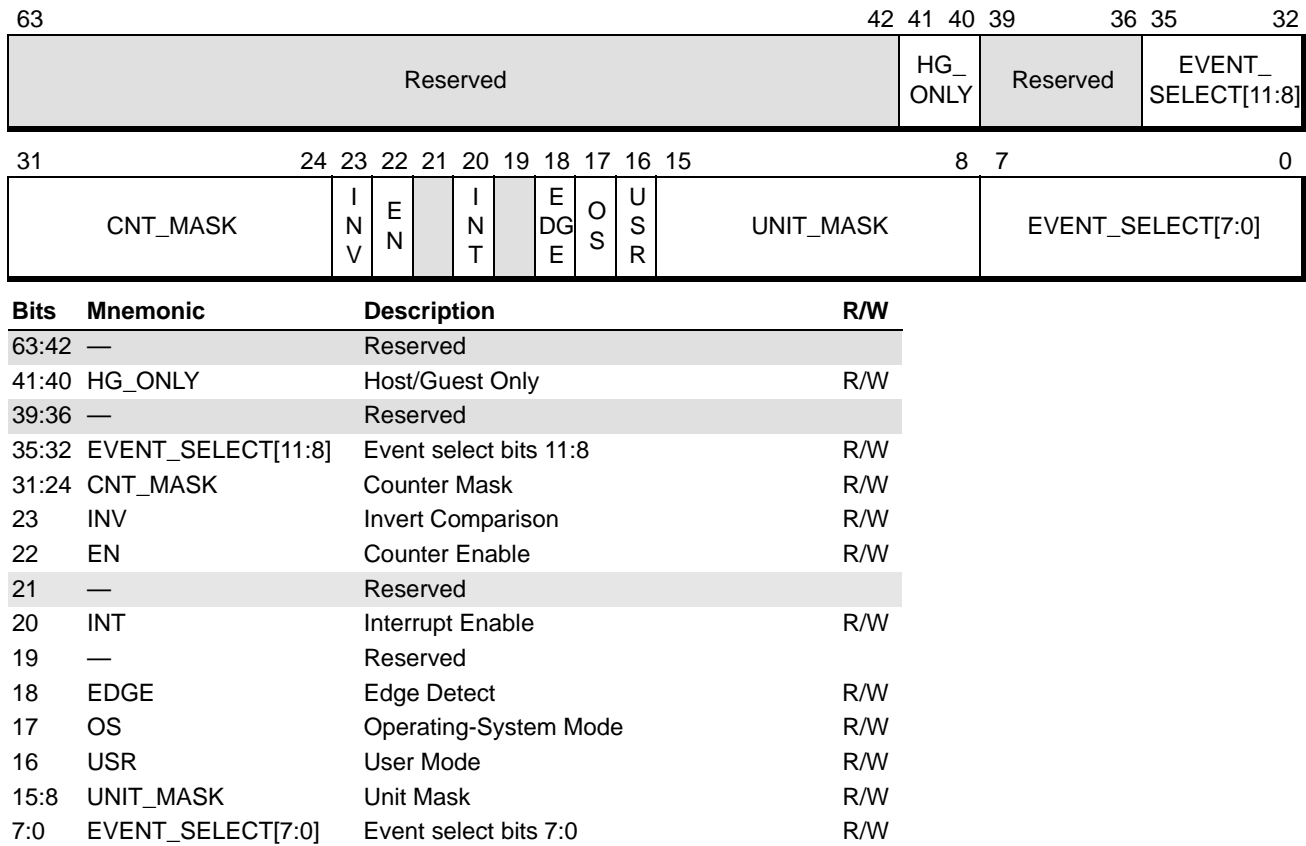
Figure 13-7. Core Performance Event-Select Register (PerfEvtSeln)
