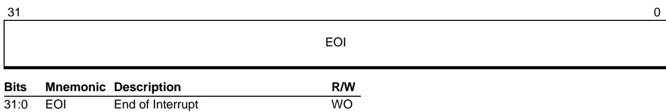
Figure 16-28. End of Interrupt (APIC Offset B0h)
