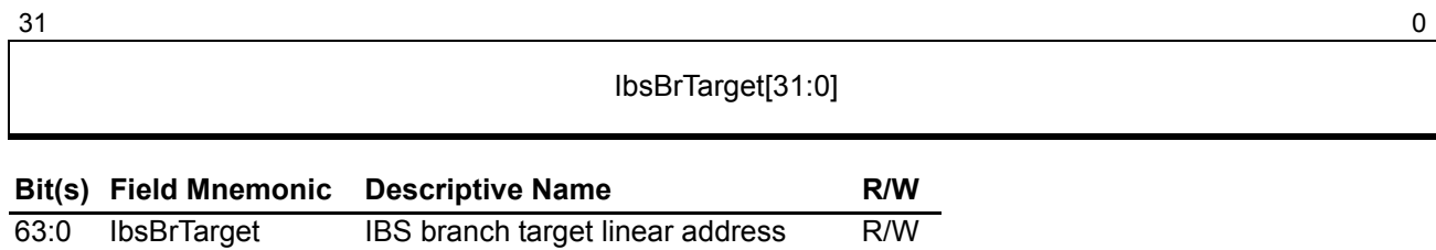
Figure 13-19. IBS Branch Target Address Register (IbsBrTarget)
