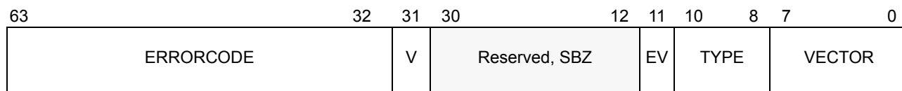
Figure 15-5. EVENTINJ Field in the VMCB
