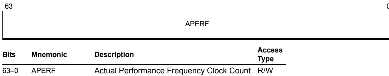
Figure 18-5. Actual Performance Frequency Count (MSR0000_00E8h)
