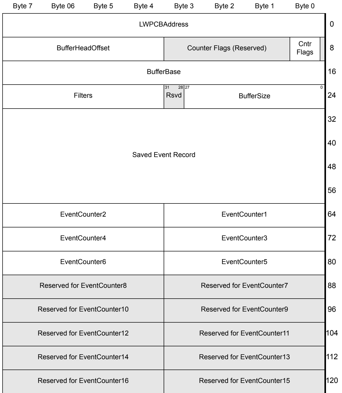
Figure 13-22. XSAVE Area for LWP
