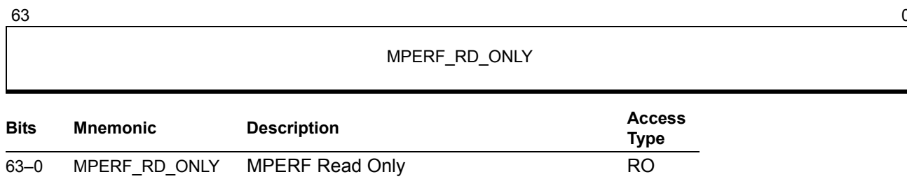
Figure 18-7. MPERF Read Only (MSR C000_00E7h)
