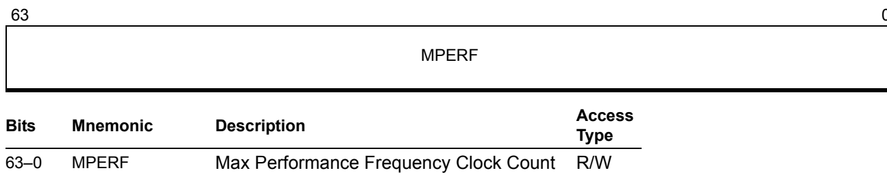
Figure 18-6. Max Performance Frequency Count (MSR0000_00E7h)
