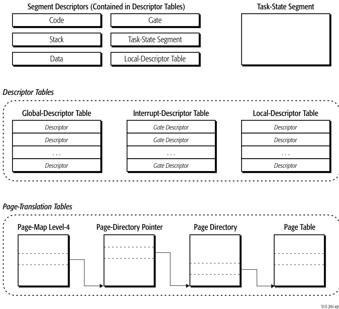
Figure 1-8. System-Data Structures
