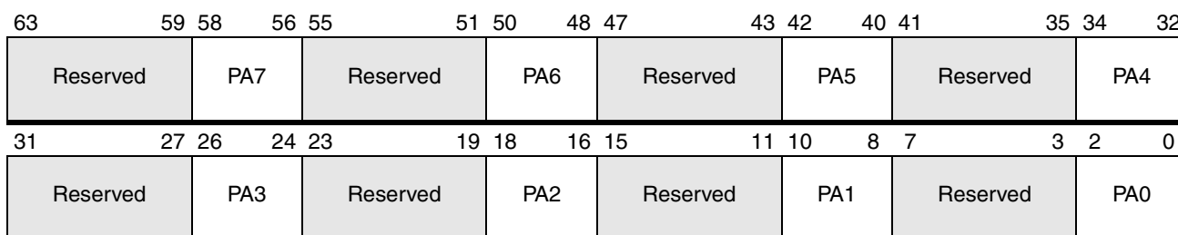
Figure 7-10. PAT Register
