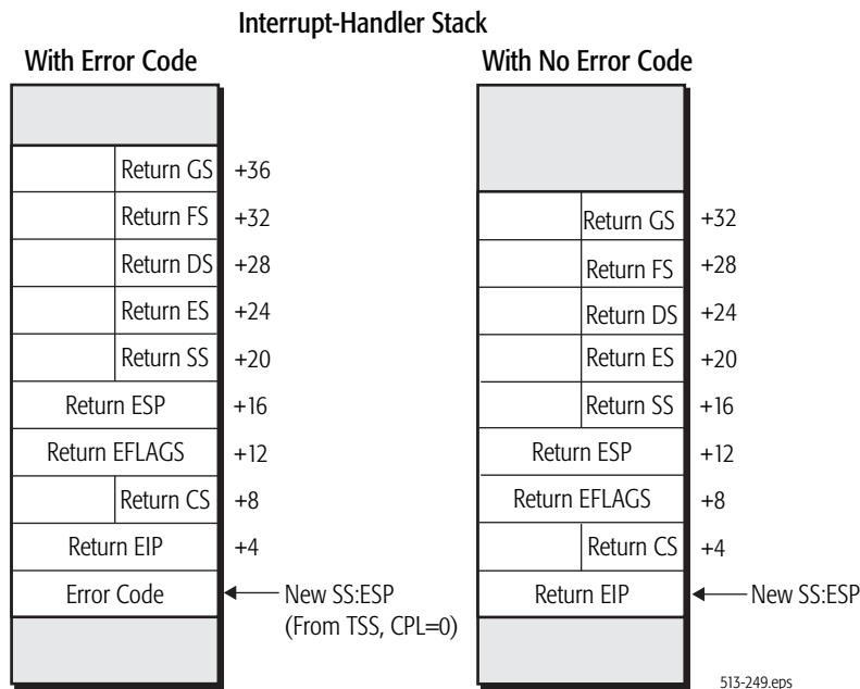
Figure 8-11. Stack After Virtual-8086 Mode Interrupt to Protected Mode
